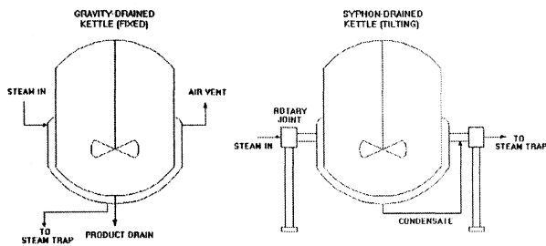
Figure 3. Types of steam-jacketed kettles
