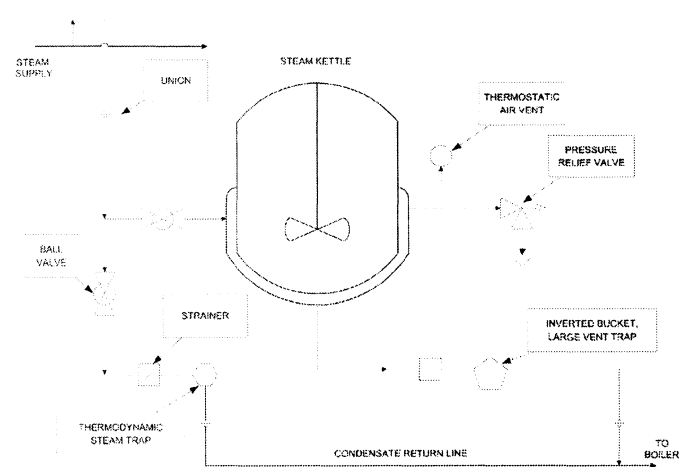
Figure 4. Suggested kettle hookup for gravity-drained kettle
