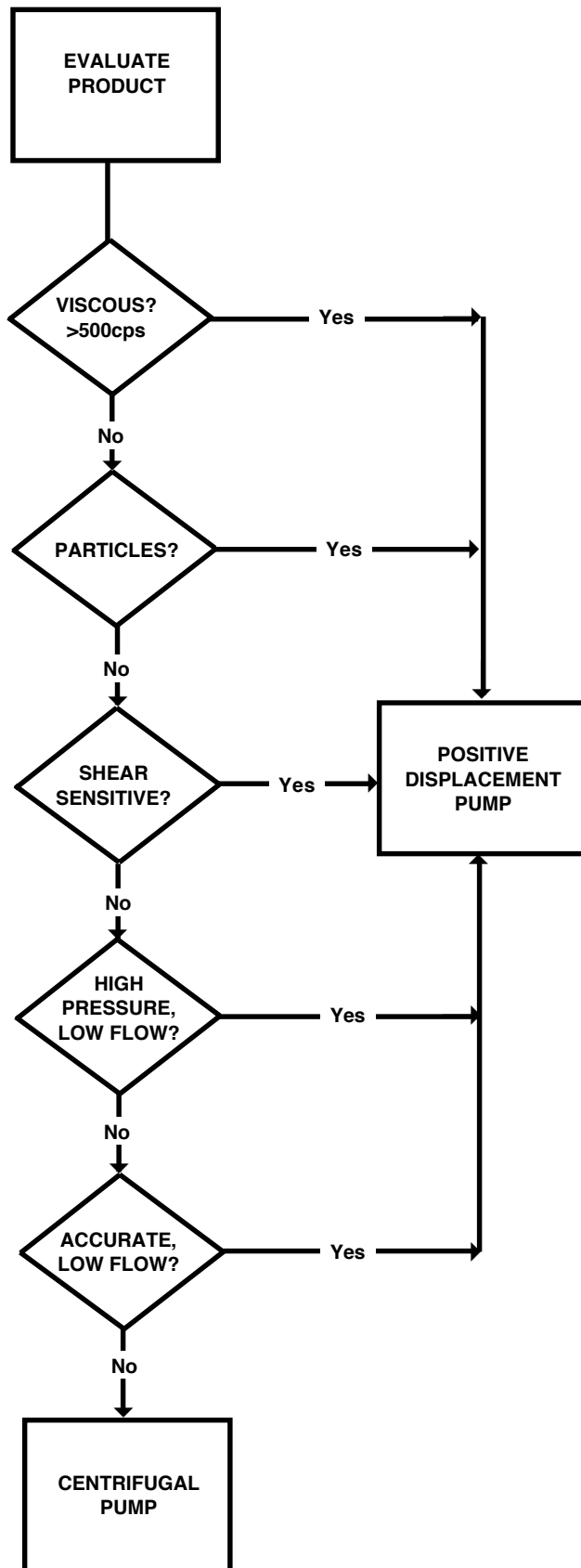
Figure 1. Decision tree for selecting sanitary pump classification.
