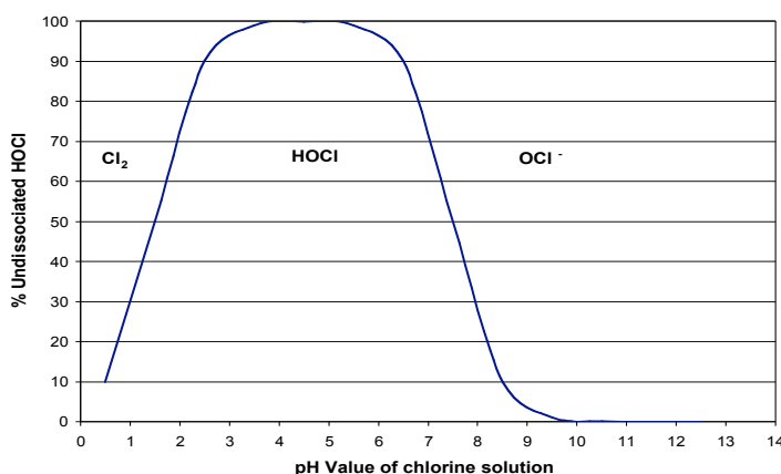
Figure 1 -- Effect of pH on hypochlorous acid content.
