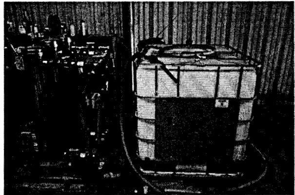
Figure 2: On-farm biodiesel filtration system.
