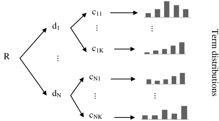
Fig.2 Generative process of ME model 1 ②
