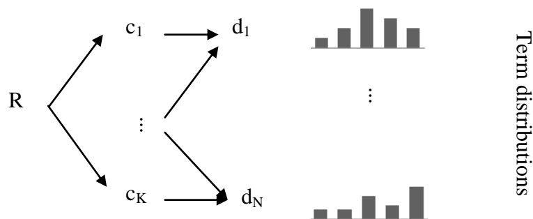
Fig.3 Generative process of ME model 2
