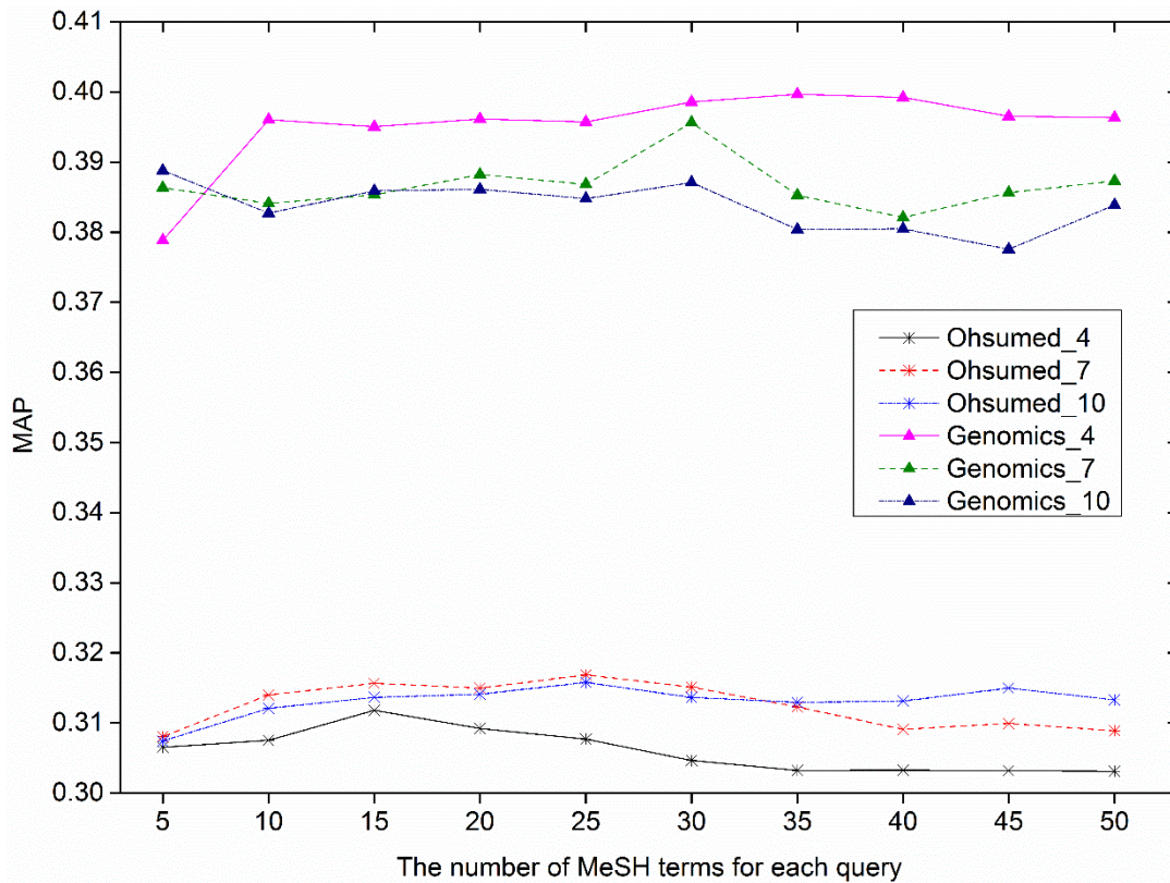
Fig.10 Performance of using different number of MeSH terms (the parameter |c| ) for each query in the Model2(Experimental runs using 4,7 and 10 pseudo-feedback documents respectively)
