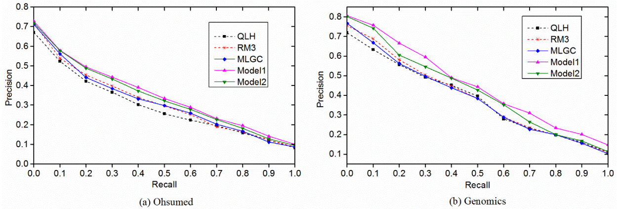
Fig.4 Precision-Recall curves for Ohsumed and Genomics
