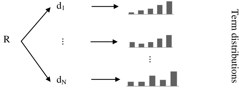
Fig.1 Generative process of RM3
