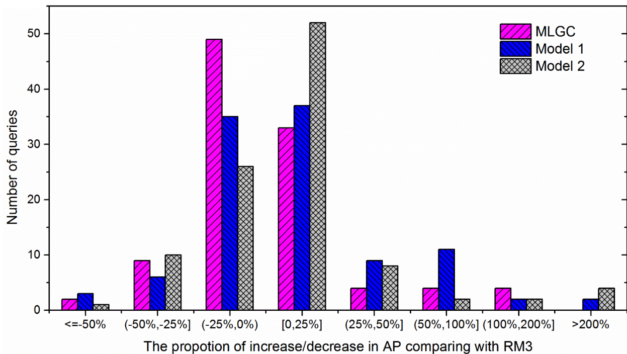
Fig. 5 The statistic of increased/decreased queries of MeSH-enhanced retrieval models compared with RM3 in Ohsumed
