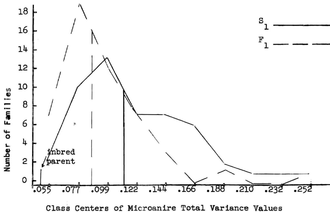
Fig. 2 Frequency distributions of variances of Micronaire readings on S_1 progenies of 50 Stoneville 62 plants and on the F_1 's of their crosses with inbred Washington.
