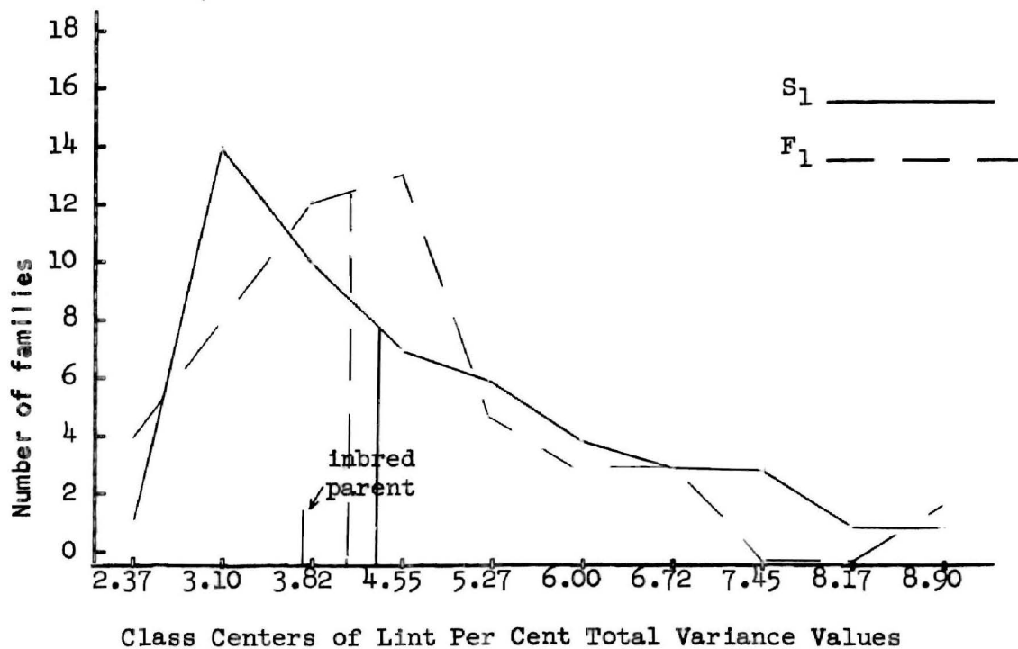
Fig. 4 Frequency distributions of variances of lint per cent values on S_1 progenies of 50 Stoneville 62 plants and on the F_1 of their crosses with inbred Washington.
