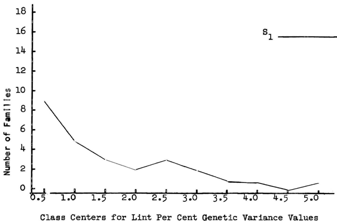
Fig. 3 Frequency distribution of genetic variance present for lint per cent in 50 Stoneville 62 S_1 progenies.
