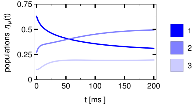
FIG. 3. (Color online) Dynamics of the fractional band populations n_\mu = \sum_{m^z} N_{\mu, m^z} / N_{\text{total}} in the Floquet realization of the Harper-Hofstadter model for the experimental parameters with a transverse harmonic confinement summed over the m^z oscillator quantum number. Colours correspond to the bands shown in Fig. 1.
