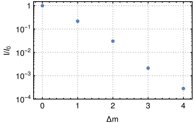
FIG. 2. (Color online) Overlap matrix element I_{\Delta m} = |\langle \langle \Phi_f^{\Delta m}(x, y) | H_{\text{int}} | \Phi_i^0(x, y) \rangle \rangle|^2 of the wavefunctions of the 2 dimensional model for a transition (1, 1) \rightarrow (3, 3) summed over the final state momenta and averaged over the initial state momenta as a function of the photon transfer \Delta m normalised to the element at \Delta m = 0 .
