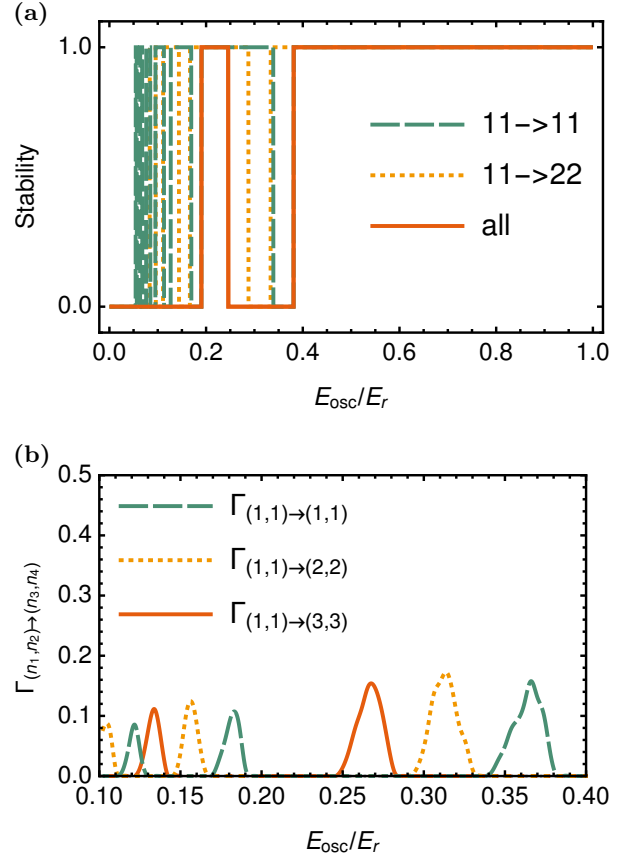
FIG. 7. (Color online) Stability of the groundstate band of the Harper-Hofstadter model to different inelastic transitions as indicated in the figure in the case of transverse confinement by a harmonic potential V_{\text{osc}}^z = \frac{1}{2}m\omega_{\text{osc}}z^2 in panel (a) and corresponding scattering rates in panel (b) both as a function of the oscillator energy E_{\text{osc}} = \hbar\omega_{\text{osc}} in terms of the recoil energy E_r .
