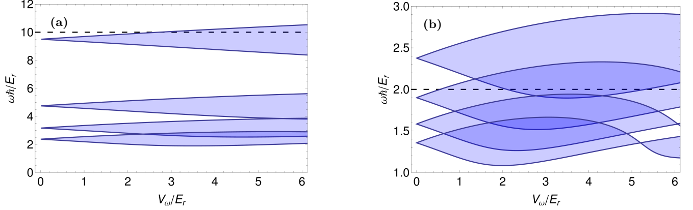
FIG. 9. (Color online) Stability diagram of the lowest band in a time-periodically modulated one-dimensional lattice of depth V_1 = 6E_r for which the band gap is 4.75E_r . Shaded regions correspond to energetically allowed scattering from the ground state into the first excited band. Different lobes correspond to different orders of the instability m starting with m = 1 at the top and increasing downwards. In (a) only the first 4 such lobes are shown for clarity, in (b) the region 1 \leq \omega\hbar/E_r \leq 3 with the m = 4, 5, 6, 7 lobes which overlap the m = 5 lobe are shown. The dashed lines of constant \omega\hbar/E_r correspond to the cuts along which the scattering rate is shown in Fig. 10.
