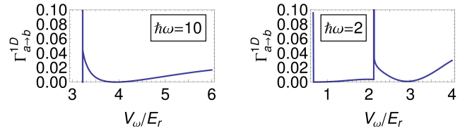
FIG. 10. (Color online) Dimensionless scattering rate \Gamma^{1D} , see Equation (79) along the cuts \hbar\omega/E_r = \text{const.} as indicated in Fig. 9 for particles in the first band (a) with momentum k = 0 scattering into the second band (b). The left corresponds to \hbar\omega/E_r = 10 for which m = 1 is the only scattering channel whereas the right corresponds to \hbar\omega/E_r = 2 for which m = 5 transitions are allowed for 0.6 \leq V_\omega/E_r \leq 6.9 and both m = 4, 5 for 2.1 \leq V_\omega/E_r \leq 5.3 .
