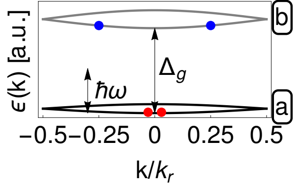
FIG. 8. (Color online) Quasienergies of the resonantly modulated lattice, Eq. (70) and (71), as a function of the quasi-momentum k in arbitrary energy units. The two lowest bands of the original lattice (a) and (b) both split into two subbands \tau = \pm which are degenerate at the Brillouin zone boundaries. Depicted is a typical situation in which the energy of the periodic modulation \hbar\omega is larger than the bandwidth of the lowest band and smaller than the bandgap \Delta_g . The balls show our initial state with two particles in the lowest band and a possible final state with two particles in the upper band after scattering. For this plot a nearest neighbour tight-binding dispersion \epsilon^{(n)}(k) = t^{(n)} \cos(k) is assumed with parameters t^a = 1.1 , t^b = 2.3 and \hbar\omega = 4.8 , \Delta_g = 10 and \kappa = 1
