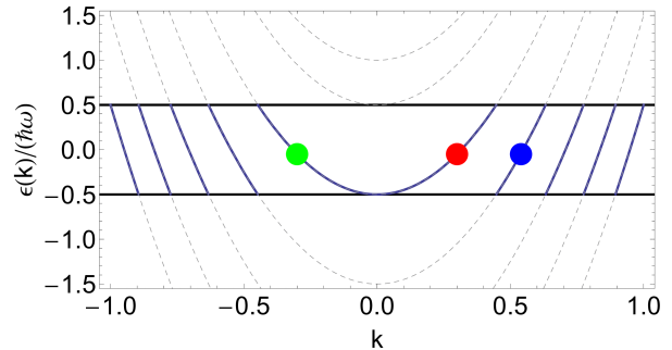
FIG. 1. (Color online) Unbounded single-particle dispersion \epsilon_k^0/(\hbar\omega) \propto k^2 as a function of dimensionless wavevector k reduced to the first BZ (bold) and continuous dispersion with periodically repeated images (dashed). Scattering an initial state (red/middle) to final state (green/left) would be considered elastic and scattering from initial state (red/middle) to a different branch (blue/right) would be considered inelastic. When regarding these processes with respect to the continuously defined dispersions, elastic scattering corresponds to no change in the Floquet index m whereas inelastic scattering changes m .
