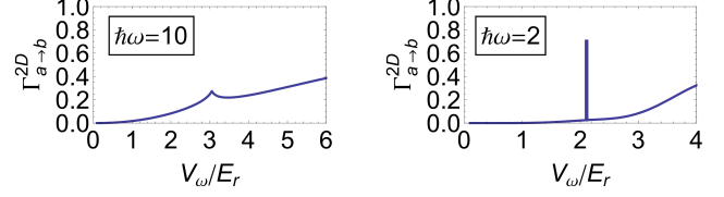
FIG. 11. (Color online) Dimensionless scattering rate \Gamma_{a \rightarrow b}^{2D} for the extension to a weakly-confined system with a free transverse degree of motion, see Equation (80) along the cuts \hbar\omega/E_r = \text{const.} as indicated in Fig. 9 for particles in the first band with quasi-momentum k = 0 and relative momentum k_y = 0 scattering into the second band, integrated over the final states with crystal momentum q and relative momentum q_y . The left corresponds to \hbar\omega/E_r = 10 for which m \geq 1 are the available inelastic scattering channel whereas the right corresponds to \hbar\omega/E_r = 2 for which m \geq 5 transitions are allowed for 0.6 \leq V_\omega/E_r \leq 6.9 and m \geq 4 for 2.1 \leq V_\omega/E_r \leq 5.3 .
