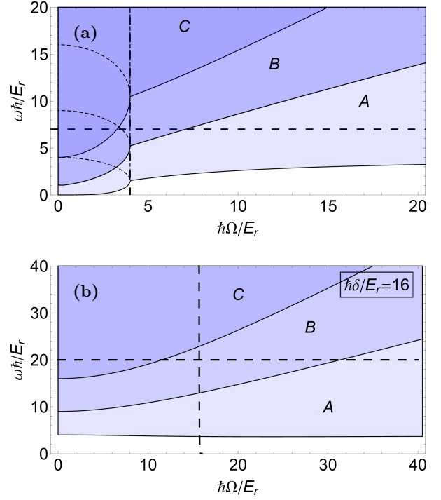
FIG. 4. (Color online) Stability diagram for (a) \hbar\delta/E_r = 0 and (b) \hbar\delta/E_r = 16 with initial state of two particles with quasi-momentum k = k_0 in lower band. For no detuning and \hbar\Omega/E_r < 4 both cases of k = +|k_0| (dashed lines) and k = -|k_0| (full lines) are shown, with detuning the minimum is unique. Shaded regions correspond to parameter regimes in which inelastic scattering is allowed. The bottom region (A) in light blue corresponds to inelastic scattering where both particles remain in the lower bands, i.e. the (-, -) -final state, in the middle region (B) particles can scatter either into the (-, -) or the (+, -) -final state and in the top region (C) scattering into all states (-, -) , (+, -) and (+, +) is allowed. The thick dashed lines of constant \omega\hbar/E_r and of constant \Omega\hbar/E_r correspond to the cuts along which the scattering rate is shown in Fig. 5 and Fig. 6.
