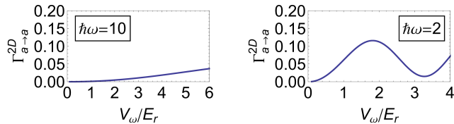
FIG. 12. (Color online) Dimensionless scattering rate \Gamma_{a \rightarrow a}^{2D} for the extension to a weakly-confined system with a free transverse degree of motion, see Equation (80) along the cuts \hbar\omega/E_r = \text{const.} as indicated in Fig. 9 for particles in the first band with quasi-momentum k = 0 and relative momentum k_y = 0 scattering inelastically and remaining in the first band, integrated over the final states with crystal momentum q and relative momentum q_y . The left corresponds to \hbar\omega/E_r = 10 and the right corresponds to \hbar\omega/E_r = 2 . In both cases all processes with m \geq 1 are inelastic and allowed as the particles remain in the same band and the energy in y direction is not gapped.
