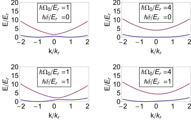
FIG. 3. (Color online) Dispersion E/E_r as a function of k/k_r , see Equation (50), including an energy offset to have zero minimum. The top row shows the dispersion for \hbar\delta/E_r = 0 and \hbar\Omega/E_r = 1 to the left and \hbar\Omega/E_r = 4 to the right and the bottom row for the same parameters in the case of \hbar\delta/E_r = 1 .
