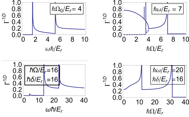
FIG. 5. (Color online) Dimensionless scattering rate \Gamma^{1D} , see Equation (54) for an initial state with particles in the lower band with momentum k = \pm|k_0| getting inelastically scattered. In the top row for no detuning \hbar\delta/E_r = 0 as a function of \omega\hbar/E_r for fixed \hbar\Omega/E_r = 4 to the left and as a function of \hbar\Omega/E_r for fixed \hbar\omega/E_r = 7 to the right (dashed k = +|k_0| , full k = -|k_0| ) and at the bottom for \hbar\delta/E_r = 16 as a function of \omega\hbar/E_r for fixed \hbar\Omega/E_r = 16 to the left and as a function of \hbar\Omega/E_r for fixed \hbar\omega/E_r = 20 to the right as indicated in Fig. 4. The rate shows divergences at the opening/closing of scattering channels corresponding to the borders in Fig. 4 at which the density of states of the final states diverges.
