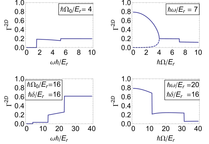
FIG. 6. (Color online) Dimensionless scattering rate \Gamma^{2D} , see Equation (59) for an initial state with particles in the lower band with momentum k = \pm|k_0| and relative momentum k_y = 0 getting inelastically scattered for the extension to a 2D setting with free motion in a transverse direction. In the top row for no detuning \hbar\delta/E_r = 0 as a function of \omega\hbar/E_r for fixed \hbar\Omega/E_r = 4 to the left and as a function of \hbar\Omega/E_r for fixed \omega\hbar/E_r = 7 to the right (dashed k = +|k_0| , full k = -|k_0| ) and at the bottom for \hbar\delta/E_r = 16 as a function of \omega\hbar/E_r for fixed \hbar\Omega/E_r = 16 to the left and as a function of \hbar\Omega/E_r for fixed \omega\hbar/E_r = 20 to the right as indicated in Fig. 4. The rate shows jumps at the opening/closing of scattering channels corresponding to the borders in Fig. 4.
