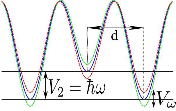
FIG. 7. (Color online) Sketch of the one-dimensional time-periodically driven lattice potential given in Eq. (60). The lattice is staggered with an energy offset V_2 between neighbouring sites which suppresses tunneling along the lattice. Tunneling is then restored by resonantly modulating the site-energies with a modulation strength V_\omega at frequency \hbar\omega = V_2
