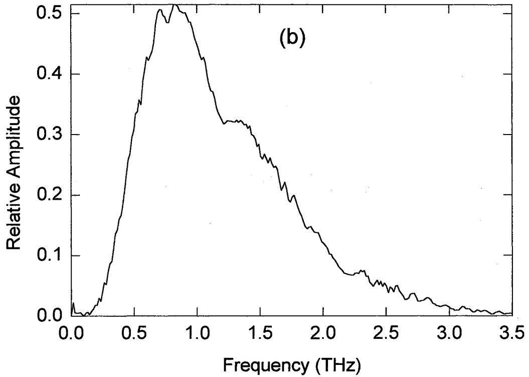
Figure 3-4. Measured propagated pulse through the long waveguide (a), and its amplitude spectrum (b).
