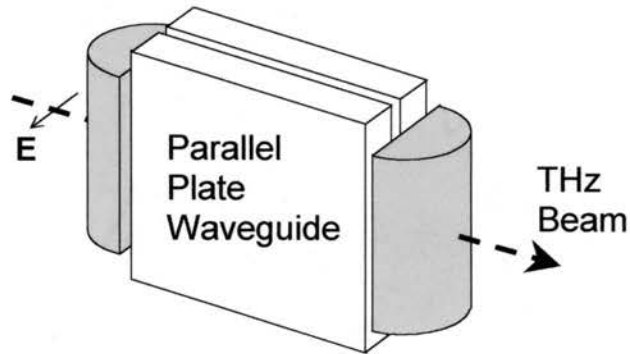
Figure 4-1. The lens-waveguide-lens system. The plate separation has been exaggerated for clarity.
