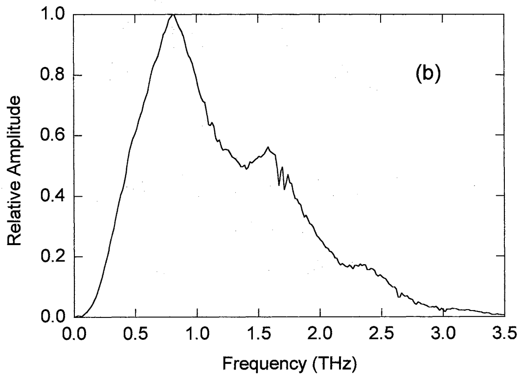
Figure 3-2. Measured reference pulse (a), and its amplitude spectrum (b).
