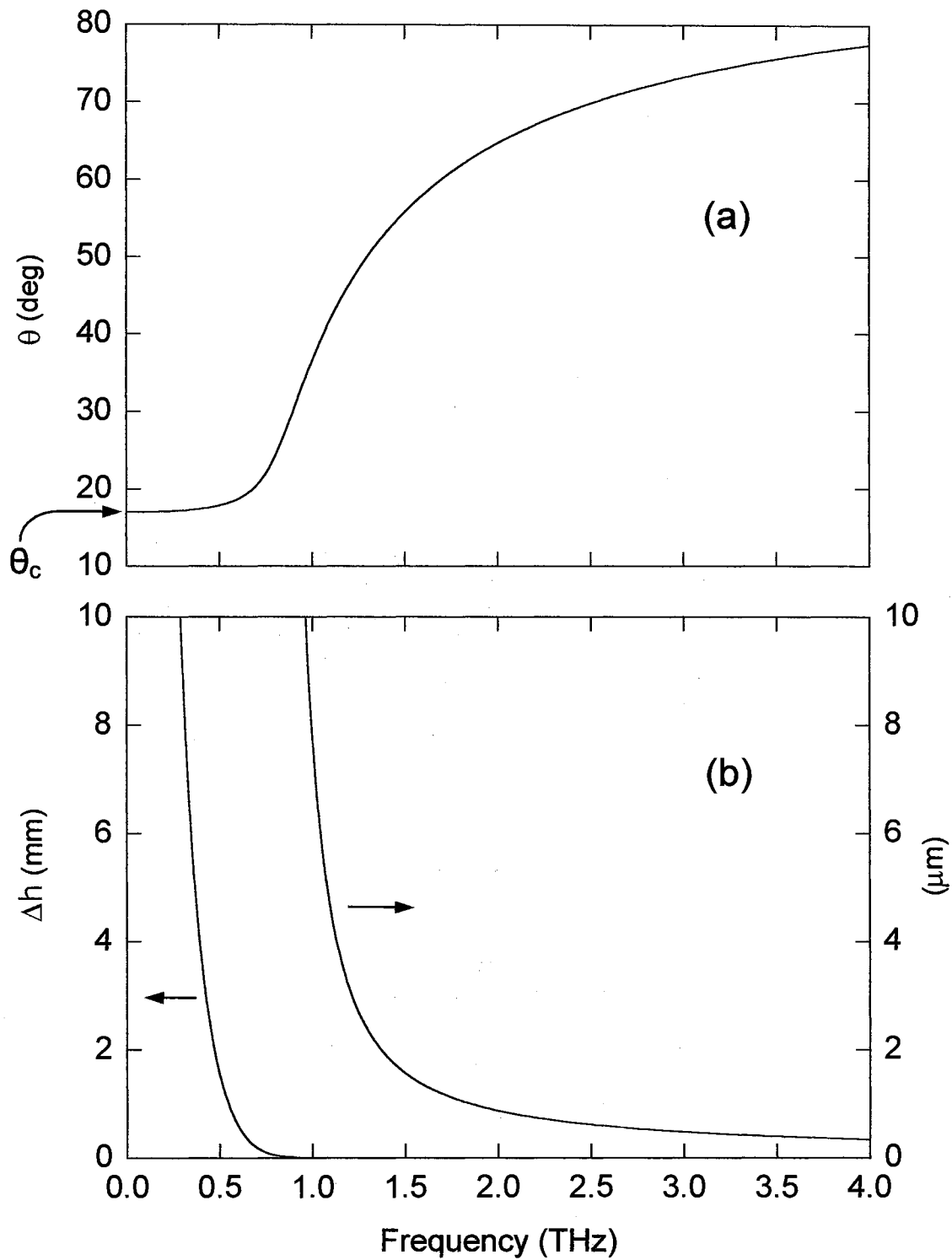
Figure 6-4. (a) Variation of \theta with frequency for the \text{TM}_0 mode. (b) Variation of \Delta h with frequency, plotted to two different vertical scales. The curve on the left corresponds to mm, and the curve on the right corresponds to \mu\text{m} .
