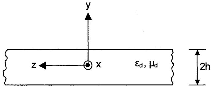
Figure 3-5. Longitudinal cross-section of the dielectric slab waveguide.
