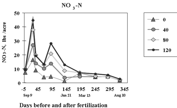
Figure 2.5. Surface soil (0-6") ammonium and nitrate nitrogen following fertilization at different rates from OSU Soil Fertility Research.
