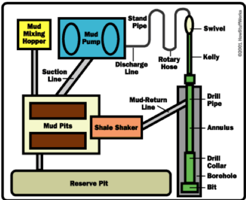
Figure 8.1. A typical schematic of drilling fluid/mud use during oil and gas drilling operations (from howstuffworks.com). Note the mud return line that allows removal of the drill cuttings from the borehole and recycling through the shale shaker.
