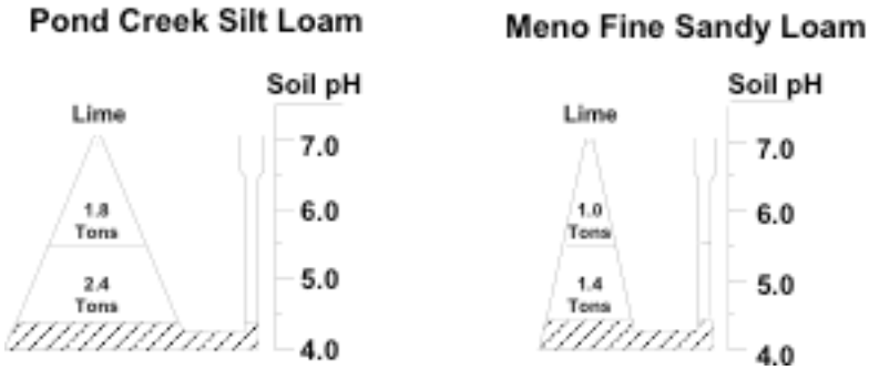
Figure 3.3 Reservoirs of soil solids in clayey vs. sandy soil.
