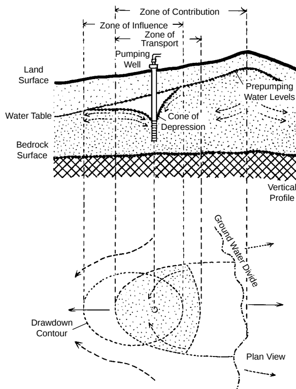
Figure 4. Diagram of ground water flow and zone of contribution around a pumping well.
