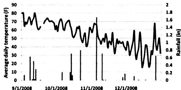
Figure 1. Average daily temperature and rainfall from Sept. 1, 2008 to Dec 31, 2008, Stillwater, Okla.
