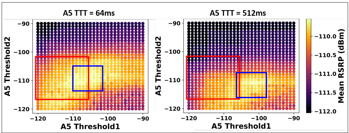
Fig. 3.3: Comparison of gold standard and simulation results. Red box represents the range of threshold values recommended by the gold standard used in industry. Blue box is the area of high mean RSRP, for analyzed network scenario. This finding can be insightful for the industry.
