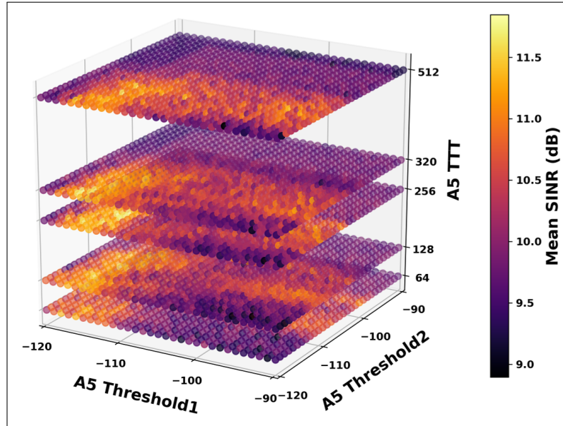
Fig. 3.2: Impact of A5 thresholds and TTT on mean SINR.
