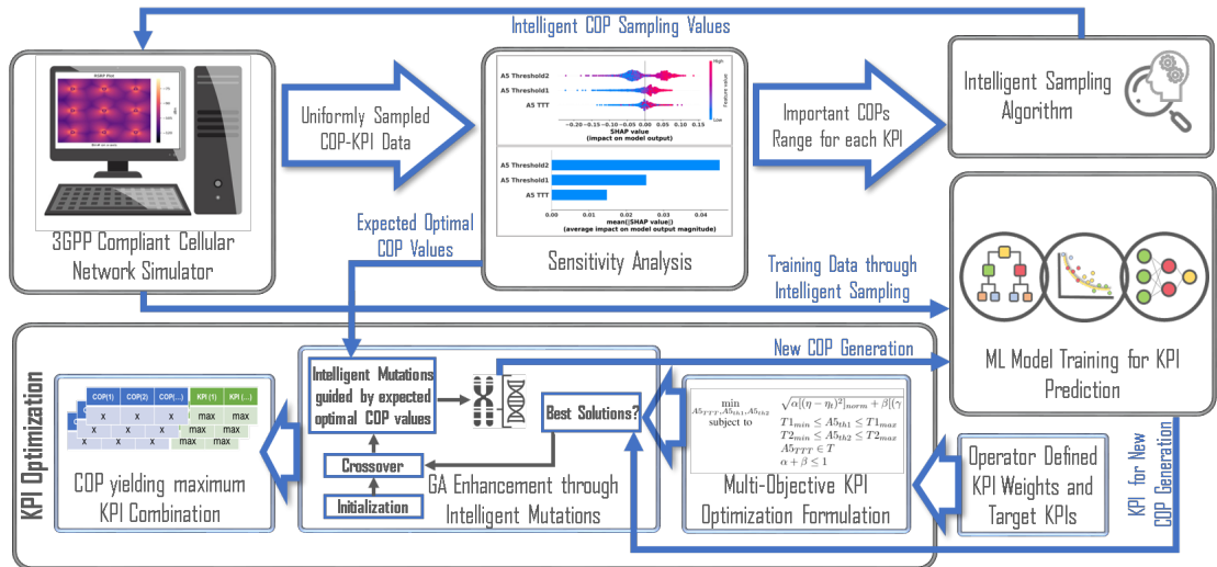
Fig. 1.1: Closed loop self-optimization framework for cellular networks.
