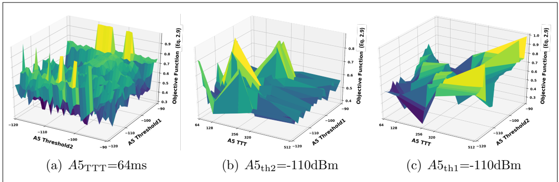
Fig. 5.1: Objective function defined in eq. (2.9) with \alpha = 0.33 , \beta = 0.33
