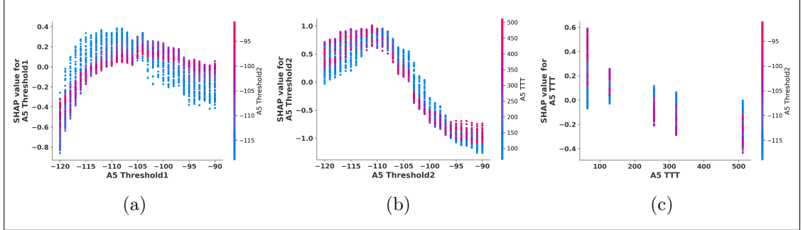
Fig. 4.2: Impact of each parameter on RSRP and their inter-dependence
