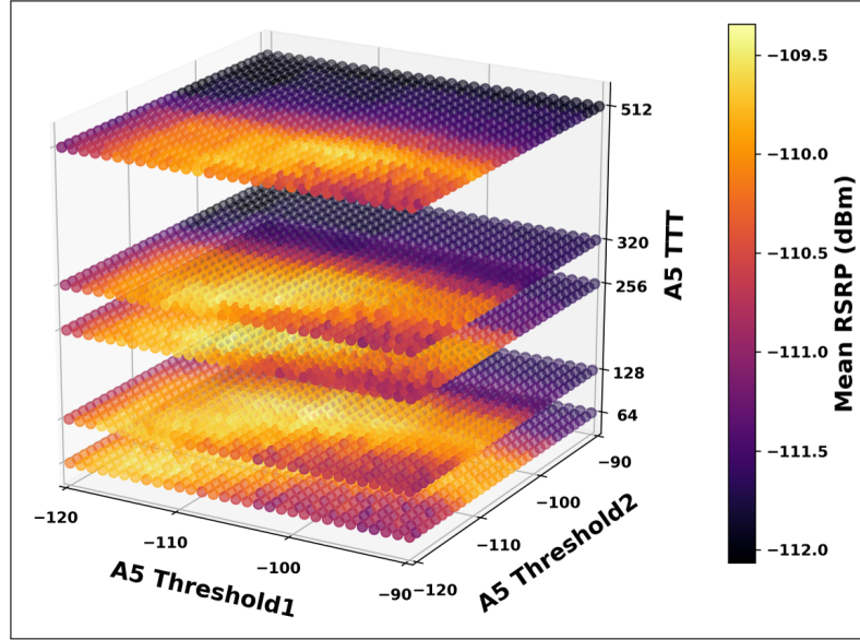
Fig. 3.1: Impact of A5 thresholds and TTT on mean RSRP.
