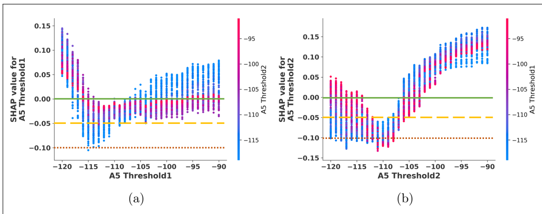
Fig. 5.2: Dependence plot of A5_{th1} and A5_{th2} for the utility function with \alpha = 0.33 and \beta = 0.33
