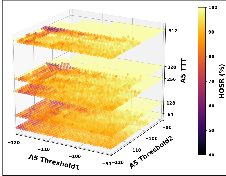
Fig. 3.4: Impact of A5 thresholds and TTT on HOSR.
