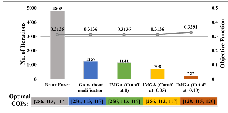
Fig. 5.3: Convergence time and objective function comparison between brute force, GA and intelligently mutated GA with different SHAP value cutoff.
