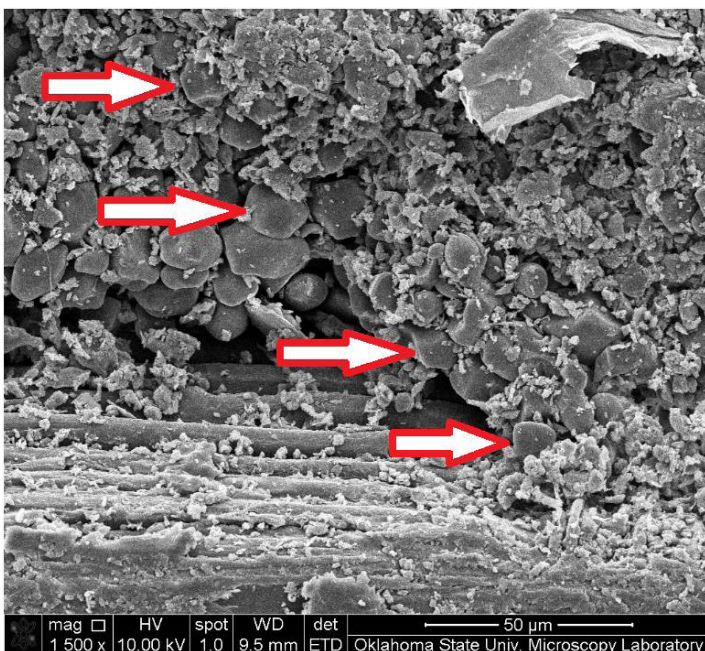
Figure 4. Scanning electron microscope showing distribution of starch particulars in the panels.
