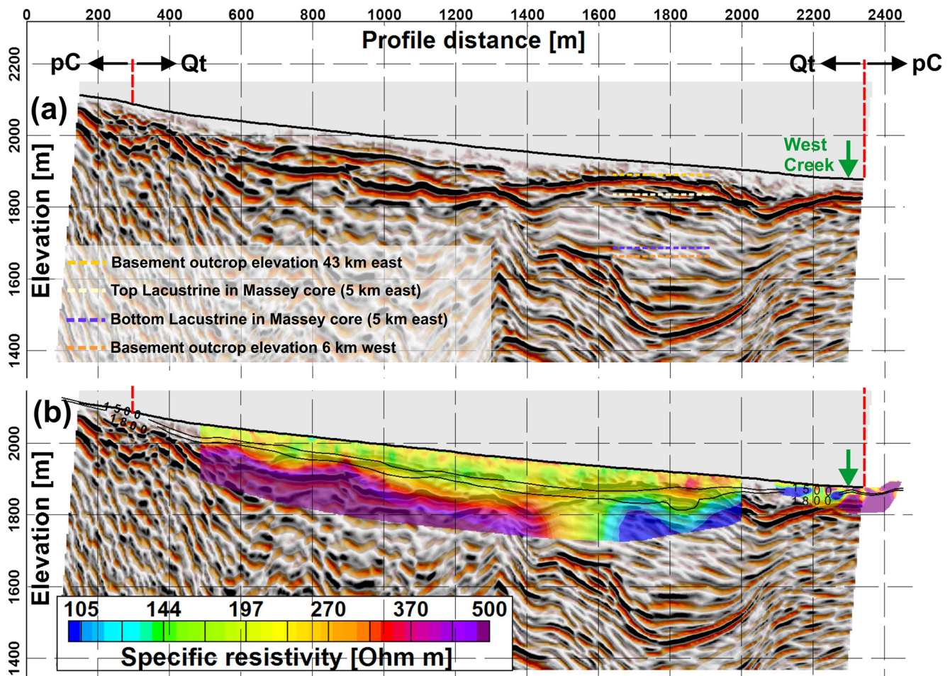
Figure 2. (a) Depth-converted prestack seismic time migration (PSTM) image and ground-truth data. Pc, Qt: Precambrian and Quaternary surface cover. Dashed lines: Elevations of basement outcrops along Unaweep Canyon and interpreted horizons in the Massey core. (b) Electrical resistivity tomography image superimposed on the PSTM image.
