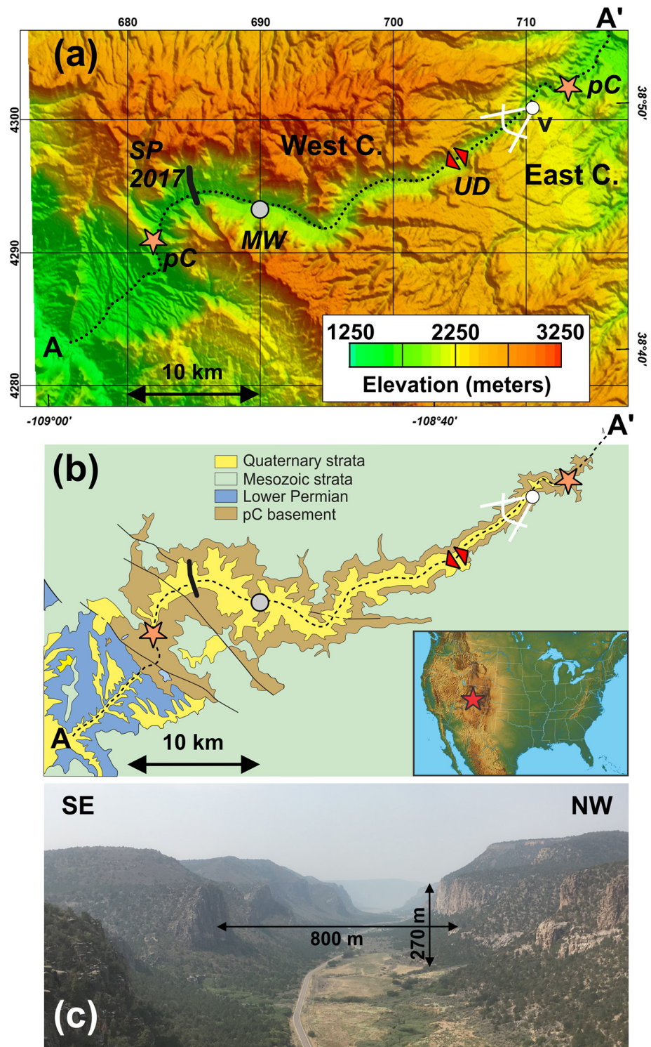
Figure 1. (a) Digital elevation model of Unaweep Canyon. UD (red triangles): Unaweep Divide; MW (gray dot): Massey well (core); SP 2017 (black line): Location of the seismic reflection profile in this study; pC (orange stars): Precambrian basement outcrops along the canyon floor; A-A': Longitudinal cross-section shown in Figure 5; v: Viewpoint of the photograph shown in (c). (b) Geologic map. (c) View into eastern Unaweep Canyon toward west.
