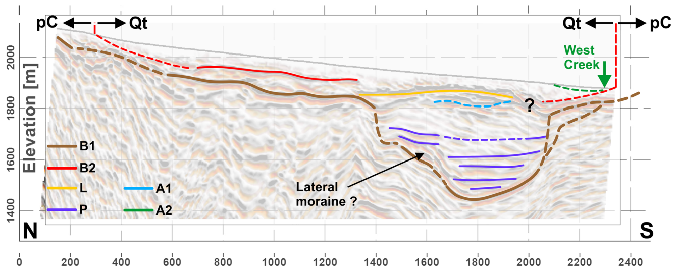
Figure 3. Integrated interpretation of the depth-converted prestack seismic time migration image, ground-truth data, and additional geophysical observables (Figures S4–S6). Dashed lines indicate where horizons are less well defined and/or are largely based on Supporting Information S1. B1: Consolidated Precambrian basement. The two different configurations at profile distances >2,000 m are explained in the text. B2: Top of Precambrian regolith and pre-Quaternary sediments; L: Reflector associated with a Cenozoic lacustrine unit; P: Pre-Quaternary strata; A1, A2: Deep and shallow aquifers.
