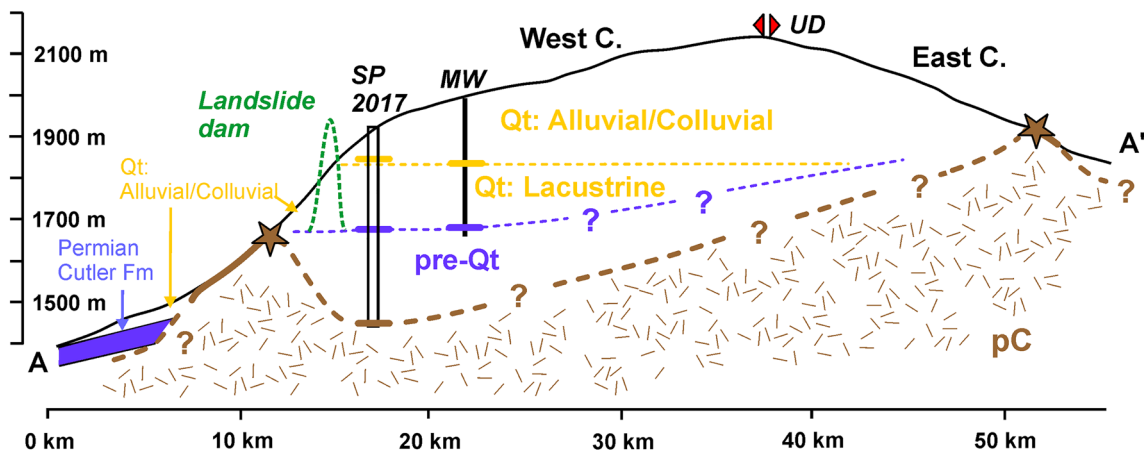
Figure 5. Hypothesized vertical section along Unaweep Canyon following profile A-A' (Figure 1). Black solid line: Topography along West and East Creek. UD: Unaweep divide; MW: Massey well; SP 2017: Location of seismic profile. Yellow line: Top of the lacustrine unit. Purple line: Top of pre-Quaternary strata. Brown line: Precambrian basement. Solid yellow/purple bars and brown lines show observations from the seismic profile, the well, and surface geology. Location of the 1.4–1.3 Ma landslide dam according to Balco et al. (2013).
