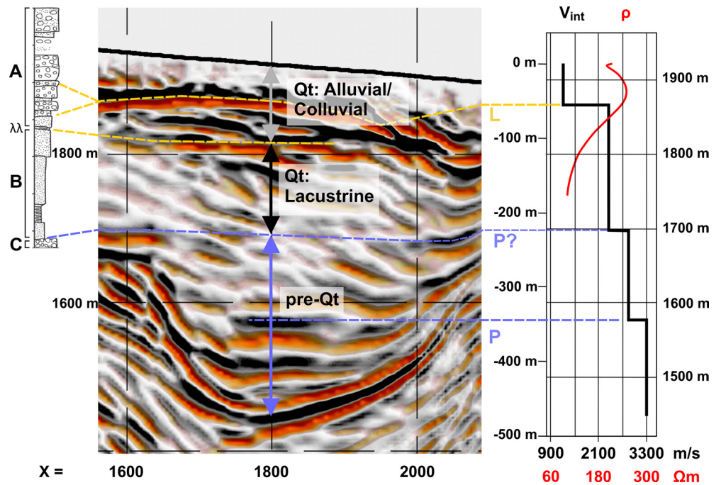
Figure 4. Correlation of the overdeepened section with the stratigraphy of the distant Massey core, interval velocities ( V_{int} ), and electrical resistivity ( \rho ). V_{int} and \rho are extracted at the central location X = 1,800 m. Discrepancies in elevation are attributed to the approximate velocity model, the distance (5 km) to the core, and lateral variation along the seismic section. Vertical axis represents elevation and depth below surface. “L” and “P”: top of interpreted reflectors. Core sections after Balco et al. (2013): A—Qt alluvium/colluvium; \lambda\lambda —Paleosoils; B—Qt lacustrine; and C—Pz Diamict.
