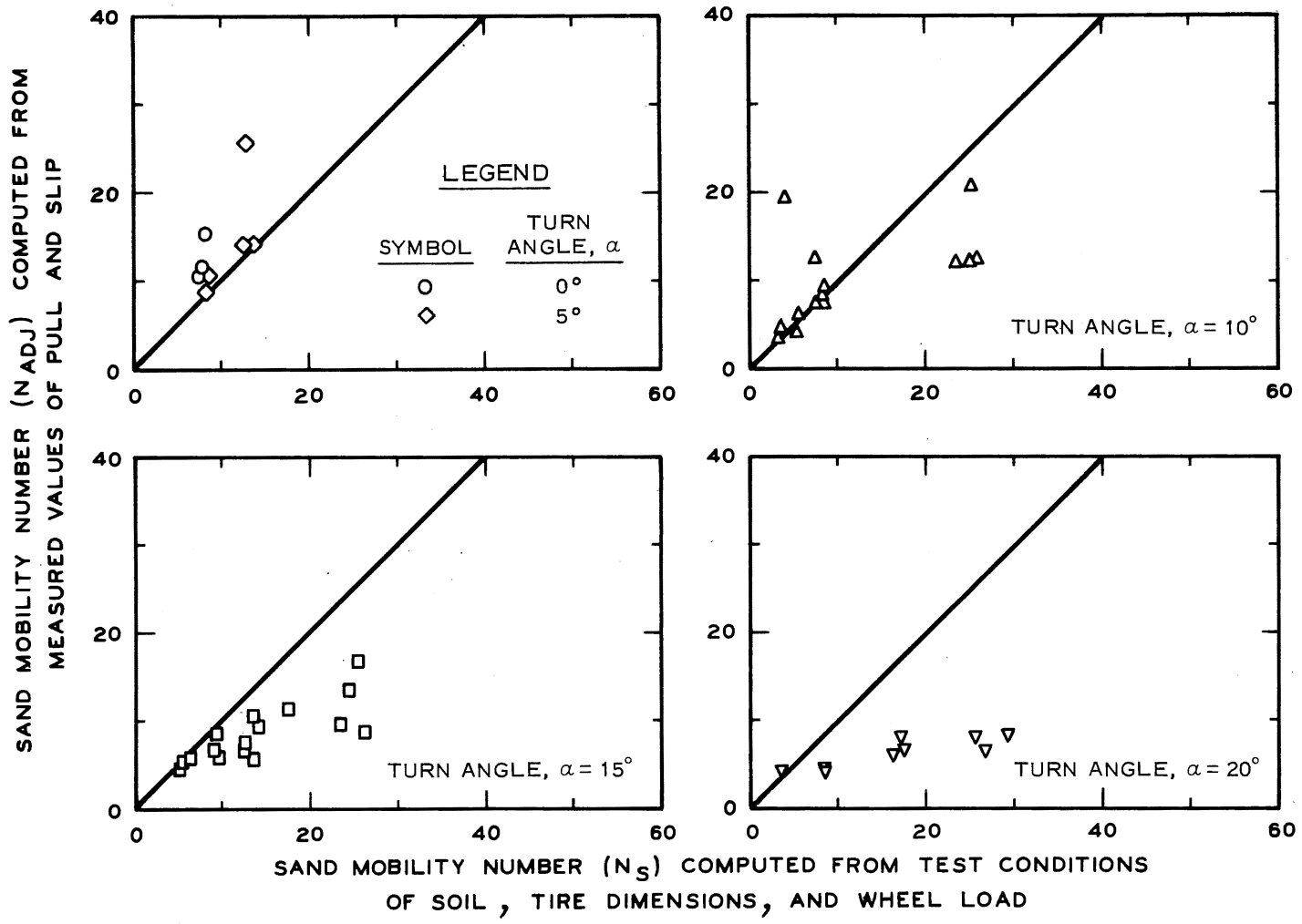
Figure 4.13. Comparison of Sand Mobility Numbers as Computed from Dependent Performance Parameter of Pull Versus Independent Test Variables.
