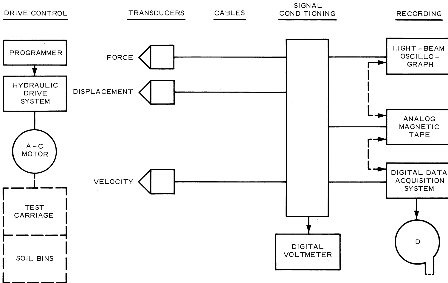
Figure 3.14. Flow Chart for Measurement and Control Systems.
