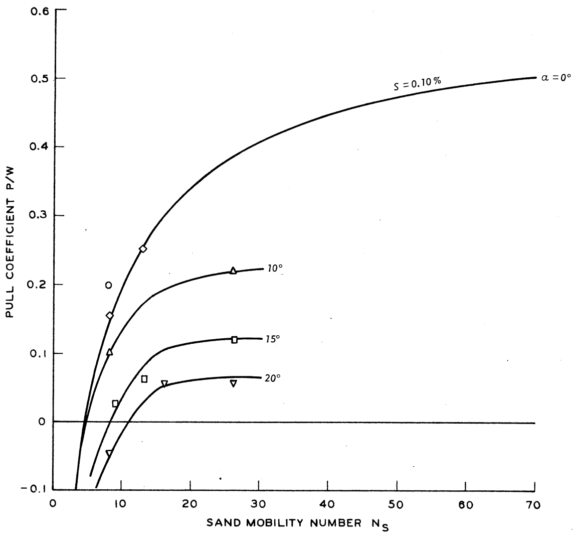
Figure 4.22. Pull Coefficient Versus Sand Mobility Number, Wheel Slip = 10 Percent.
