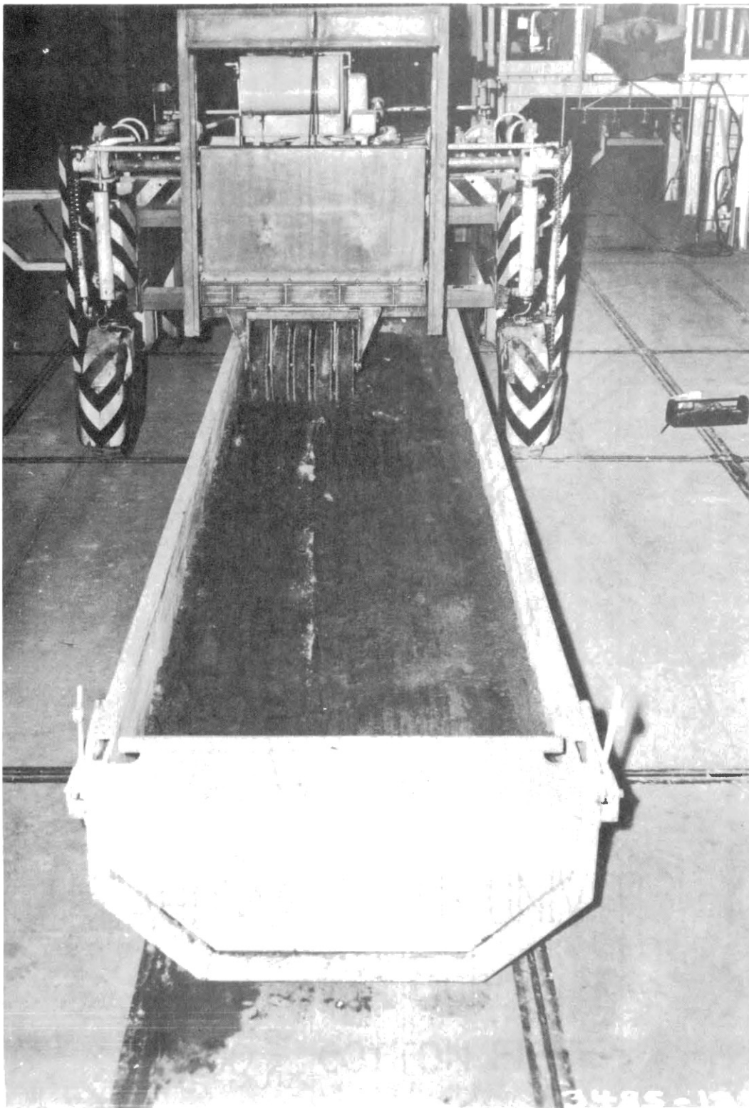
Figure 3.6. Straddle Truck Equipped with Pneumatic Tired Compactor.
