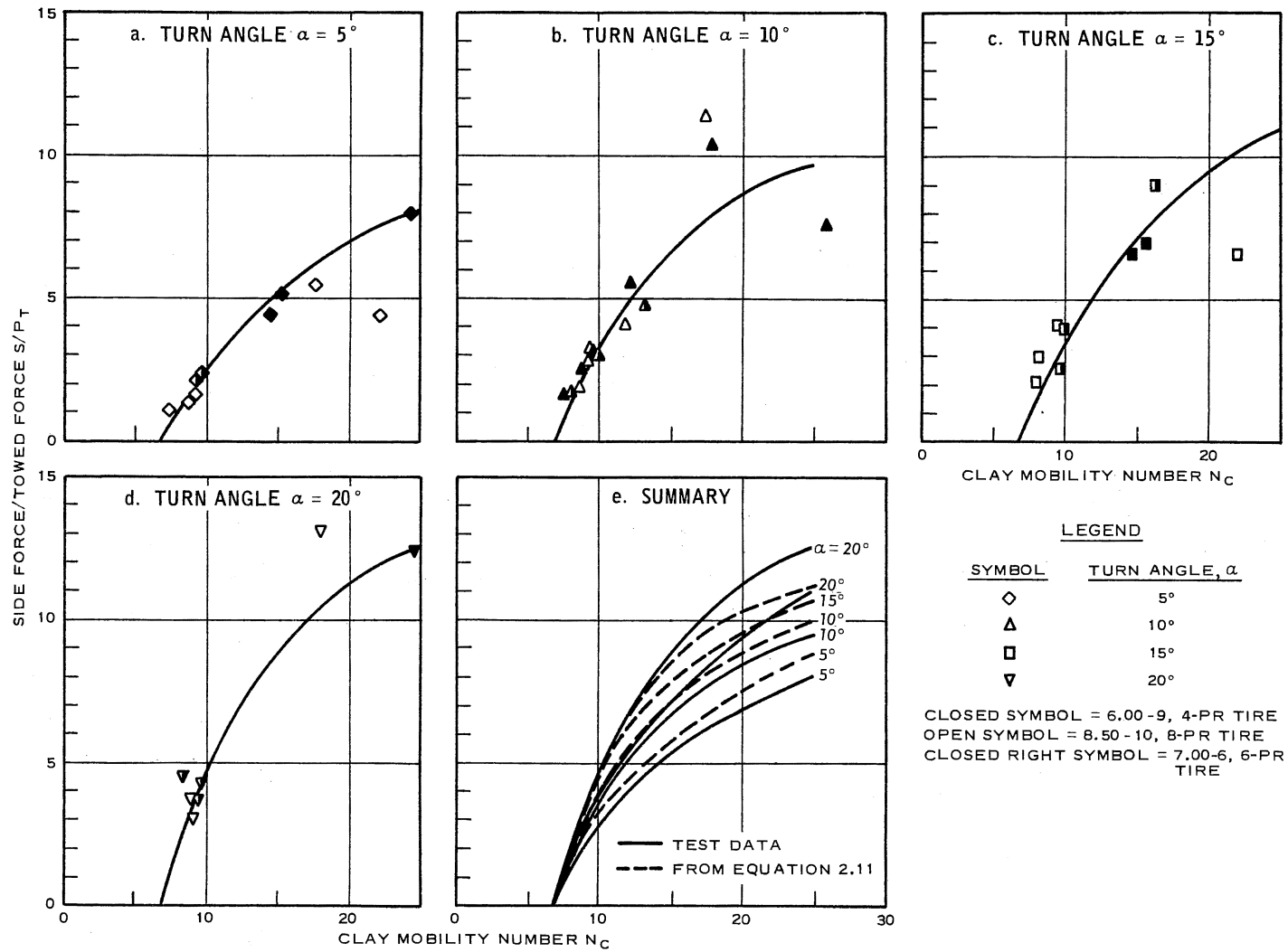
Figure 2.10. Ratio of Side Force/Towed Force as a Function of Clay Mobility Number and Wheel Turn Angle (Data from Melzer, 1976).
