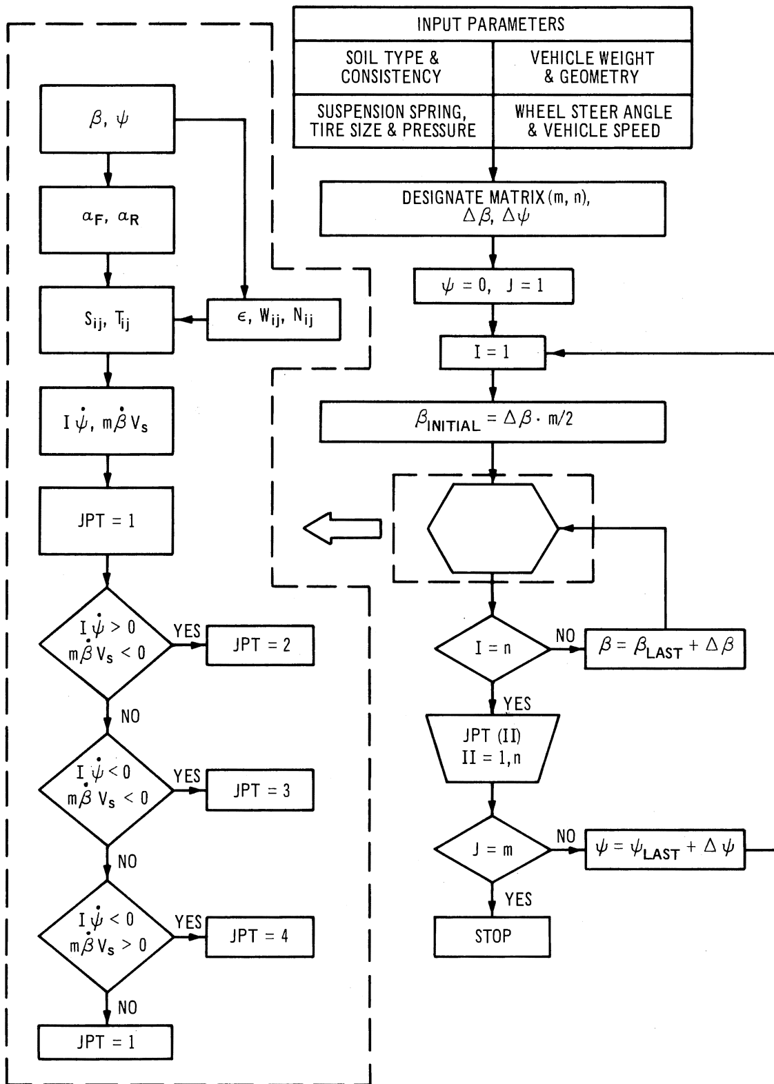
Figure 5.6. Flow Diagram for Finding Real Zeros.
