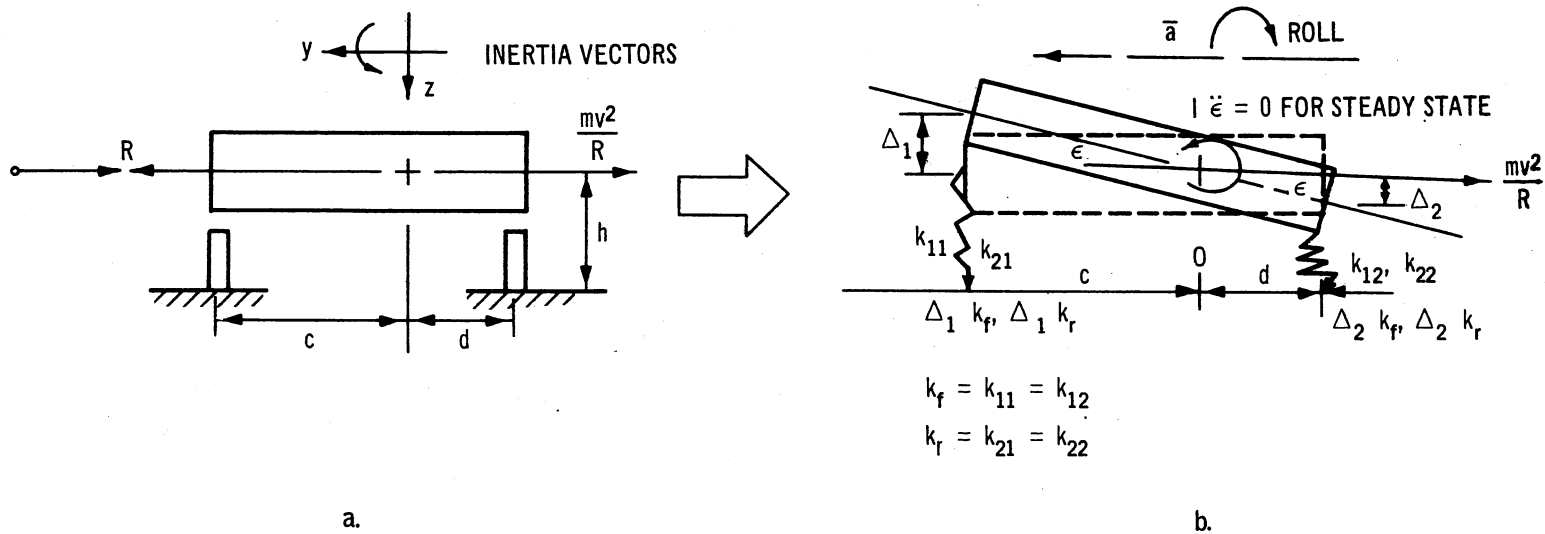
Figure 5.2. Roll Angle of a Vehicle in a Steady-State Turn.
