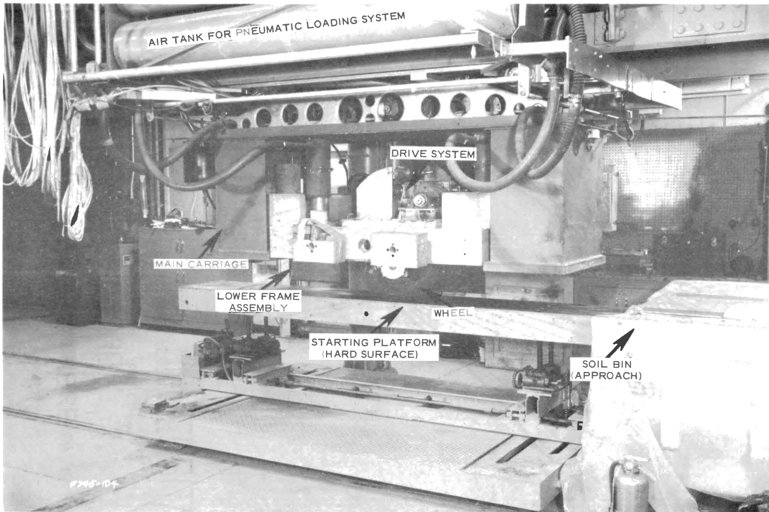
Figure 3.10. Overall View of Dynamometer Carriage.
