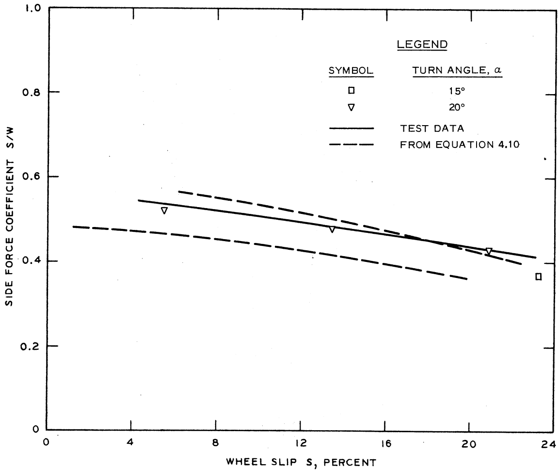
Figure 4.35. Influence of Turn Angle on Side Force Coefficient. Average Cone Penetration Resistance Gradient G = 2.0 , Tire Deflection \delta/h = 0.35 , Design Wheel Load W = 1,000 \text{ N} . Desired Sand Mobility Number N_s = 16.4 .
