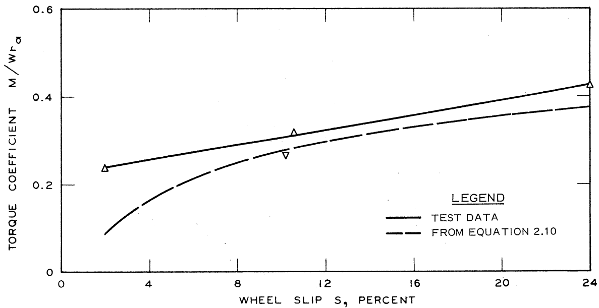
b. TORQUE COEFFICIENT
