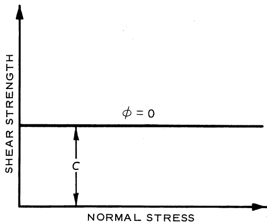
a. MOHR-COULOMB REPRESENTATION OF PURELY COHESIVE SOIL
