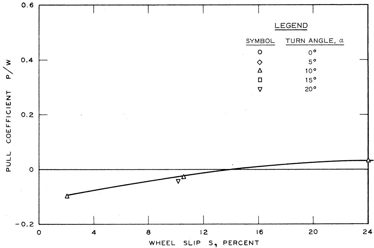
a. PULL COEFFICIENT
