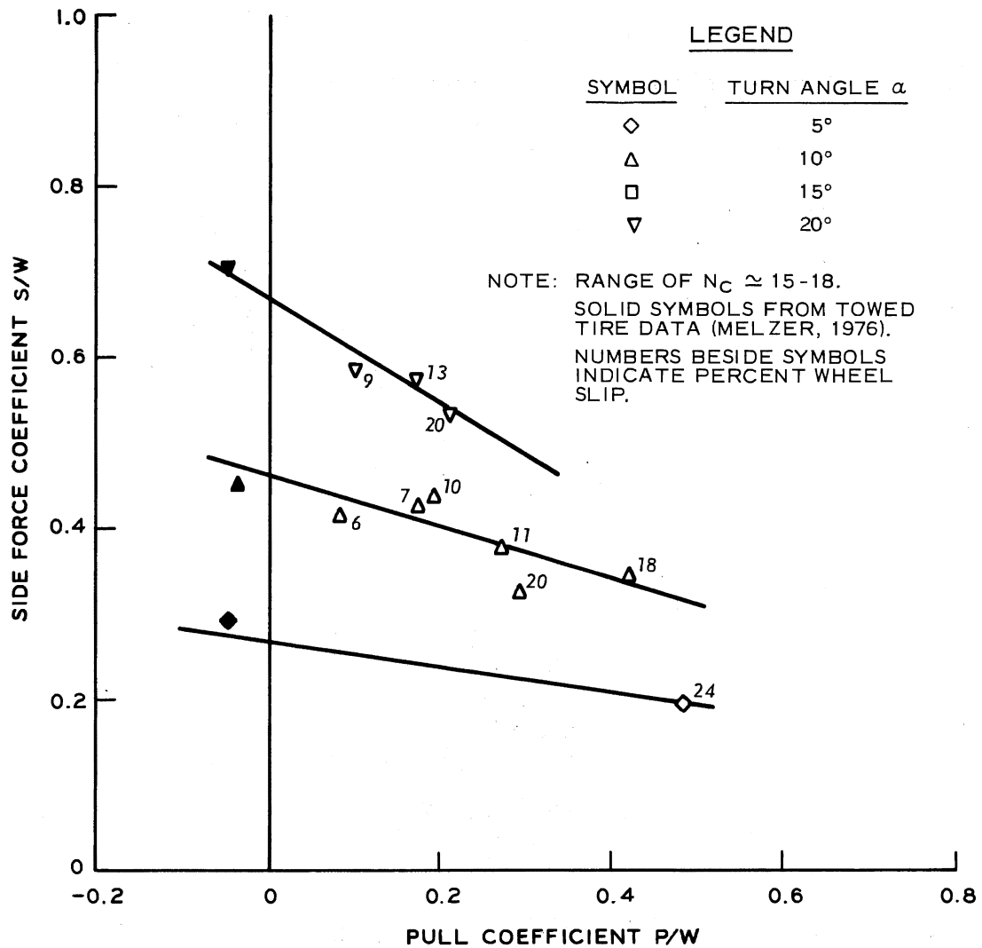
Figure 4.4. Side Force Versus Pull Coefficient for 6.00-9, 4-PR Tire on Clay. Cone Penetration Resistance C = 290 kPa. Clay Mobility Number N_c \approx 15 to 18 .
