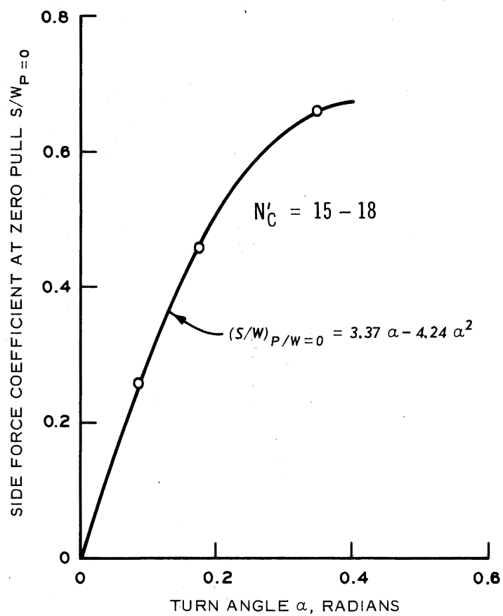
Figure 4.7. Side Force Coefficient at Zero Pull Versus Turn Angle \alpha . Data Points Extrapolated from Figure 4.4. Clay Mobility Number N'_c = 15 to 18.
