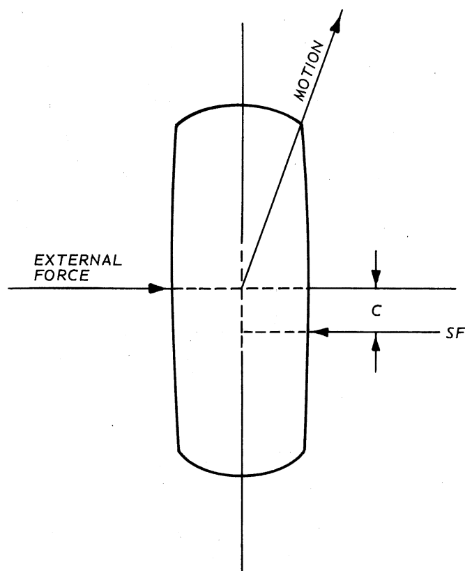
Figure 2.3. Development of Trail Moment SF \cdot C from an Externally Applied Force.
