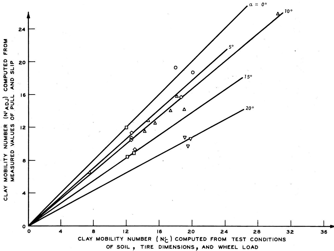
Figure 4.2. Comparison of Clay Mobility Numbers as Computed from Dependent Performance Parameter of Pull Versus Independent Test Variables.
