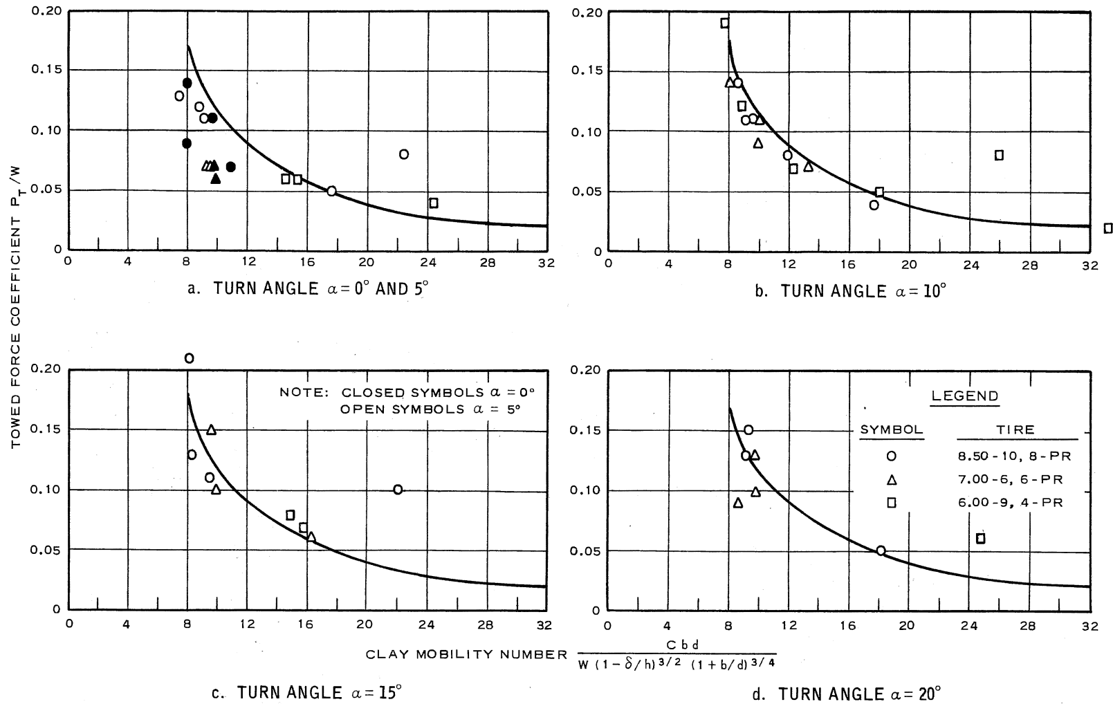
Figure 2.9. Towed Force Coefficient as a Function of Clay Mobility Number and Wheel Turn Angle (Data from Melzer, 1976).
