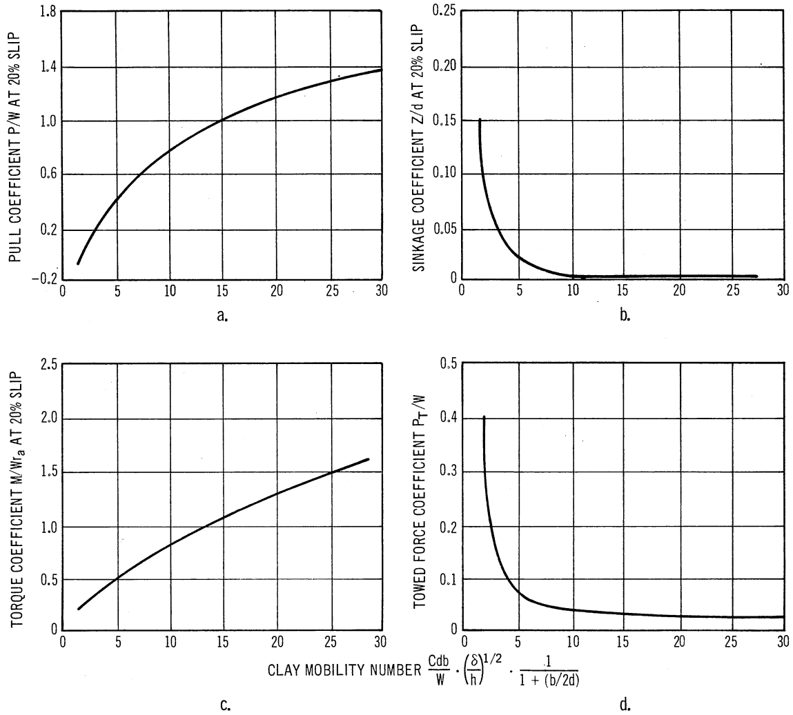
Figure 2.4. Relation of Performance Coefficients to Clay Mobility Number (after Turnage, 1972, Figure 4 ).
