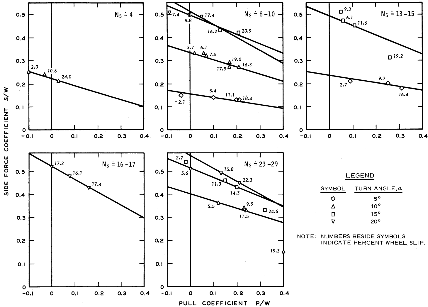
Figure 4.28. Side Force Versus Pull Coefficient for 6.00-9, 4-PR Tire on Sand for Various Values of Sand Mobility Number N_s .
