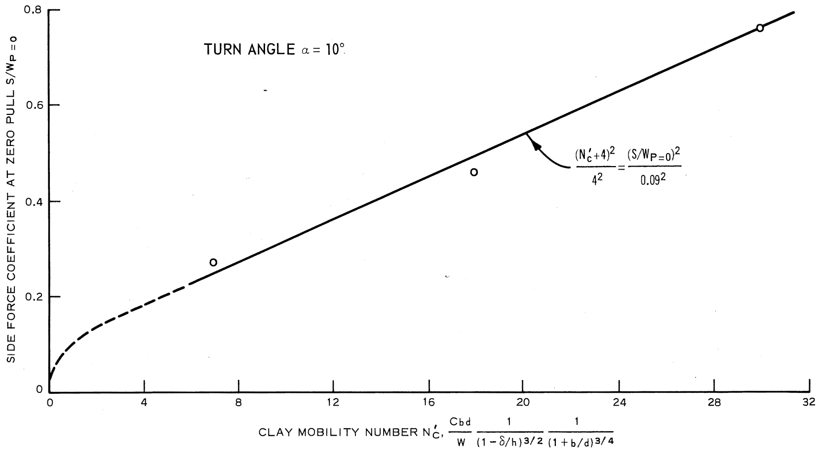
Figure 4.8. Side Force Coefficient at Zero Pull Versus Clay Mobility Number for a Turn Angle of 10 Degrees.
