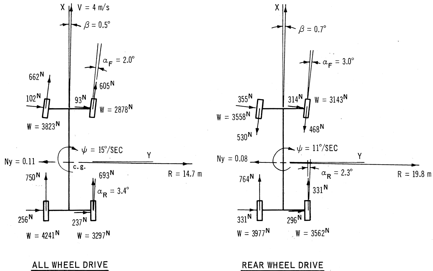
Figure 5.9. Plan View of Vehicle Showing Responses and Tire Forces ( \delta = 7 Degrees).
