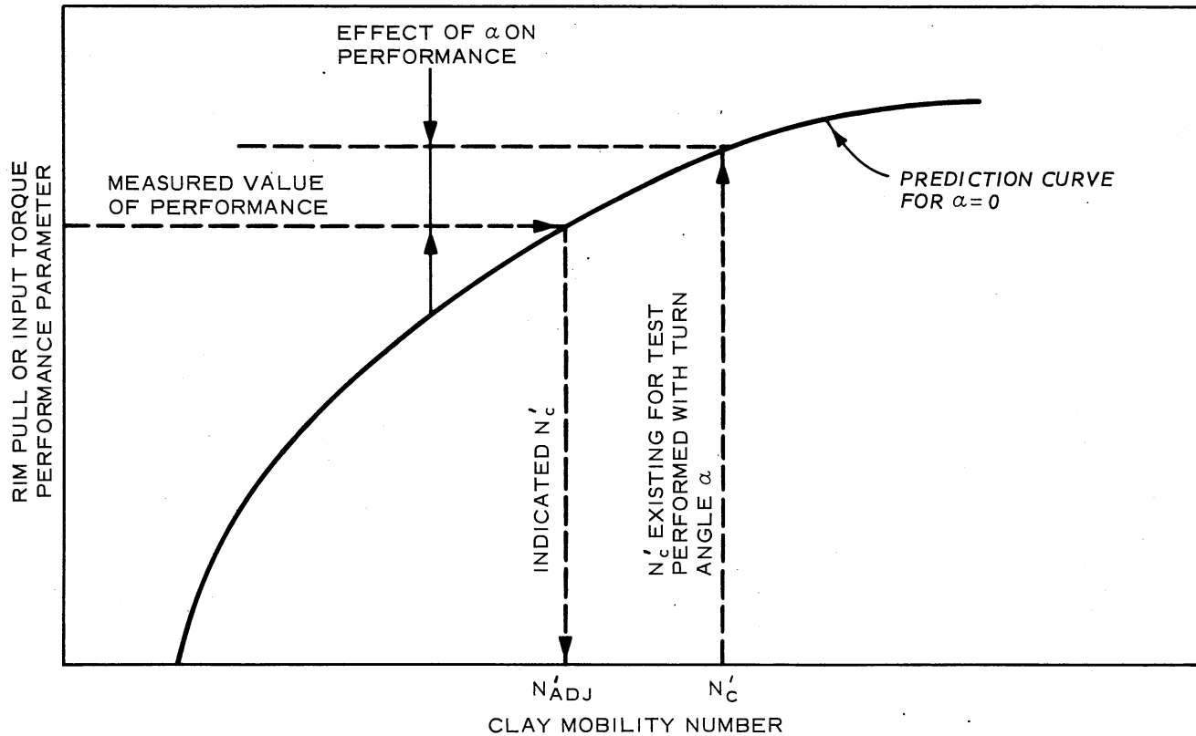
Figure 4.1. Qualitative Comparison of Clay Mobility Numbers as Determined from Test Condition at Turn Angle \alpha and as Indicated by Measured Performance Parameter.
