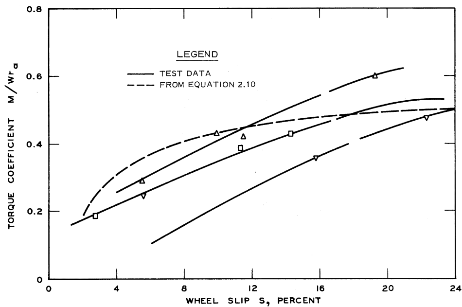
b. TORQUE COEFFICIENT
