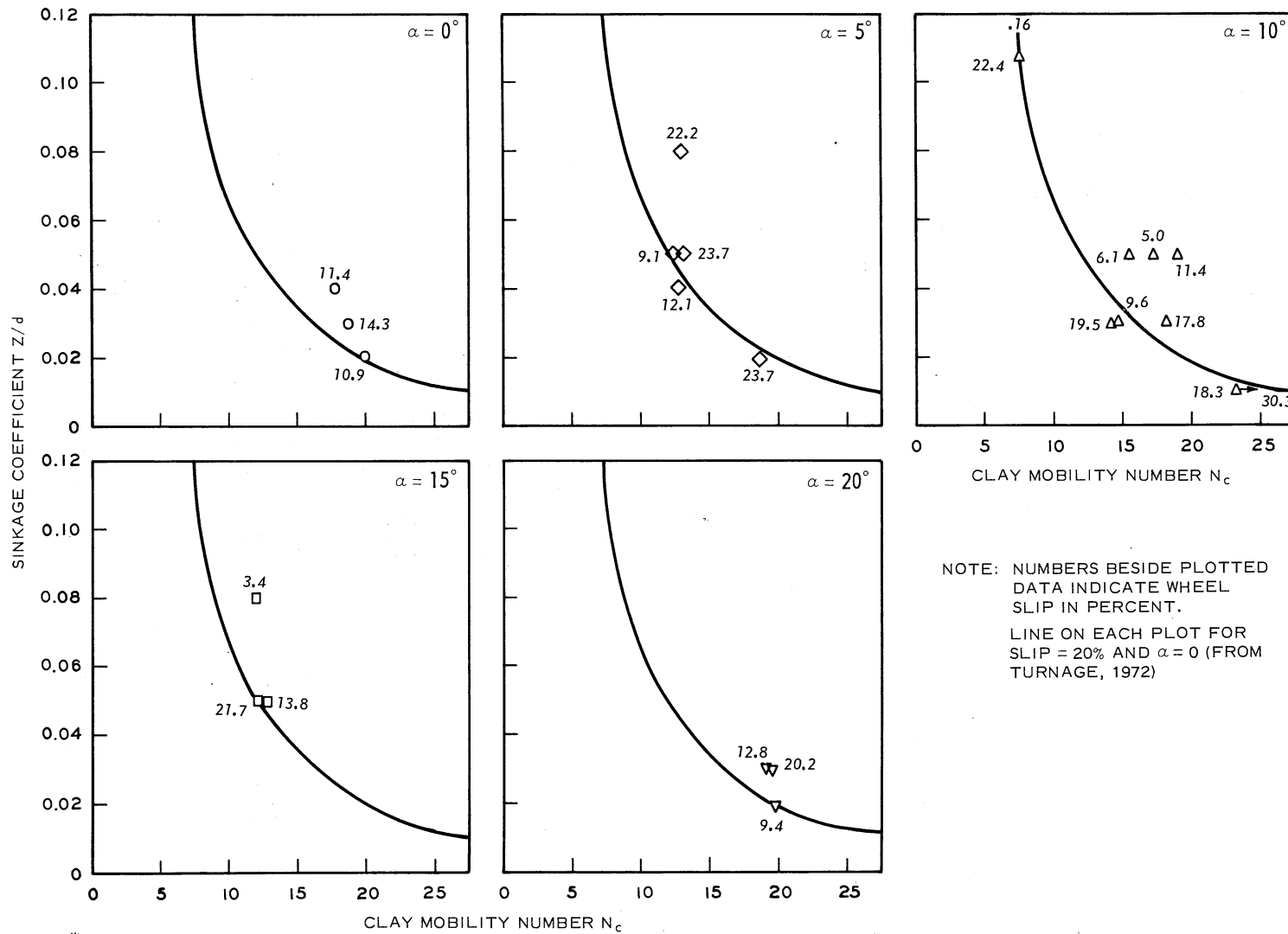
Figure 4.9. Sinkage Coefficient as Functions of Clay Mobility Number and Turn Angle.
