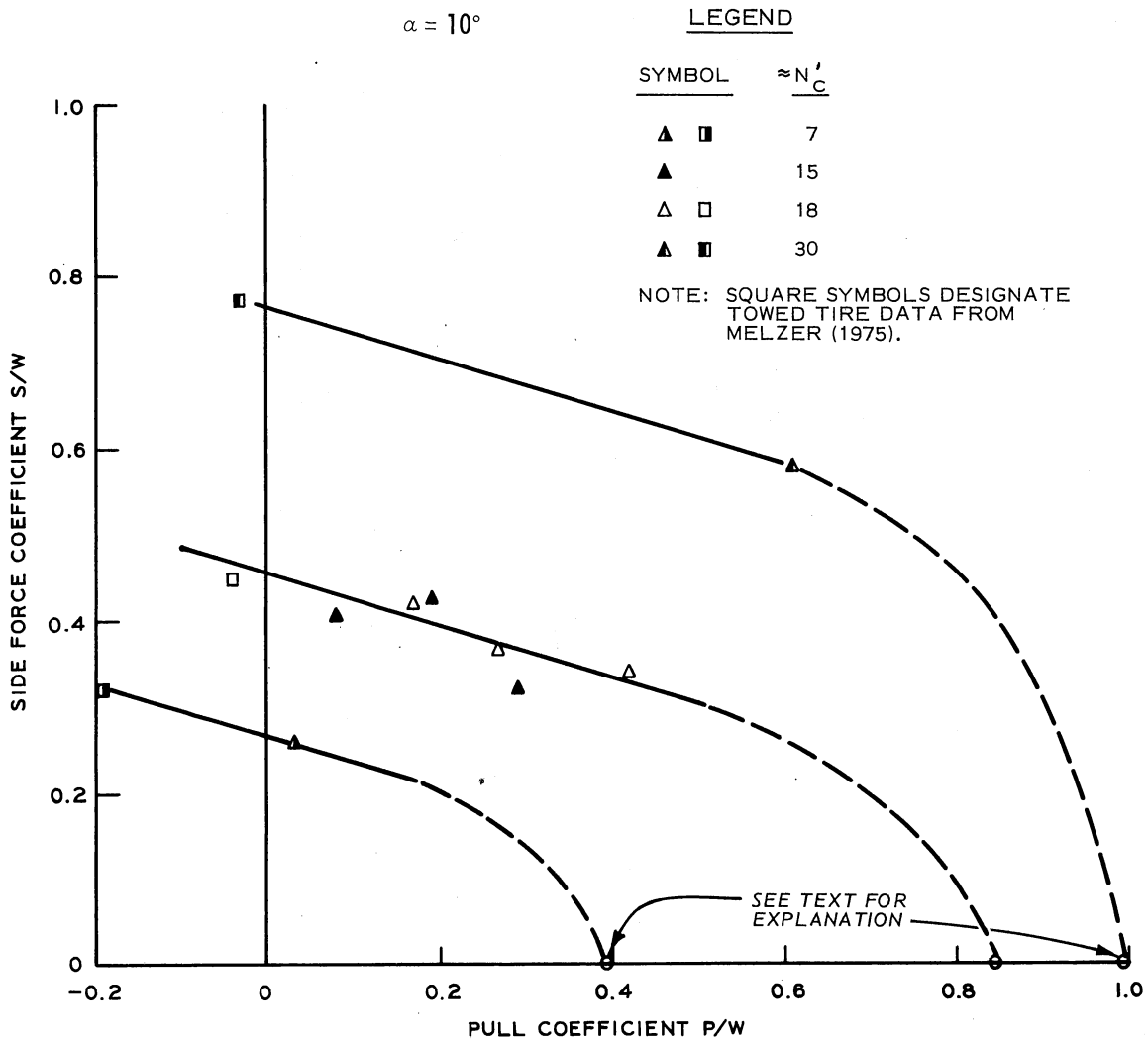
Figure 4.5. Effect of Variation in Clay Mobility Number on Side - Force Versus Pull Coefficient for 6.00-9, 4-PR Tire at 10 Degrees Turn Angle. Cone Penetration Number C = 290 kPa.
