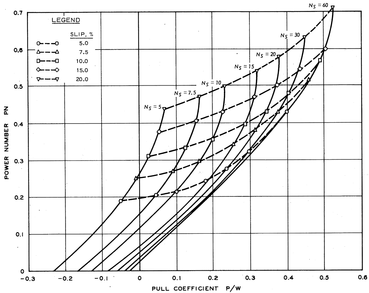
Figure 2.7. Power Number as Function of Pull Coefficient, Slip, and Sand Mobility Number (from Melzer, 1973).
