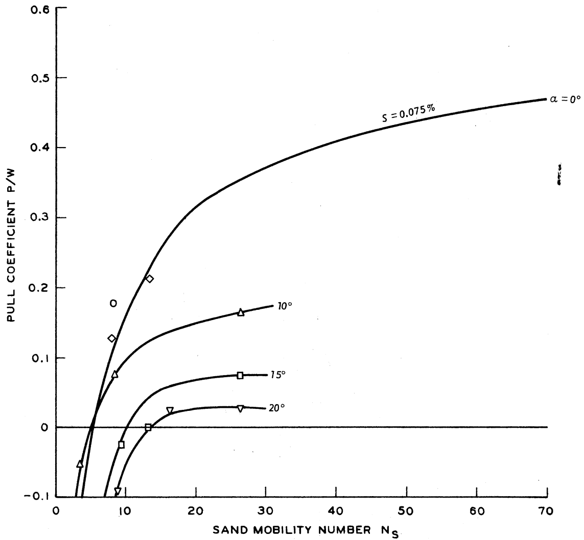
Figure 4.21. Pull Coefficient Versus Sand Mobility Number, Wheel Slip = 7.5 Percent.
