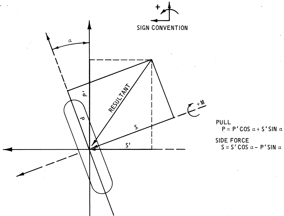
Figure A.1. Forces and moments acting on the powered turned tire (effect of trail moment neglected)
