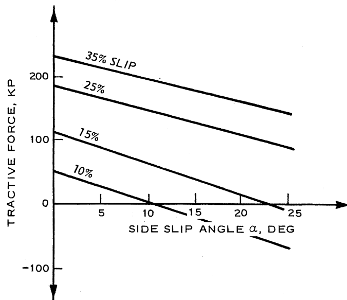
a. LINEARIZED TRACTIVE FORCE VERSUS SLIP ANGLE
