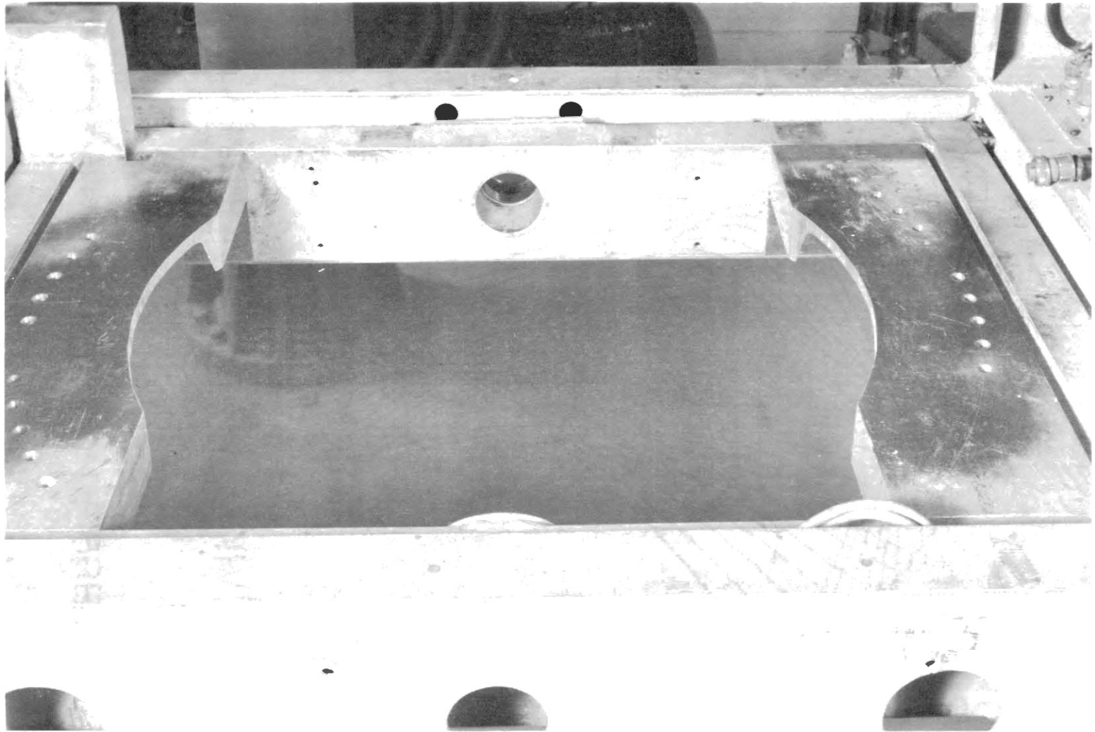
Figure 3.12. Lower Frame Assembly of Dynamometer System (Without Subframe and Wheel).
