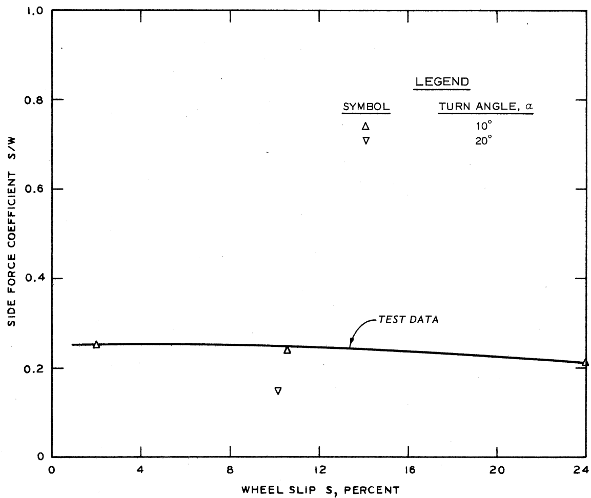
Figure 4.31. Influence of Turn Angle on Side Force Coefficient. Average Cone Penetration Resistance Gradient G = 2.0 , Tire Deflection \delta/h = 0.15 , Design Wheel Load W = 2,000 N . Desired Sand Mobility Number N_s = 3.5 .
