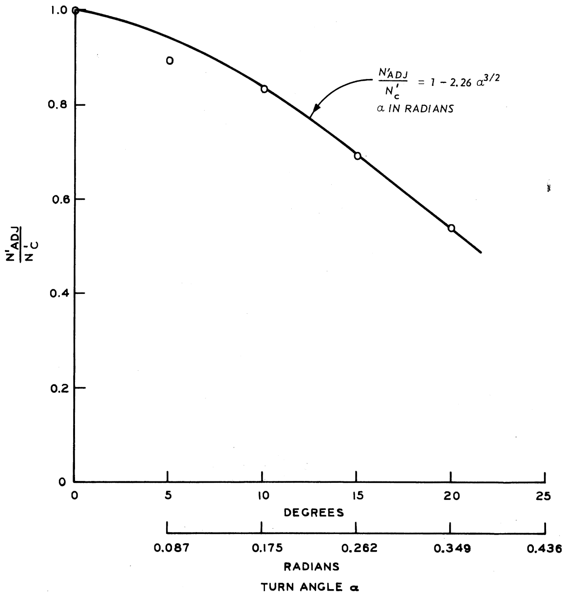
Figure 4.3. Relation between N'_{ADJ}/N'_C and Turn Angle \alpha .
