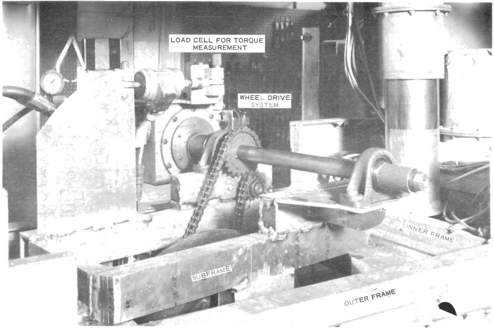
Figure 3.13. Subframe Mounted in Place and Wheel Drive System.
