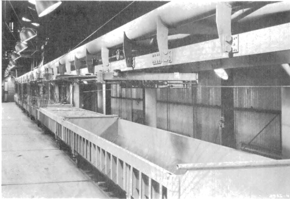
Figure 3.4. Soil Bin in Position Beneath Overhead Rail System.
