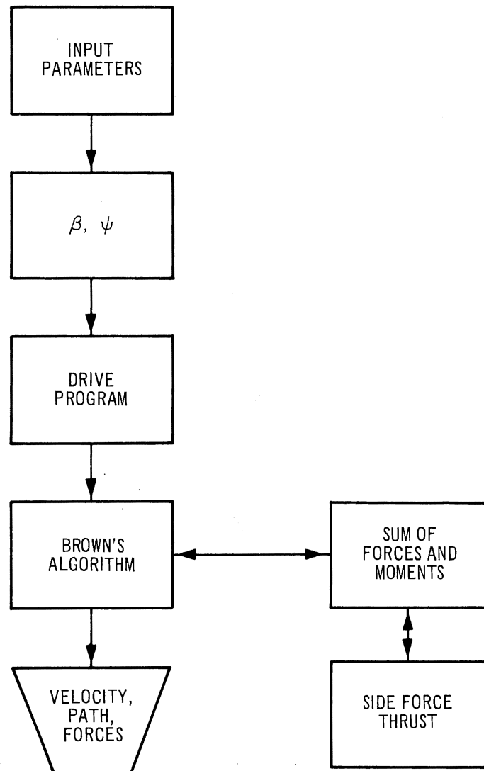
Figure 5.7. Turning Program Block Diagram
