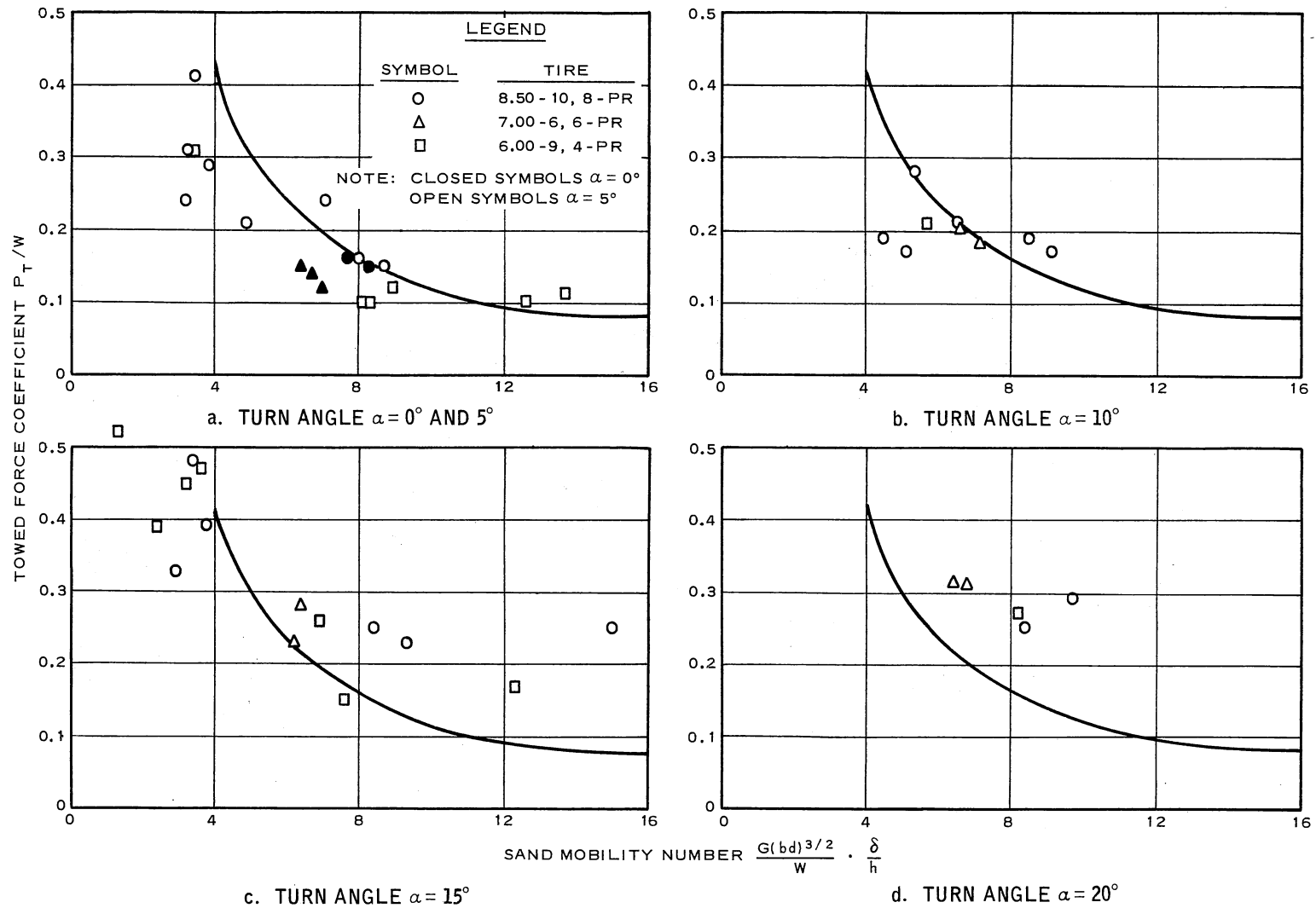
Figure 2.11. Towed Force Coefficient as a Function of Sand Mobility Number and Wheel Turn Angle (Data from Melzer, 1976).
