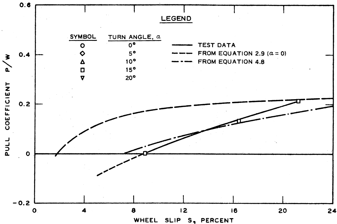
a. PULL COEFFICIENT
