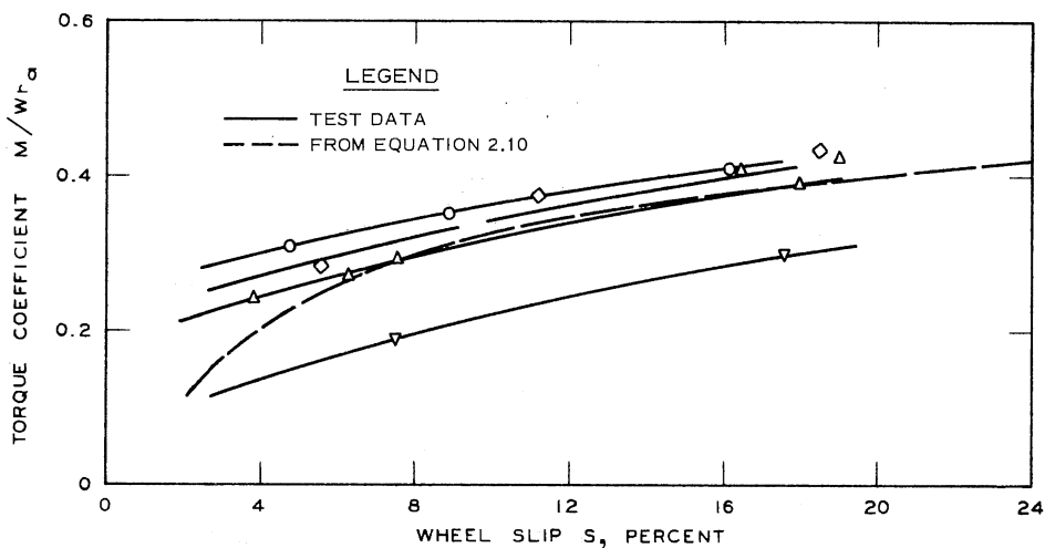
b. TORQUE COEFFICIENT
