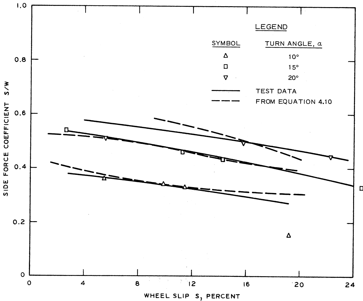
Figure 4.36. Influence of Turn Angle on Side Force Coefficient. Average Cone Penetration Resistance Gradient G = 3.2 , Tire Deflection \delta/h = 0.35 , Design Wheel Load W = 1,000 \text{ N} . Desired Sand Mobility Number N_s = 26.3 .
