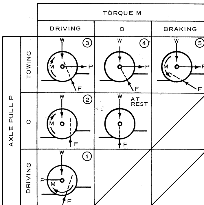
Figure 2.1. Combination of Torque M and Horizontal Axle Pull P of a Free-Bodied Wheel (after Schuring, 1966).
