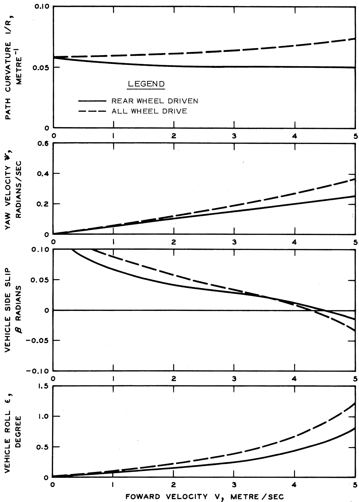
Figure 5.8. Comparison of Motion Inducted Parameters Versus Velocity for Rear Wheel and Four Wheel Driven Vehicle. Steer Angle \delta = 7 Degrees .
