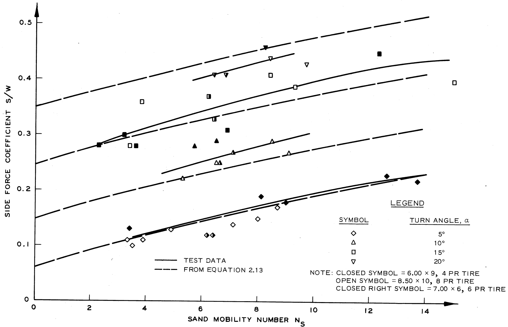
Figure 2.12. Side-Force Coefficient as a Function of Sand Mobility Number and Wheel Turn Angle (Data from Melzer, 1976).
