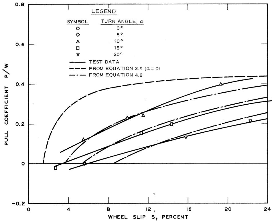
a. PULL COEFFICIENT
