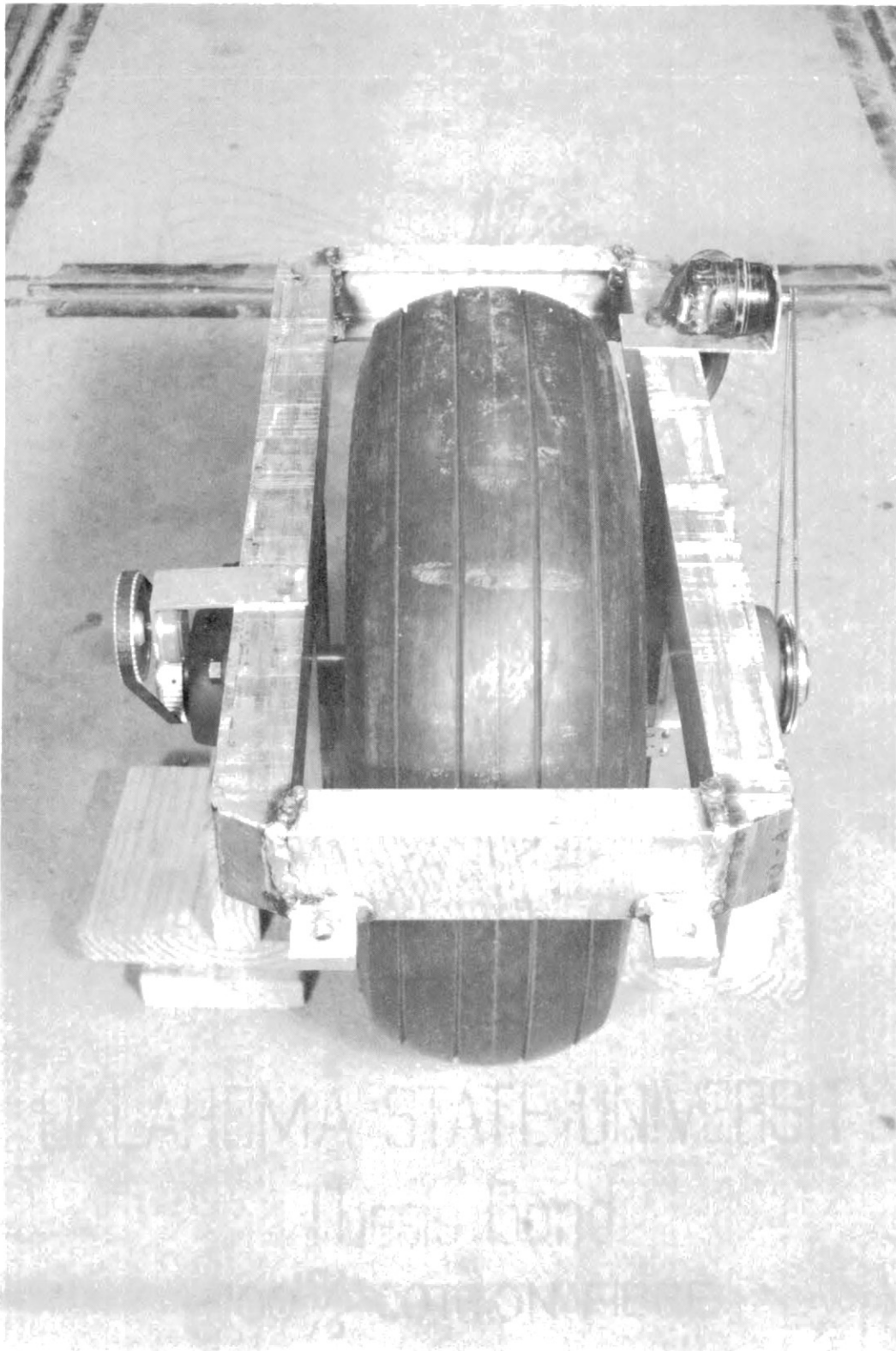
Figure 3.11. Wheel Equipped with 850-10, 8-PR Aircraft Pneumatic Tire Mounted in Subframe.
