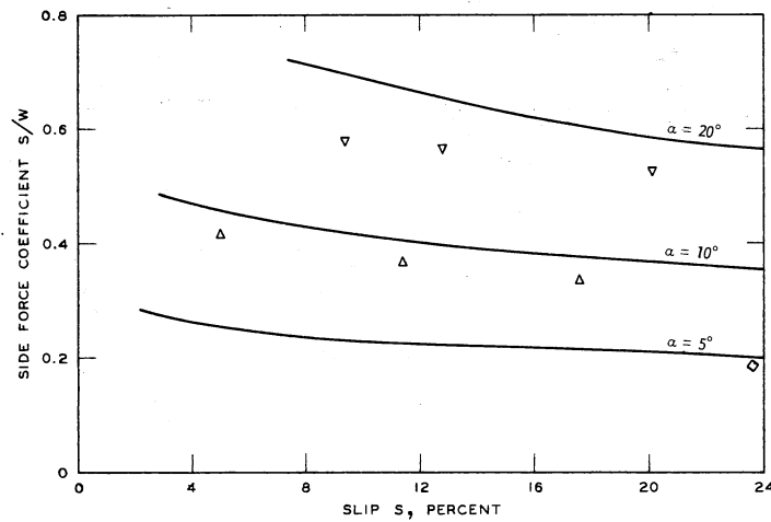
c. SIDE FORCE COEFFICIENT
