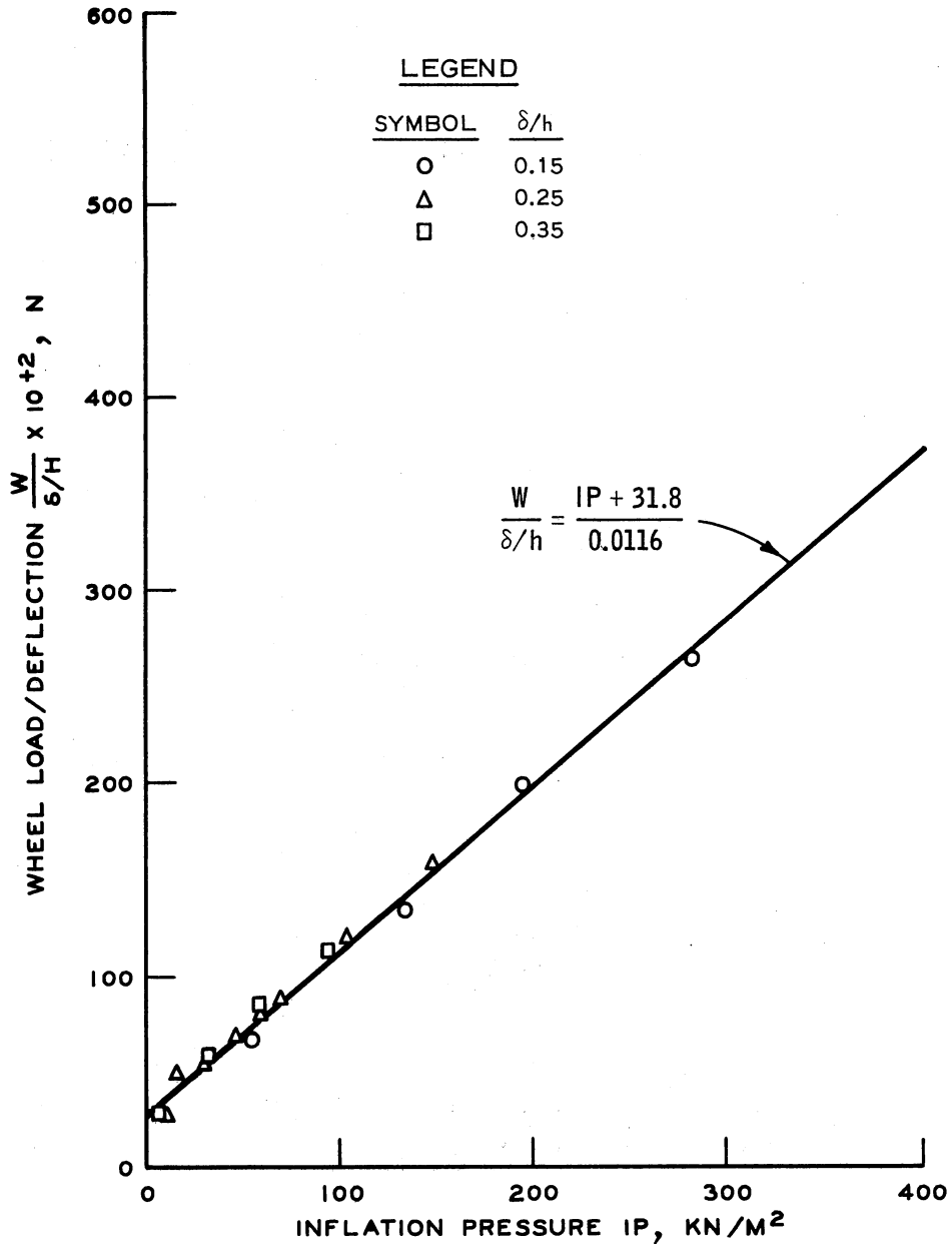
Figure 5.3. Dependency of Load/Deflection Ratio on Tire Pressure.
