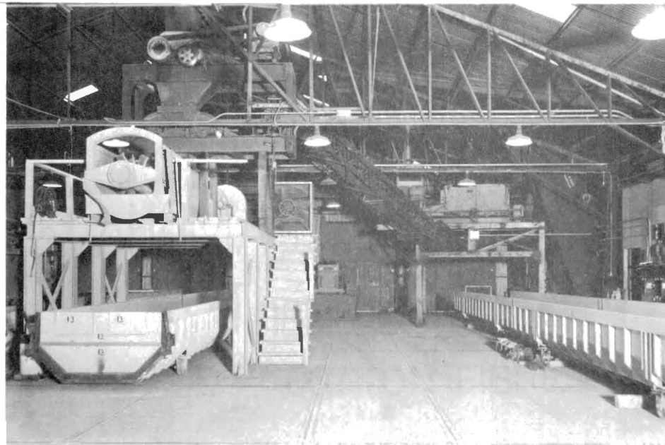
Figure 3.5. Fine-grained Soil Processing Plant.
