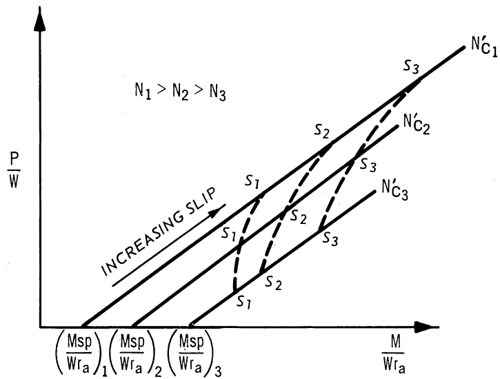
a. TIRE DEPENDENT
