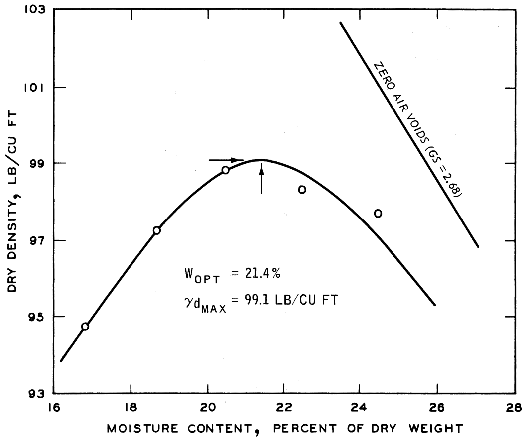
Figure 3.2. Standard Compaction Test on Vicksburg Buckshot.
