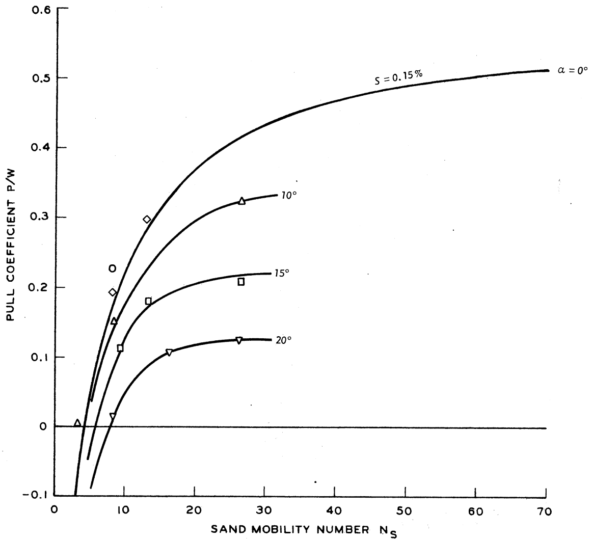
Figure 4.23. Pull coefficient Versus Sand Mobility Number, Wheel Slip = 15 Percent.
