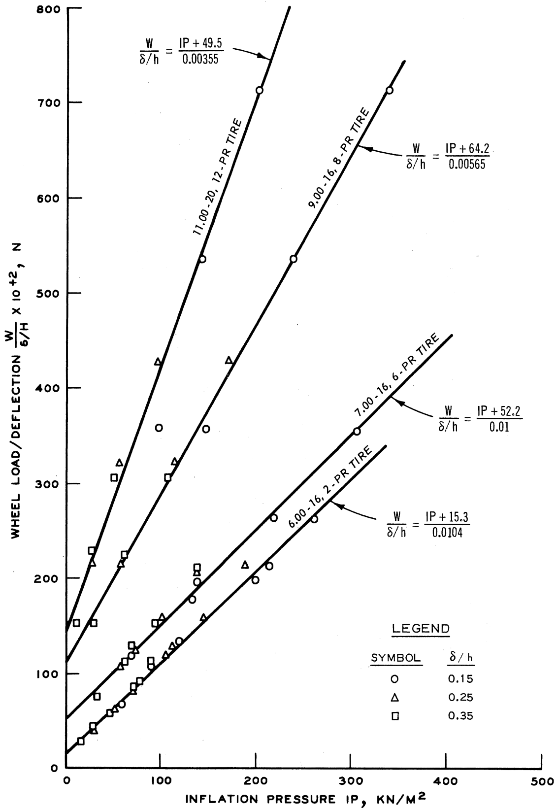
Figure 5.4. Dependency of Load/Deflection Ratio on Tire Pressure and Size.
