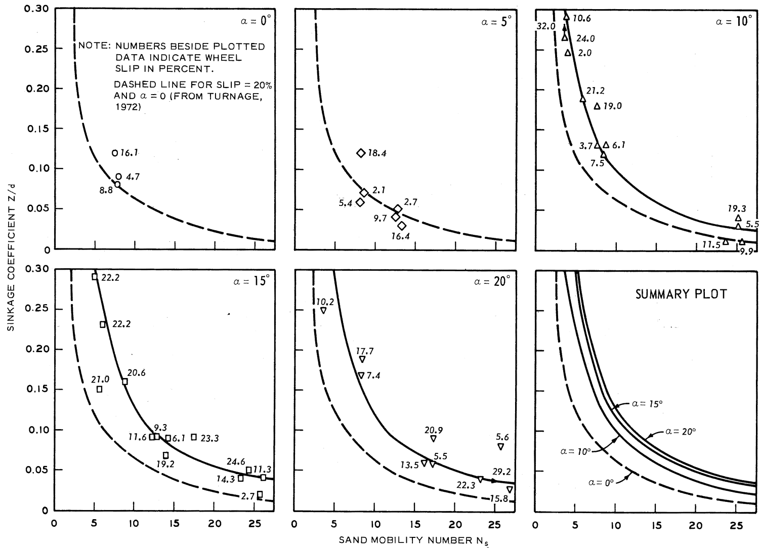
Figure 4.37. Sinkage Coefficient as Functions of Sand Mobility Number and Turn Angle.
