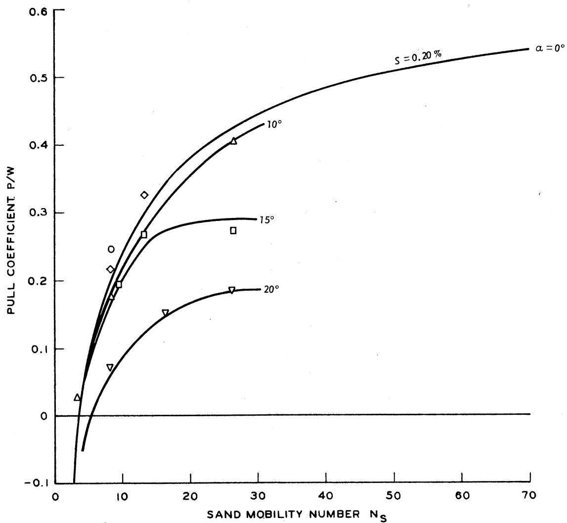
Figure 4.24. Pull Coefficient Versus Sand Mobility Number, Wheel Slip = 20 Percent.
