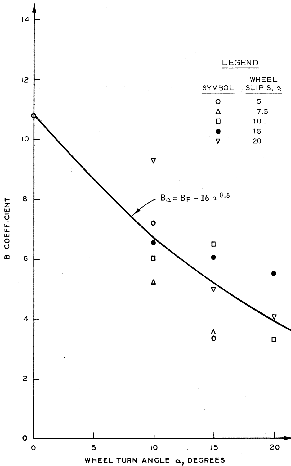
Figure 4.26. Effect of Wheel Turn Angle and Wheel Slip on B_p Coefficient.
