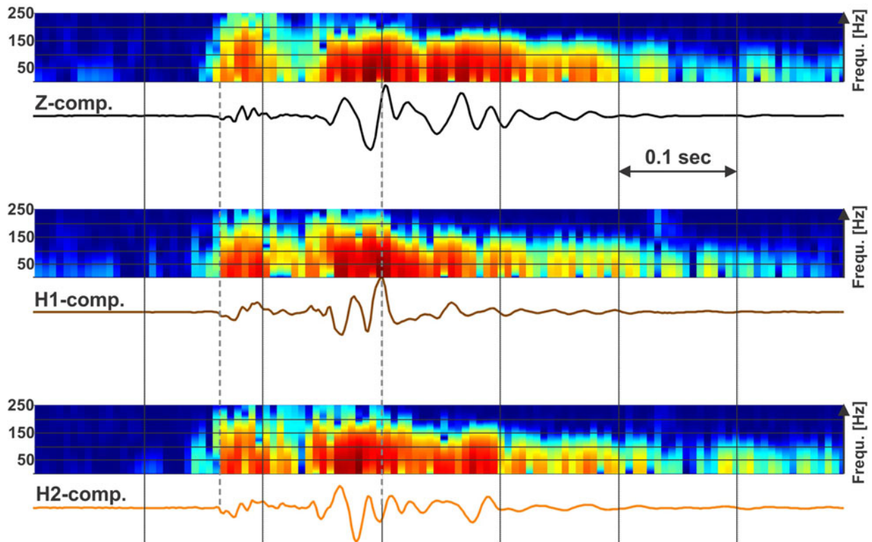
Fig. 3. A typical seismic event in the syn-discharge phase (6/1/2012) recorded on the 3C-station APO3 with spectrograms on top. H1 is oriented towards the flow direction of the glacier (ca. SE), and H2 is oriented 90° clockwise to H1. The left, dashed vertical line indicates the onset of a body wave, and the dashed line on the right is aligned with the strongest positive peak in the following Rayleigh surface-wave arrival. Note that the surface wave appears earlier on the H2 component, suggesting the superposition of Love waves.
