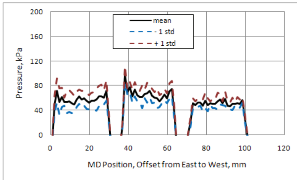
Figure 8 – Nip Pressure vs MD Position, Dual Durometer Symmetrical Roller Pair, 1620 N/m Loading
