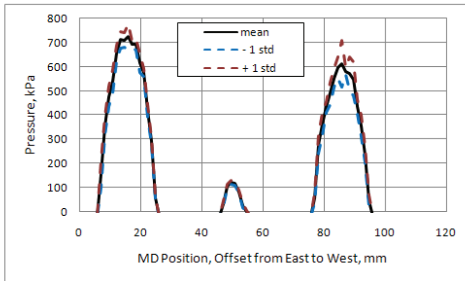
Figure 6 – Nip Pressure vs MD Position, Single Durometer (2) Symmetrical Roller Pair, 1620 N/m Loading
