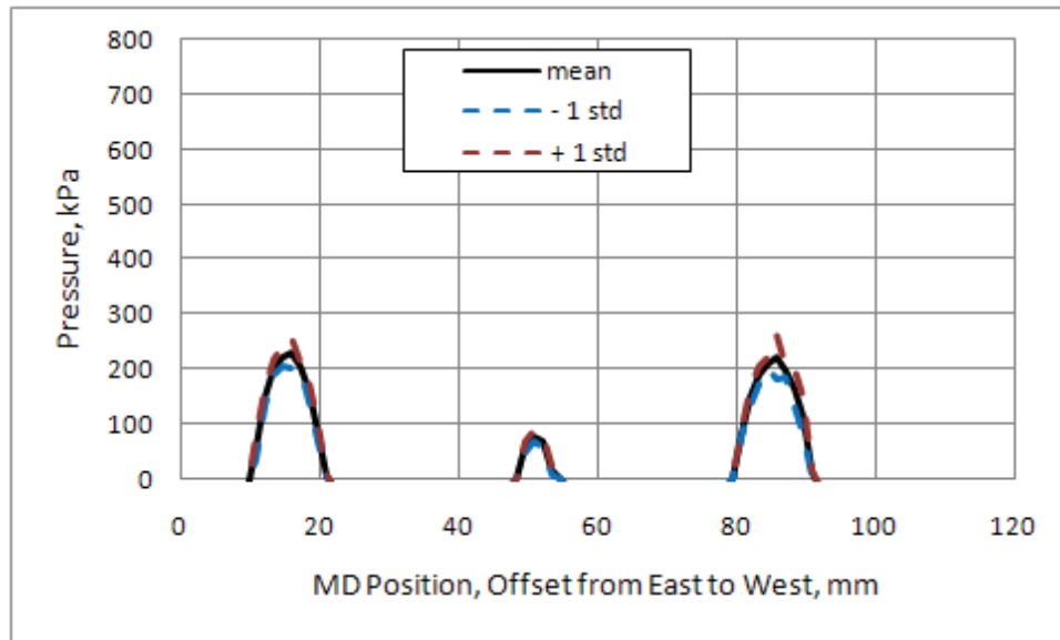
Figure 7 – Nip Pressure vs MD Position, Single Durometer (2) Symmetrical Roller Pair, 540 N/m Loading
