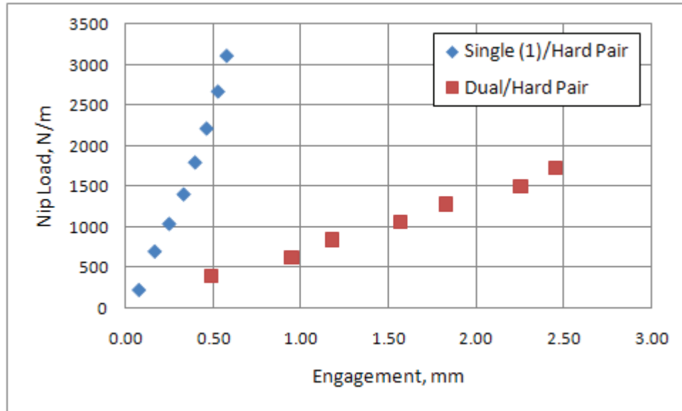
Figure 3 – Nip Load vs Engagement, Asymmetrical Nip Roller Pair
