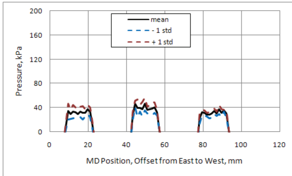
Figure 9 – Nip Pressure vs MD Position, Dual Durometer Symmetrical Roller Pair, 540 N/m Loading
