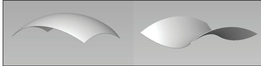
Elliptic surface
