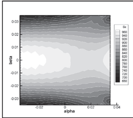
Figure 10 – MD stress Axes in radians, stress in psi
