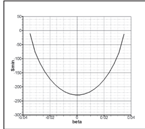
Figure 13 – Principal minimum stress at downstream roller in psi
