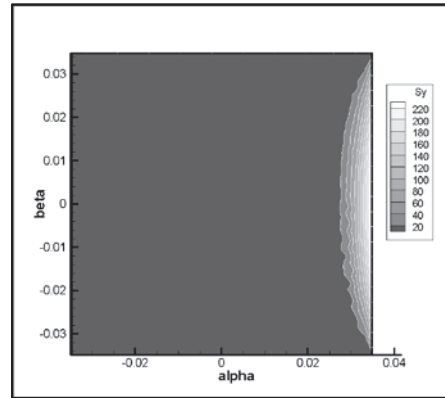
Figure 7 – CD stress, elliptic web Axes in radians, stress in psi
