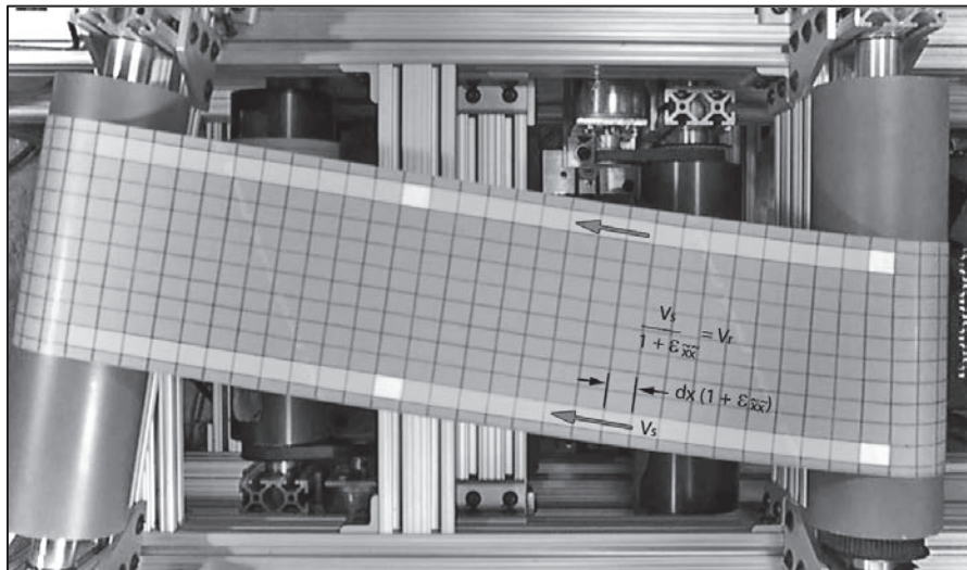
Figure 3 – Qualitative Demonstration of the Velocity-Strain equation.
