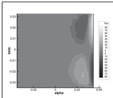
Figure 8 – Shear stress, elliptic web Axes in radians, stress in psi
