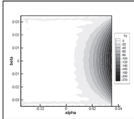
Figure 11 – CD stress Axes in radians, stress in psi
