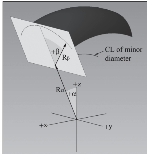
Figure 5 – A Section of a Torus
