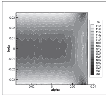
Figure 6 – MD stress, elliptic web Axes in radians, stress in psi
