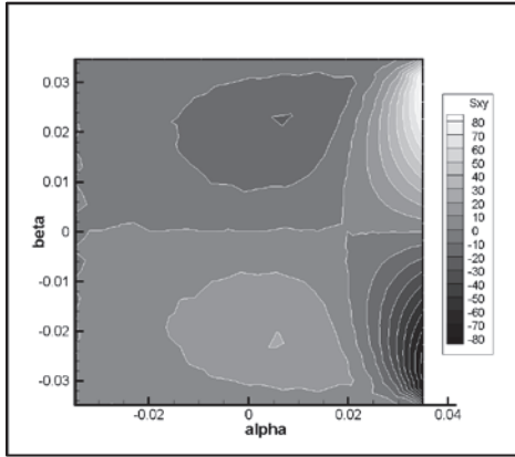
Figure 12 – Shear stress Axes in radians, stress in psi
