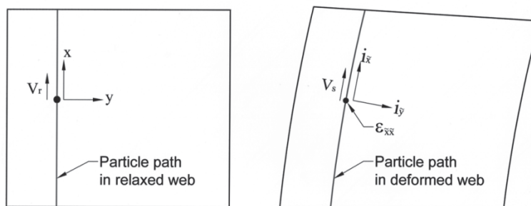
Figure 2 – Geometric relationships in the Velocity-Strain equation
