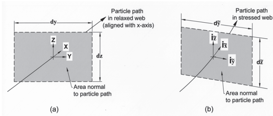
Figure 1 – Mapping mass flow in the relaxed web to mass flow in a stressed web.
