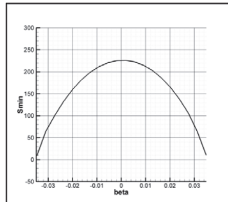
Figure 9 – Principal minimum stress at downstream roller in psi
