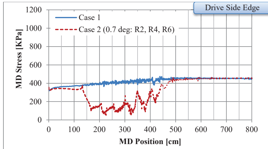
Figure 6 – Comparison of MD stresses in the web along its length at different CD locations between Case (1) and Case (2)
