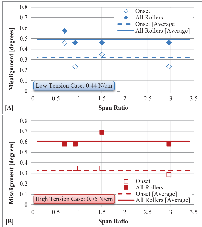
Figure 15 – Misalignment needed to cause wrinkles within accumulator at different span heights and tensions
