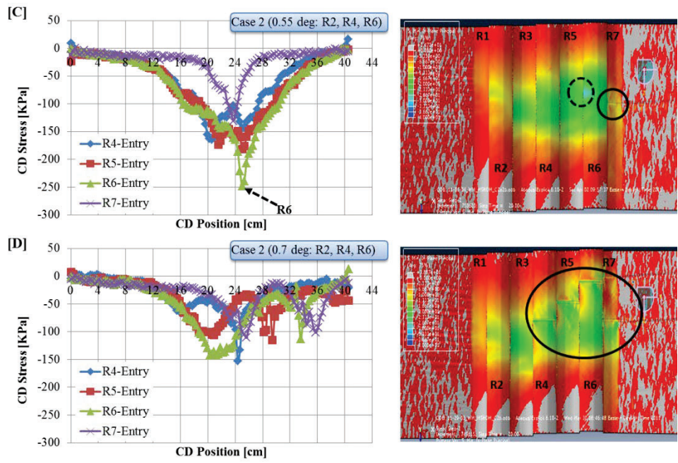
Figure 7 – CD stresses in the web at the entry of rollers R4-R7 and contours of CD stresses in the web for rollers R1-R7.
