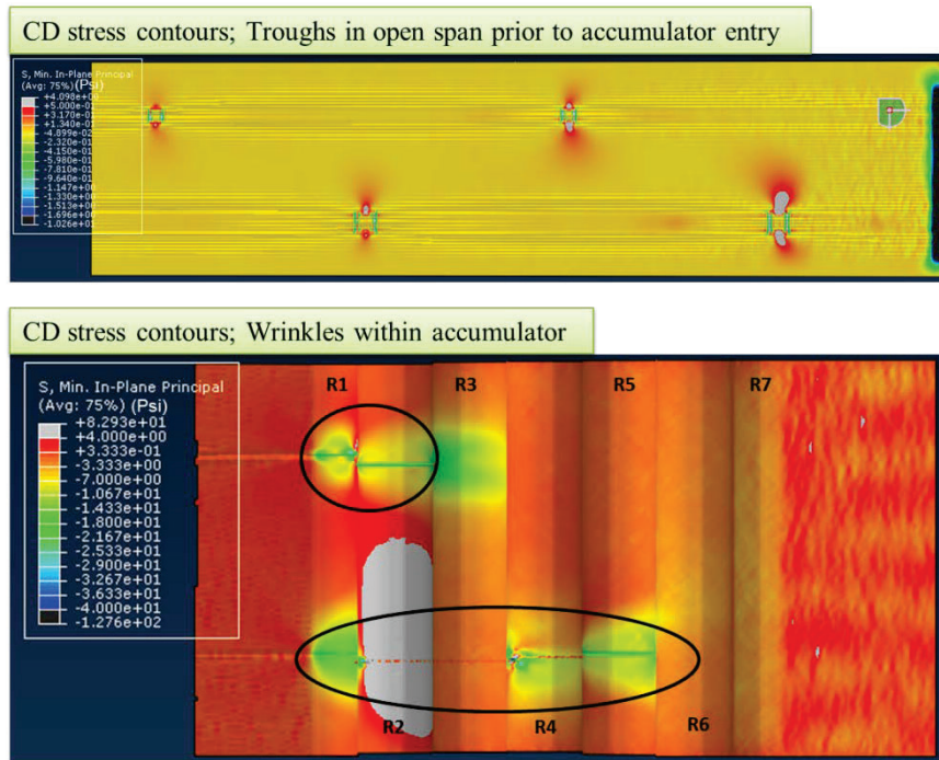
Circles in the figure indicate the presence of a wrinkle on one or more rollers
