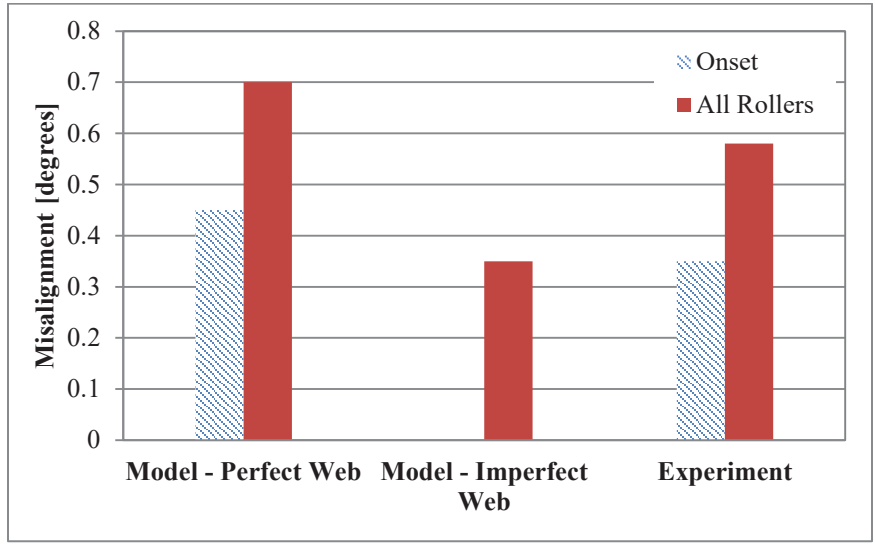
Figure 17 – Misalignment needed to cause wrinkles within accumulator at different span heights and tensions
