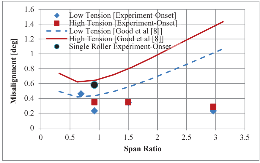
Figure 16 – Misalignment needed to cause wrinkles within accumulator at different span heights and tensions
