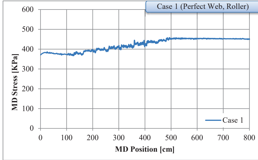
Figure 4 – MD stresses in the web along its length at different CD locations for Case (1)
