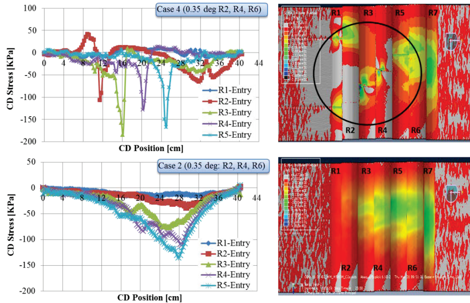
Figure 13 – CD stresses due to web imperfections and misaligned rollers within accumulator.
