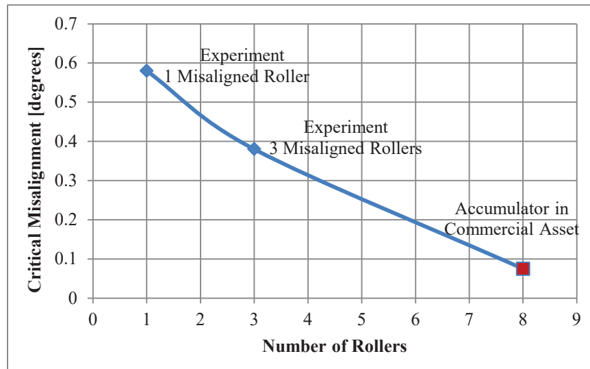
Figure 18 – Critical misalignment needed to cause wrinkles within accumulator for different number of rollers
