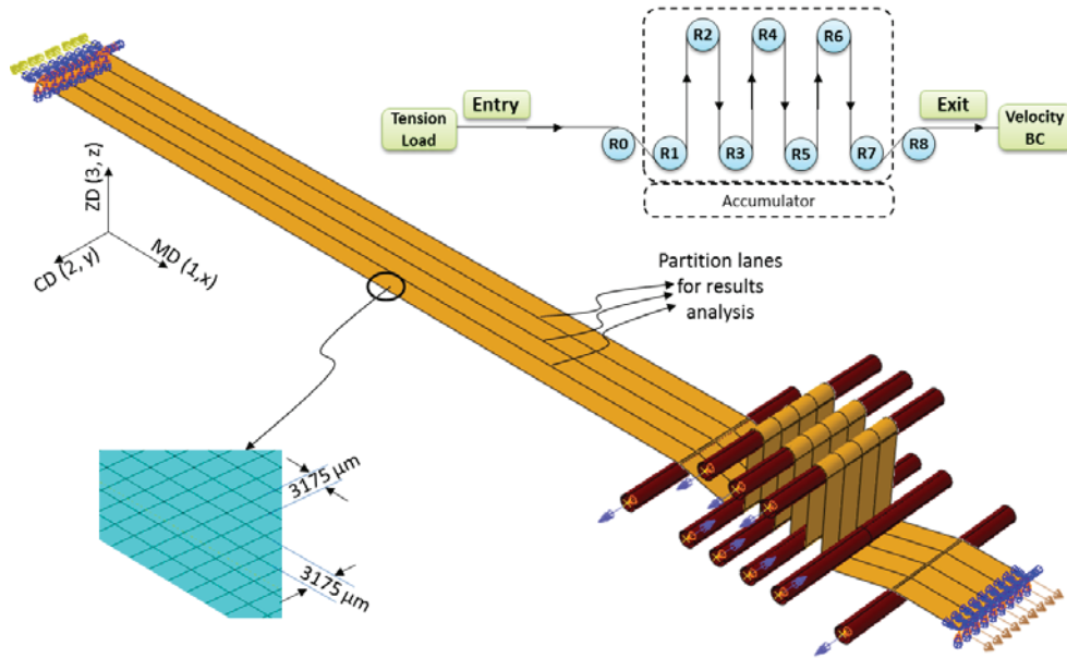
Figure 2 – Schematic representation of the FE model set up
