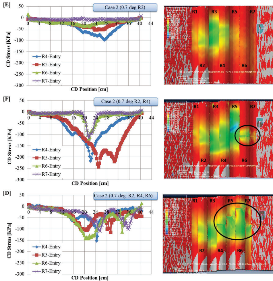
Figure 8 – Comparison of CD stresses for cases wherein one, two or all three top carriage rollers are misaligned.
