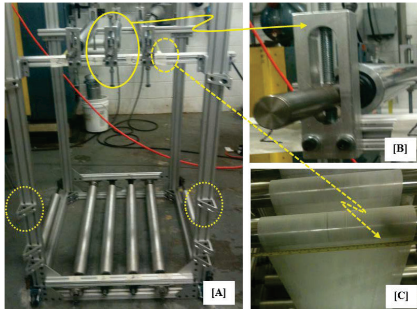
Figure 14 – Accumulator Module
