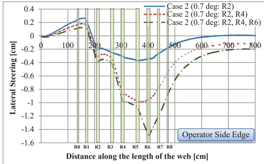
Figure 10 – Comparison of lateral steering for cases wherein one, two or all three top carriage rollers are misaligned.
