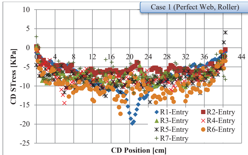
Figure 5 – CD stress in the web at the entry of all rollers in the accumulator in Case (1)
