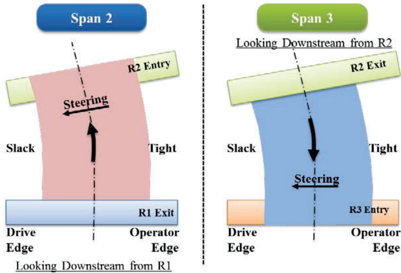
Figure 9 – Schematic of web behavior in spans 2 and 3.
