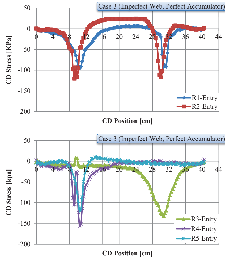
Figure 12 – CD stresses due to web imperfections at the entry of rollers R1-R5.
