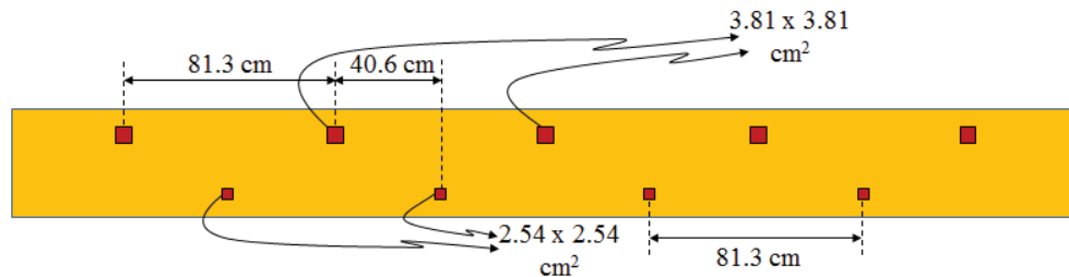
Figure 3 – Schematic of imperfections in the web in the entering span
