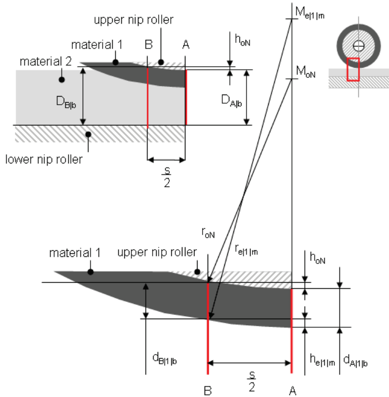
Figure 5 – Calculation of the substituting radii using the formula for a segment of a circle. Shown are the heights of the segment of a circle for the upper nip roller, for the substituting cycle and the compressed thicknesses of material on position A and B.
