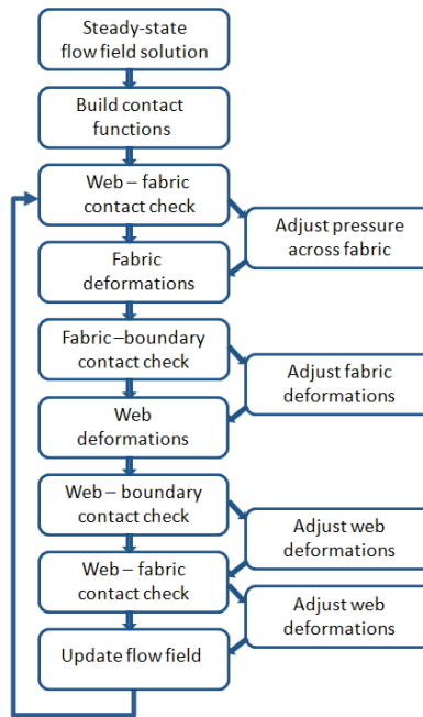
Figure 4 – Schematic representation of numerical resolution of the FSI model
