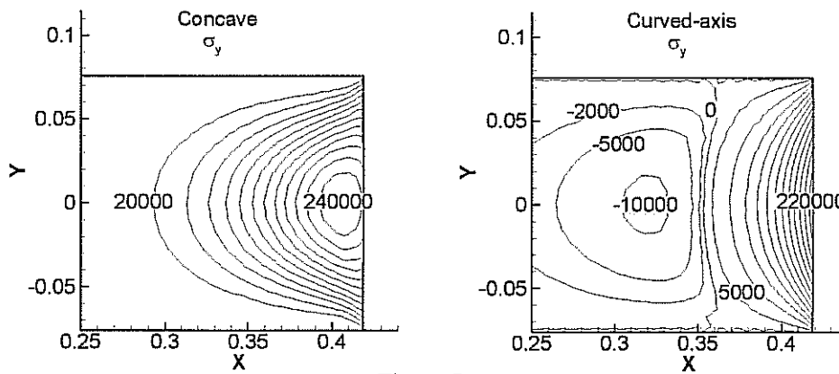
Figure 5 Comparison of cross web stress (Pa) for concave and curved-axis rollers
