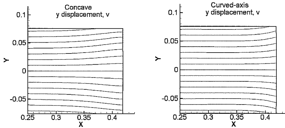
Figure 4 Comparison of y displacement, v , for concave and curved-axis rollers
