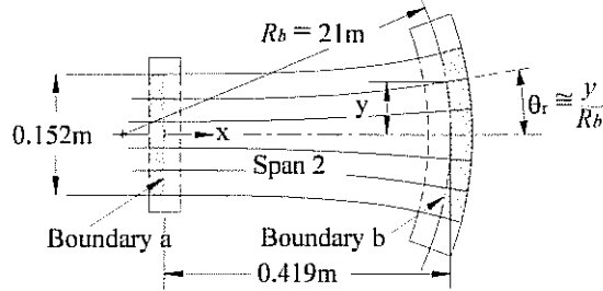
Figure 2 Curved-axis roller
