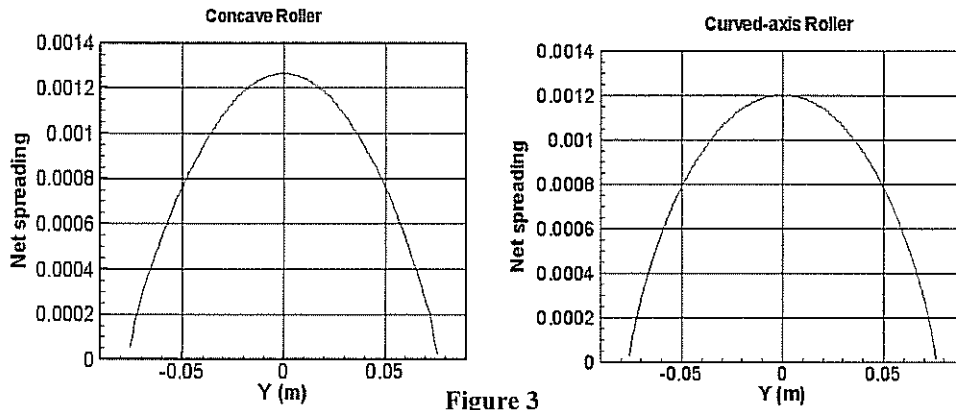
Figure 3 Comparison of spreading by Concave and Curved-axis rollers
