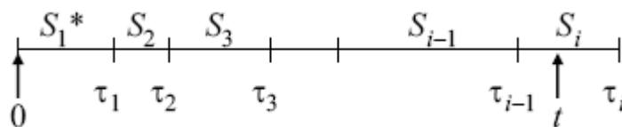
Figure 3. 2: Poisson Process
