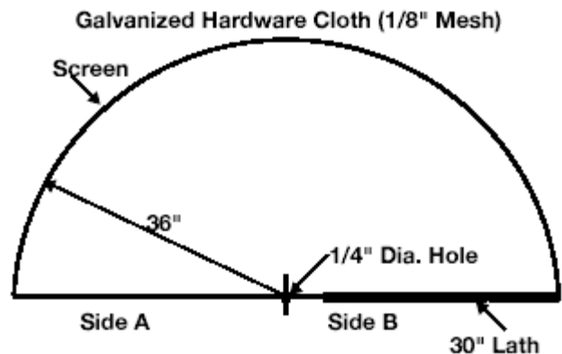
Figure 2. Schematic diagram of the wire cone emergence trap.
