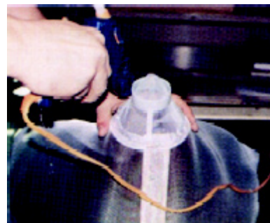
Figure 9G. Seal trap top assembly into place using hot glue.
