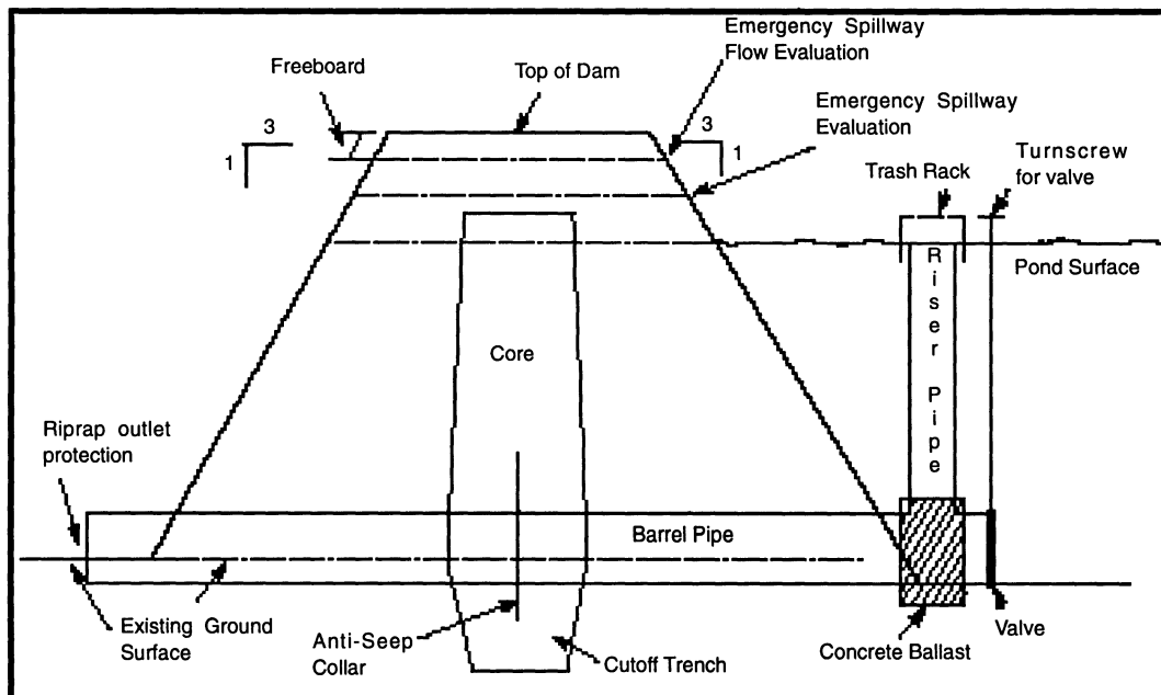
Figure 5. Typical cross-section of dam at the pipe.
