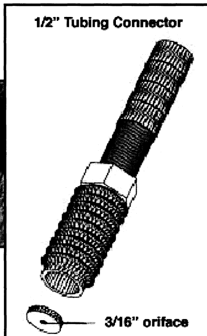
Figure 7. PVC tubing connectors with construction orifice.
