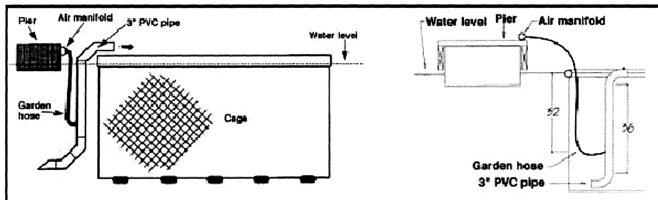
Figure 5. Cage along a pier with air-lifts mounted over the top of the case (left) and inside the cage (right).
