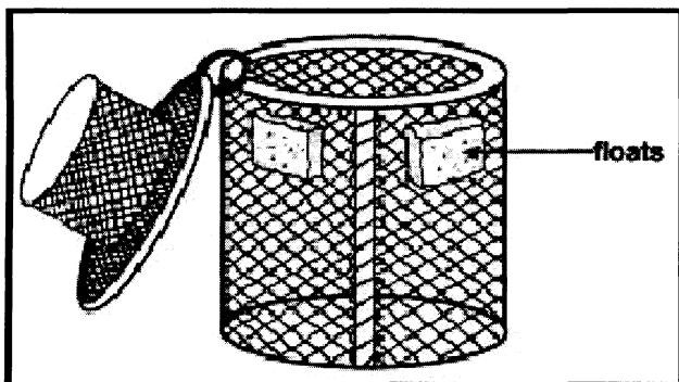
Figure 2. The 4' x 4' cylindrical cage design.
