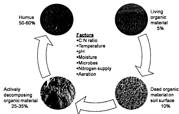
Figure 1. Organic components of the soil.
