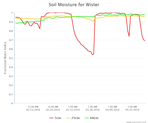
Figure 2. FWI Graphs for three soil depths at Mesonet Site: Hollis, Kingfisher and Wister.
