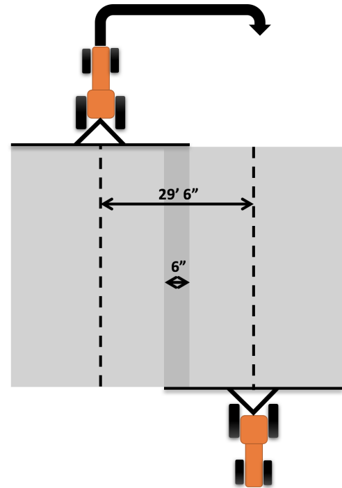
Figure 1. An example of pass-to-pass accuracy measurement for a standard 30-foot machine swath. Pass-to-pass error is 6 inches.
