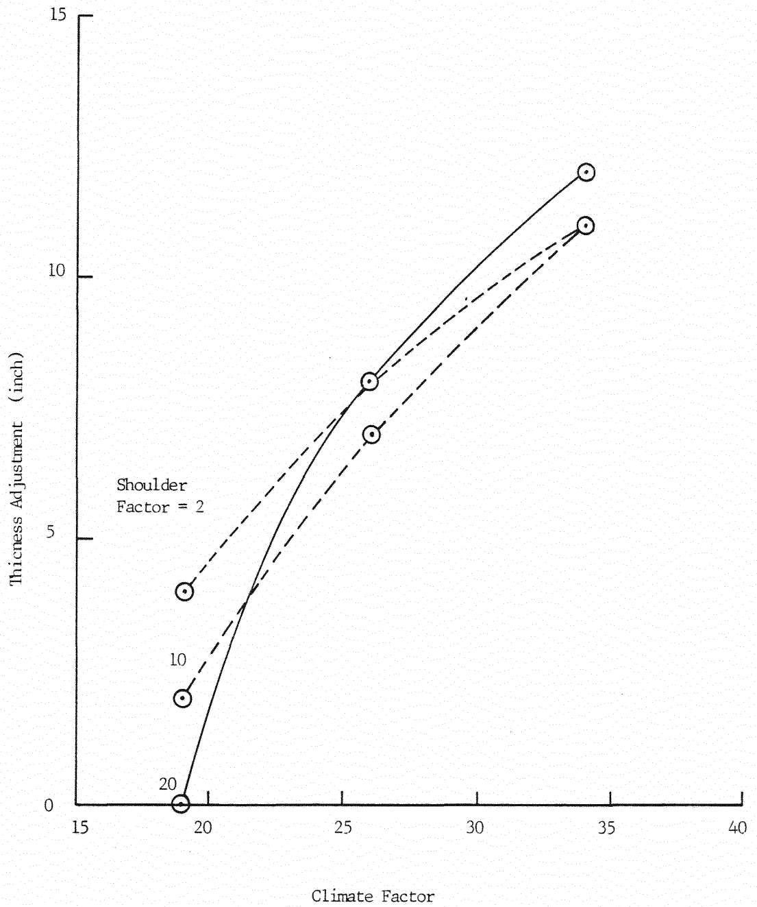
Figure 16. Sensitivity of thickness adjustment on climate factor for a traffic factor = 300.
