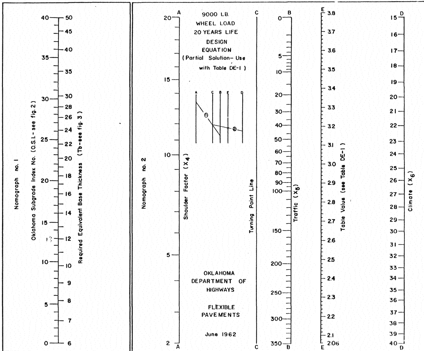
Figure 14. Nomograph for EBT adjustment by different factors.
