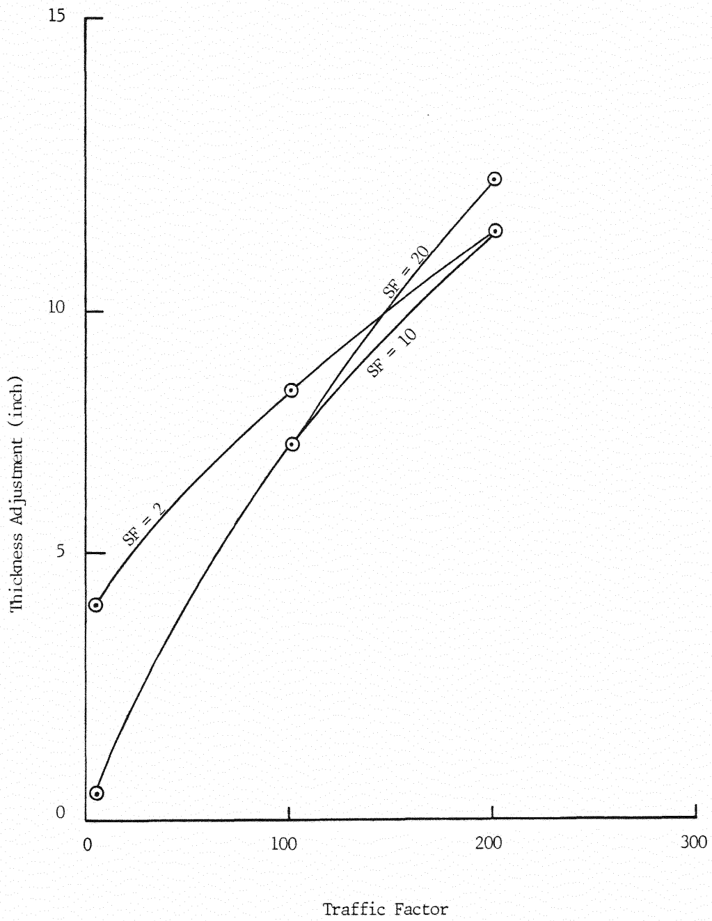
Figure 17. Sensitivity of thickness adjustment on traffic factor for a climate factor = 34.
