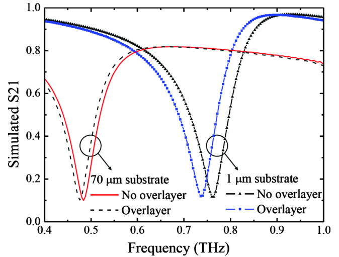
FIG. 3. (Color online) Effect of substrate thickness on sensitivity: shift in \omega upon addition of 1 \mu\text{m} overlayer of \epsilon = 2 onto SRRs on silicon substrates 1 \mu\text{m} thick and 70 \mu\text{m} thick.
