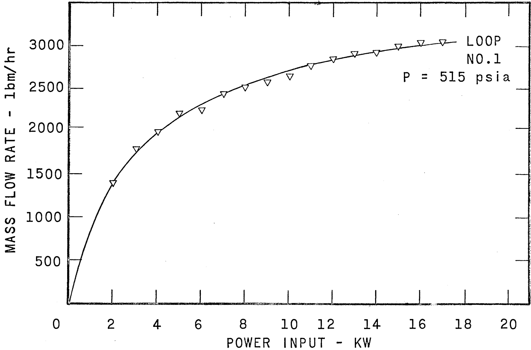
Fig. 16 Mass Flow Rate as a Function of Power Input
