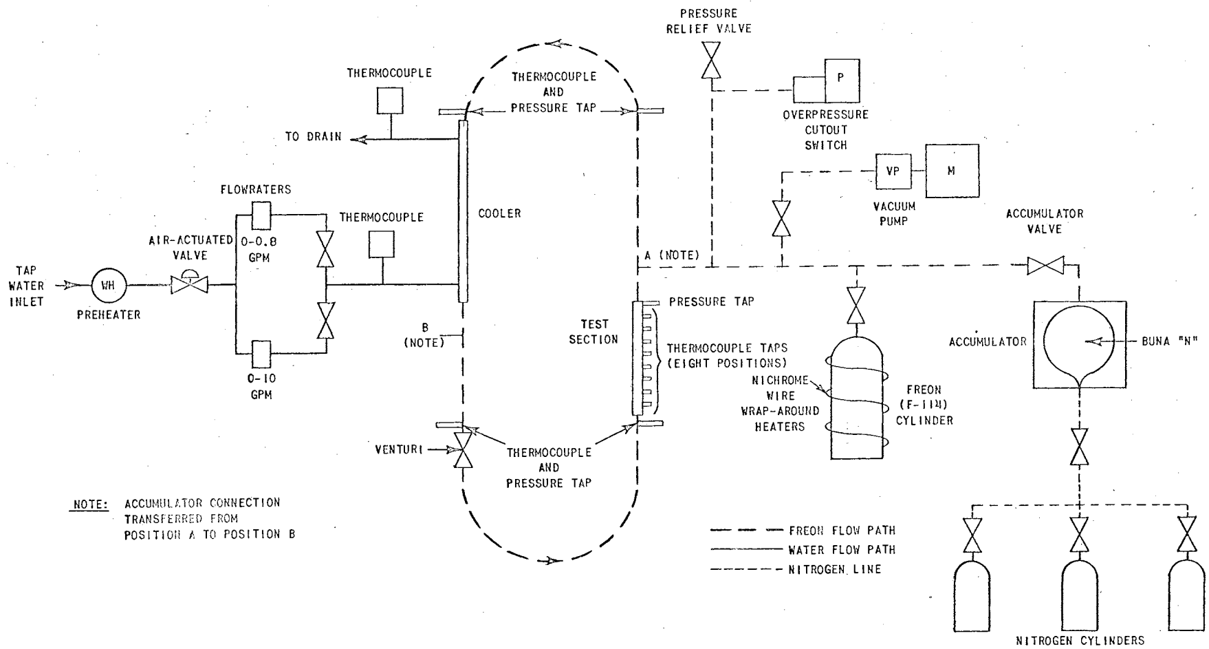
Fig. 5 Schematic Diagram of Test Apparatus
