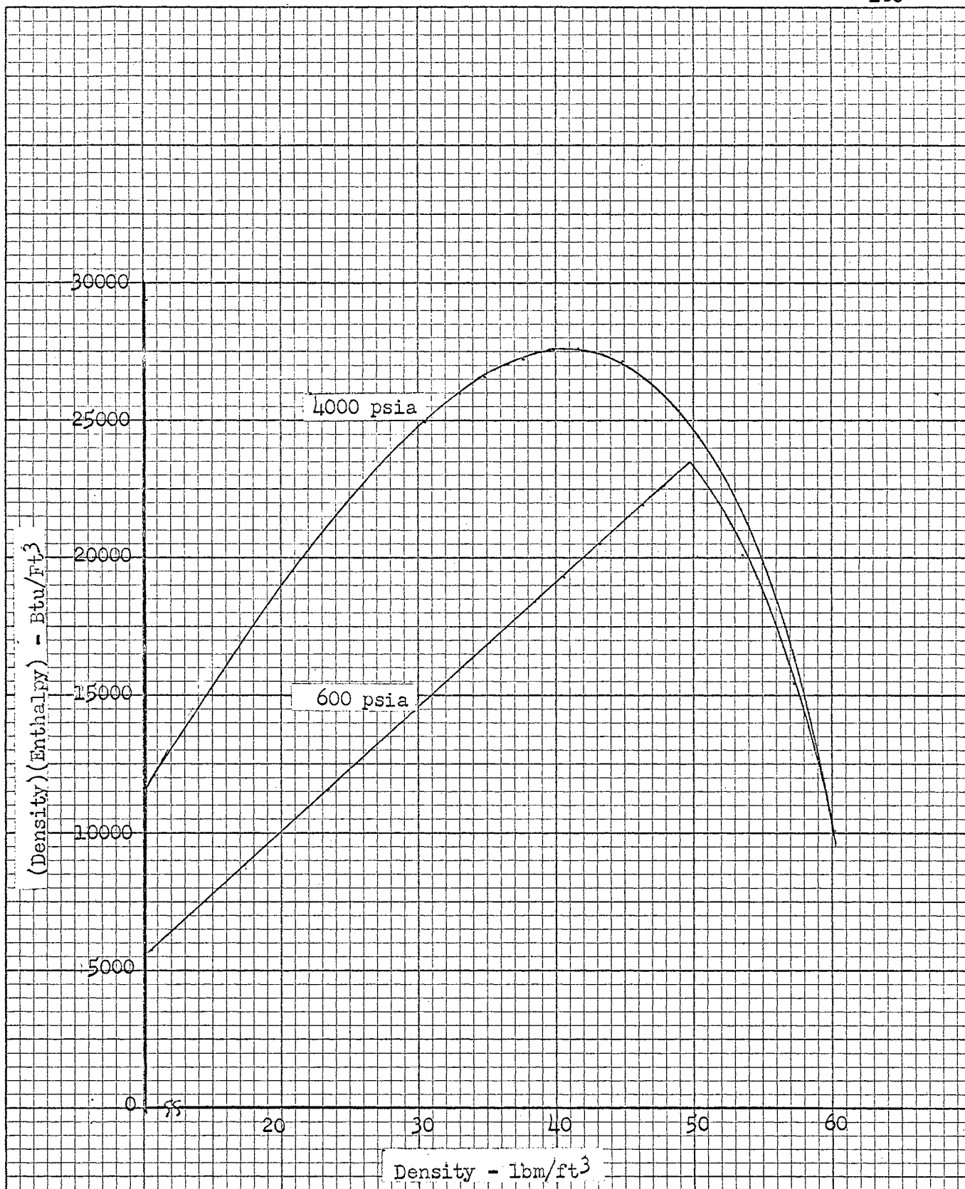
Fig. 40. The Variation of the Density-enthalpy Product with Density along Isobars for Water
