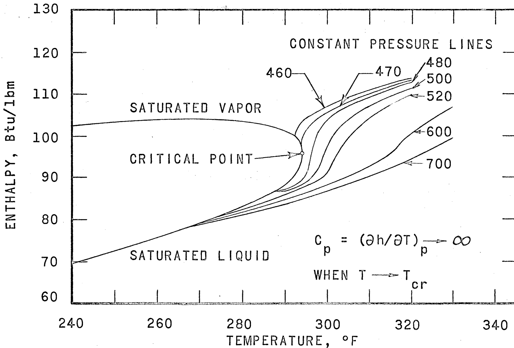
Fig. 33. Enthalpy-Temperature Relationship for F-114 in the Critical Region
