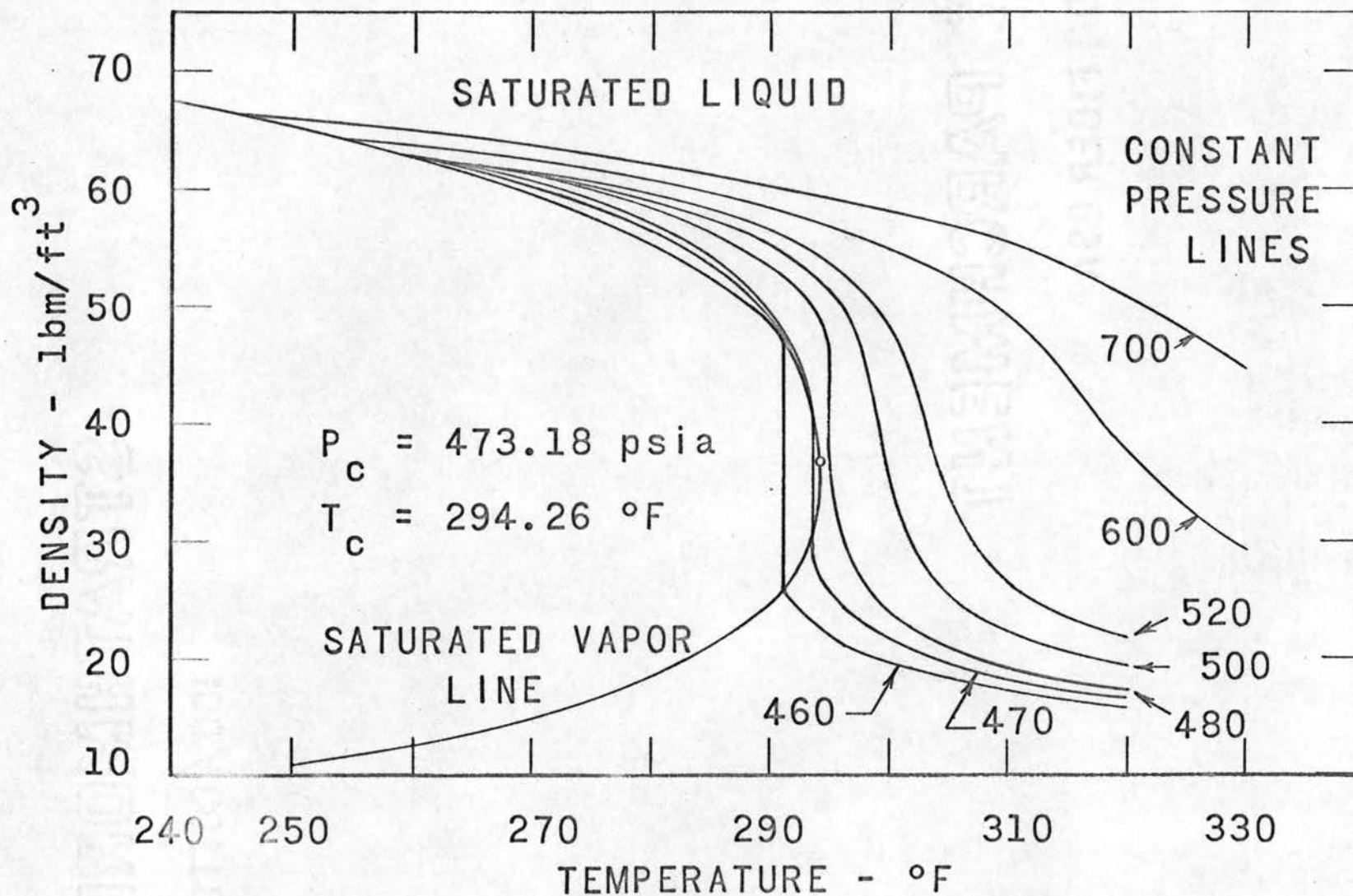
Fig. 34. Density-Temperature Relationship for F-114 in the Critical Region
