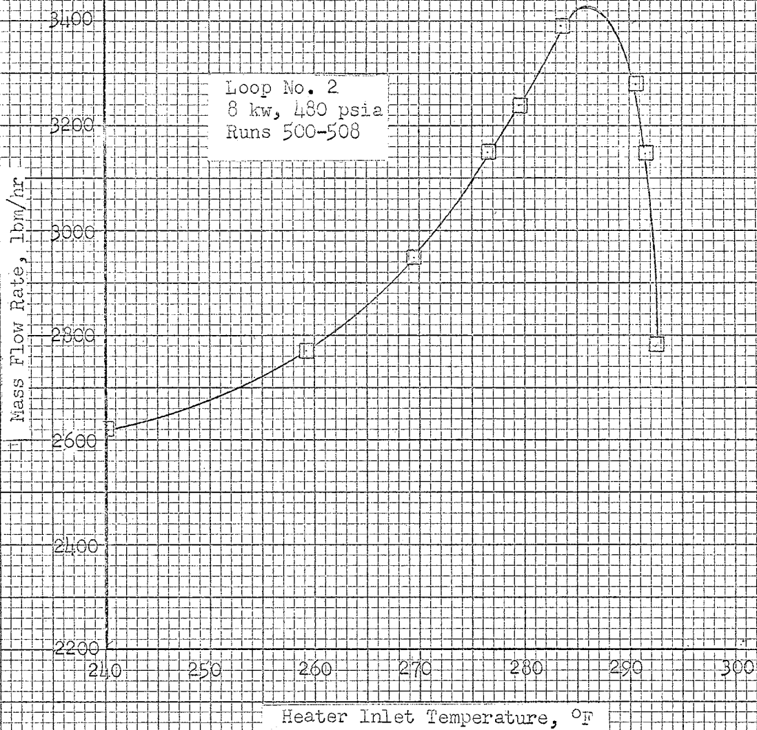
Fig. 15. Effect of Inlet Temperature on Flow Rate
