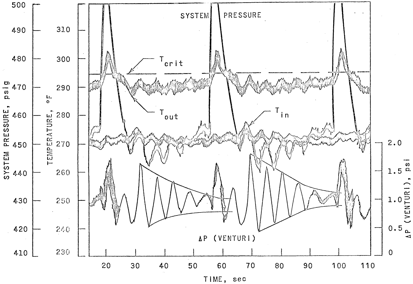
Fig. 23 Operation in the Two-Phase Region, Loop No. 1, 6 kw, Oct. 3, 1962
