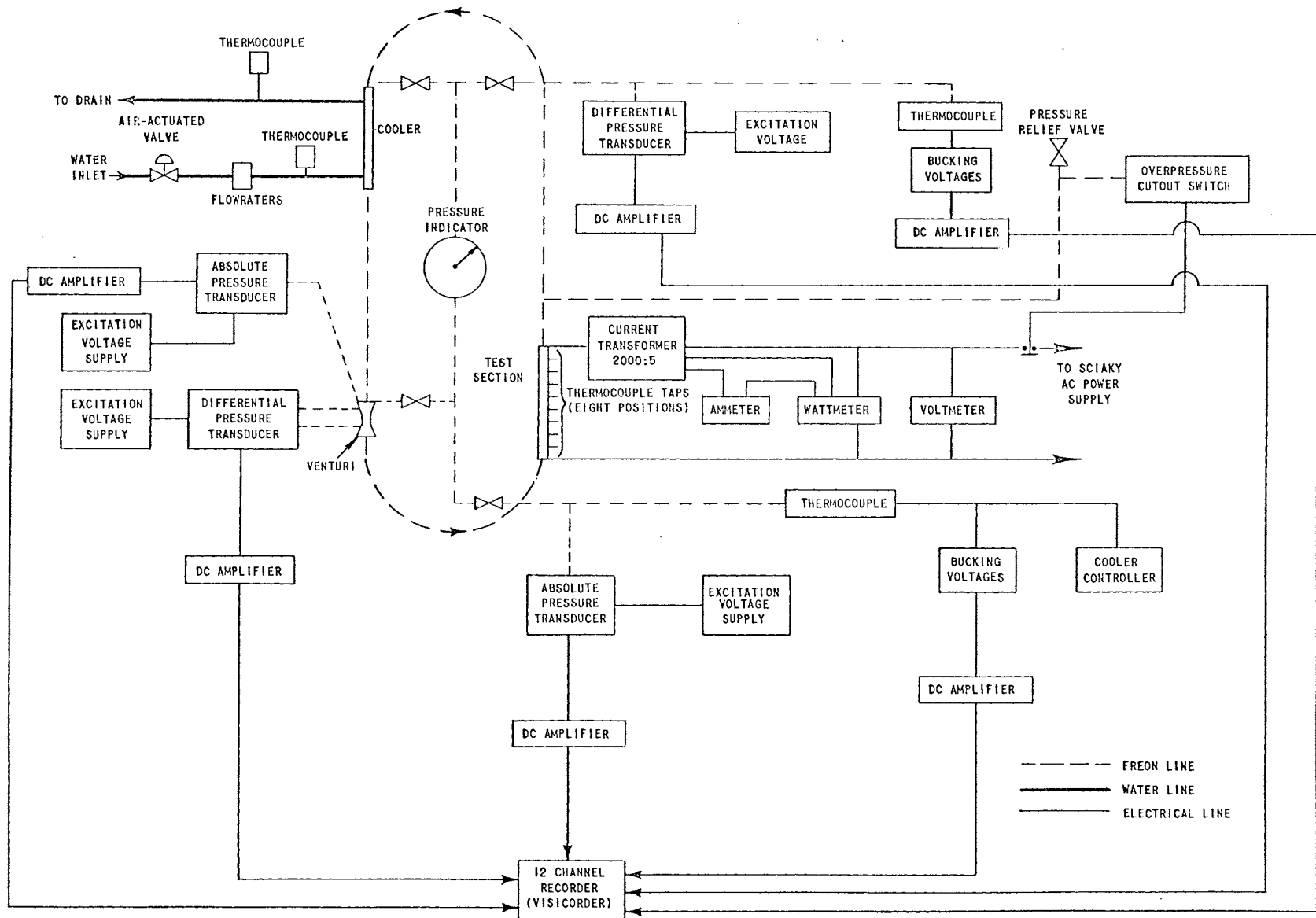
Fig. 6 Instrumentation Block Diagram
