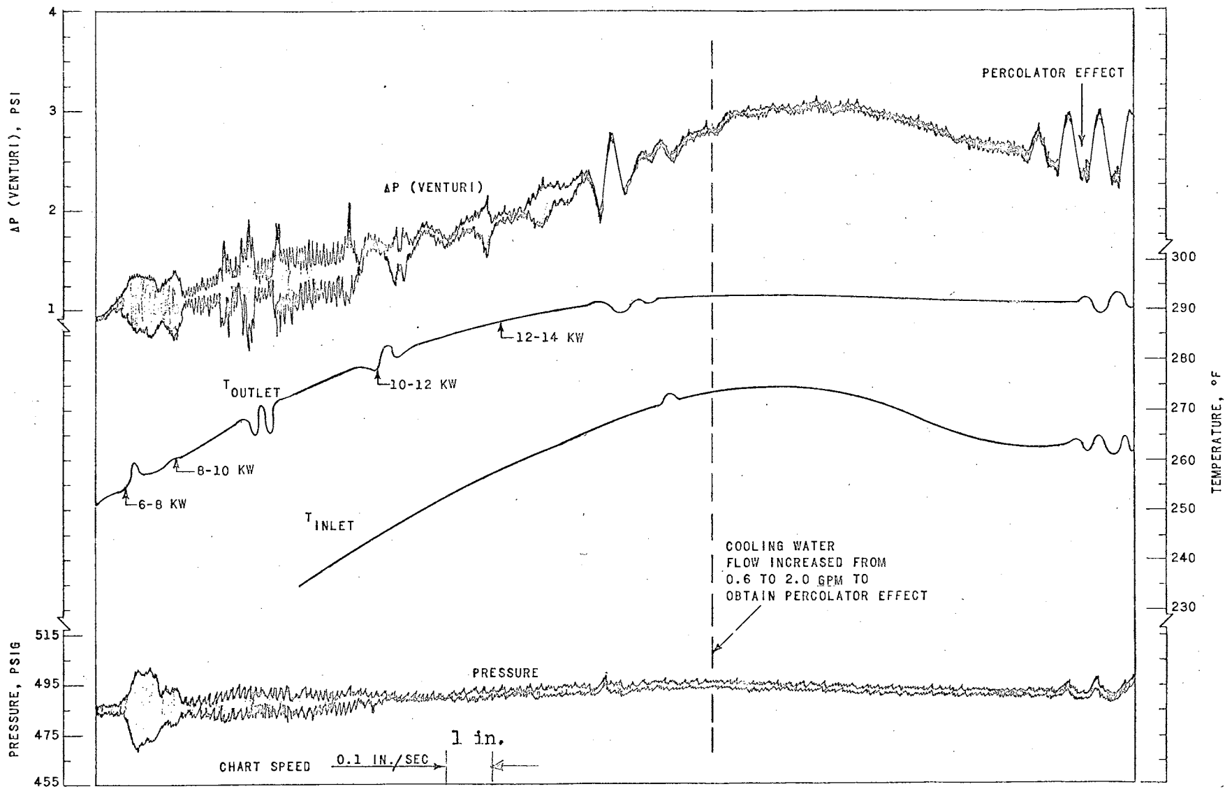
Fig. 21 Rapid Heating Through the [ph] Maximum and Subsequent Cooling, Loop No. 2, Nov. 9, 1962
