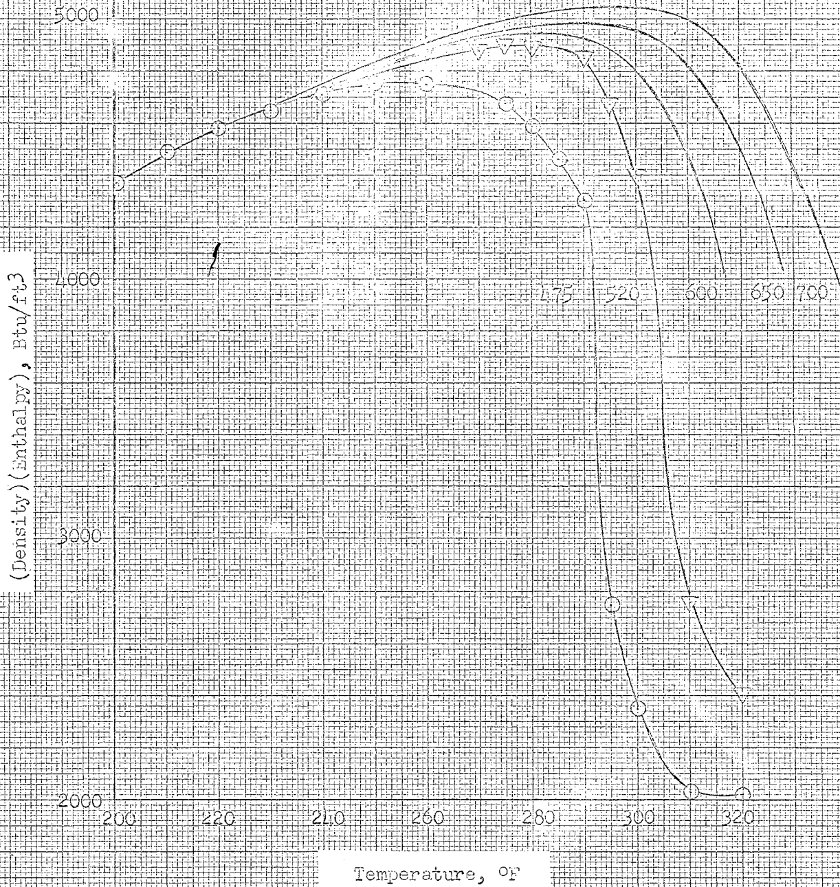
Fig. 13. Density-Enthalpy Product for F-114 along an Isobar as a Function of Temperature.
