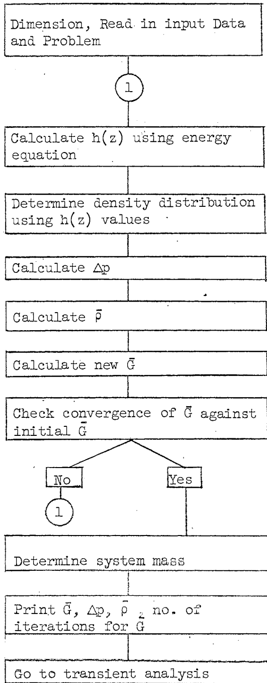
Fig. 36. Simplified Computer Flow Chart for the Steady State Analysis
