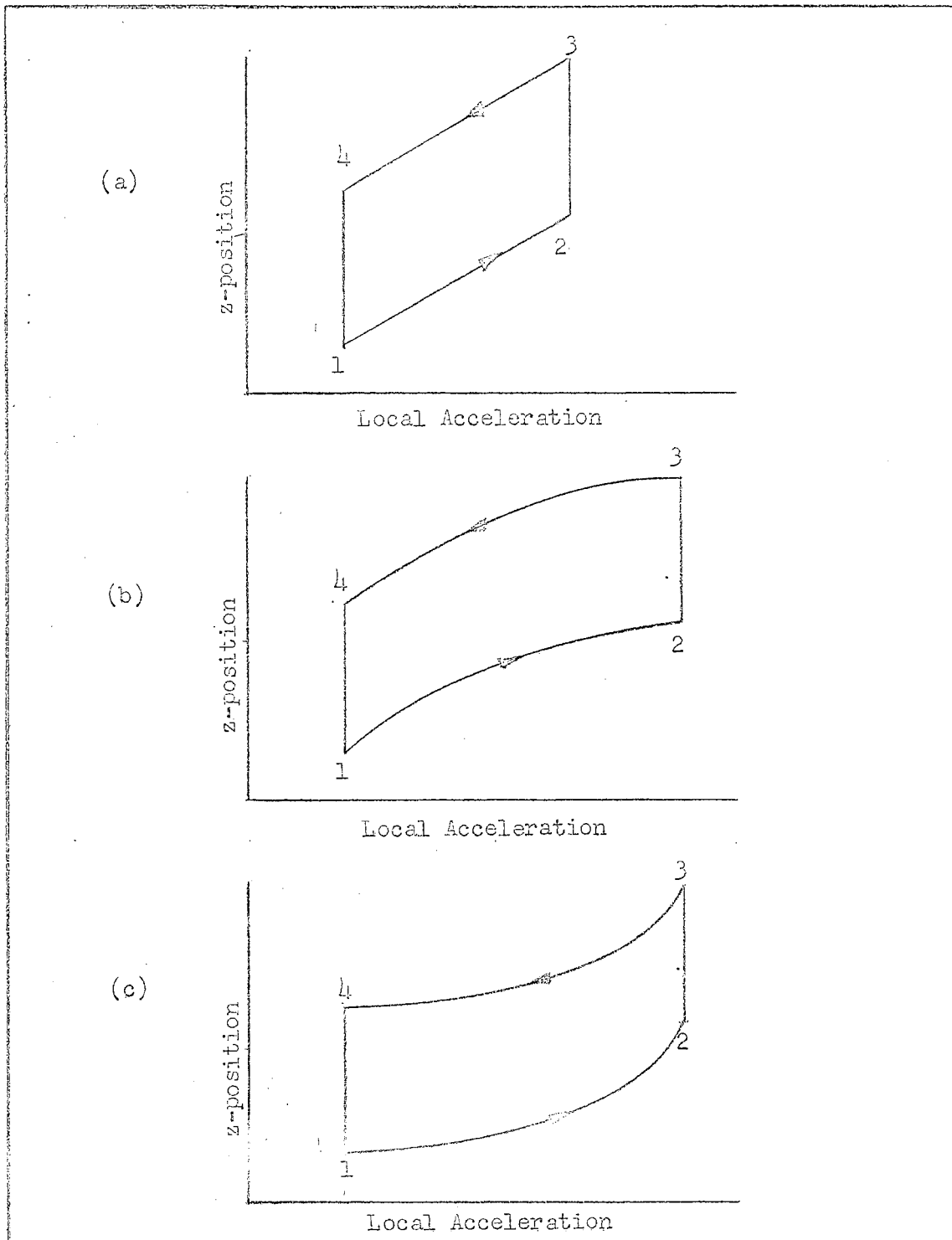
Fig. 3. Fluid Control Volume Position Versus Local Acceleration in a Closed, Natural-Circulation Loop.
