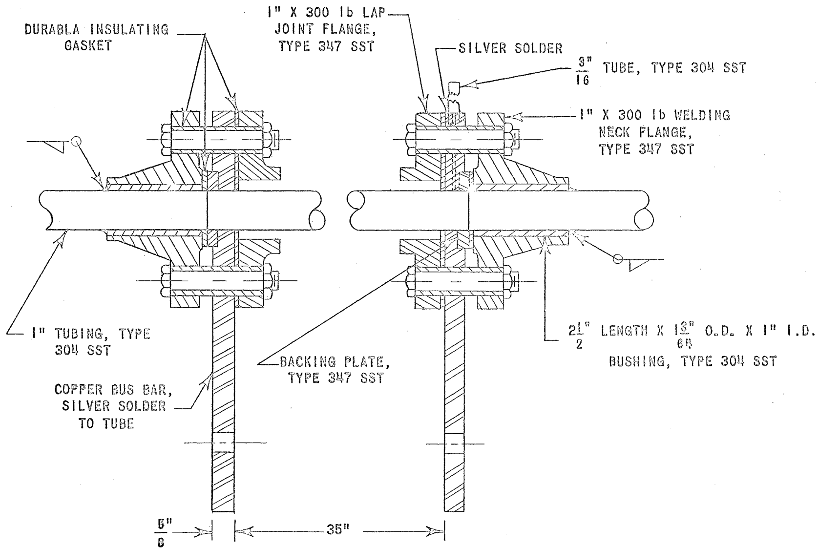
Fig. 9 Assembly Drawing of Test Section
