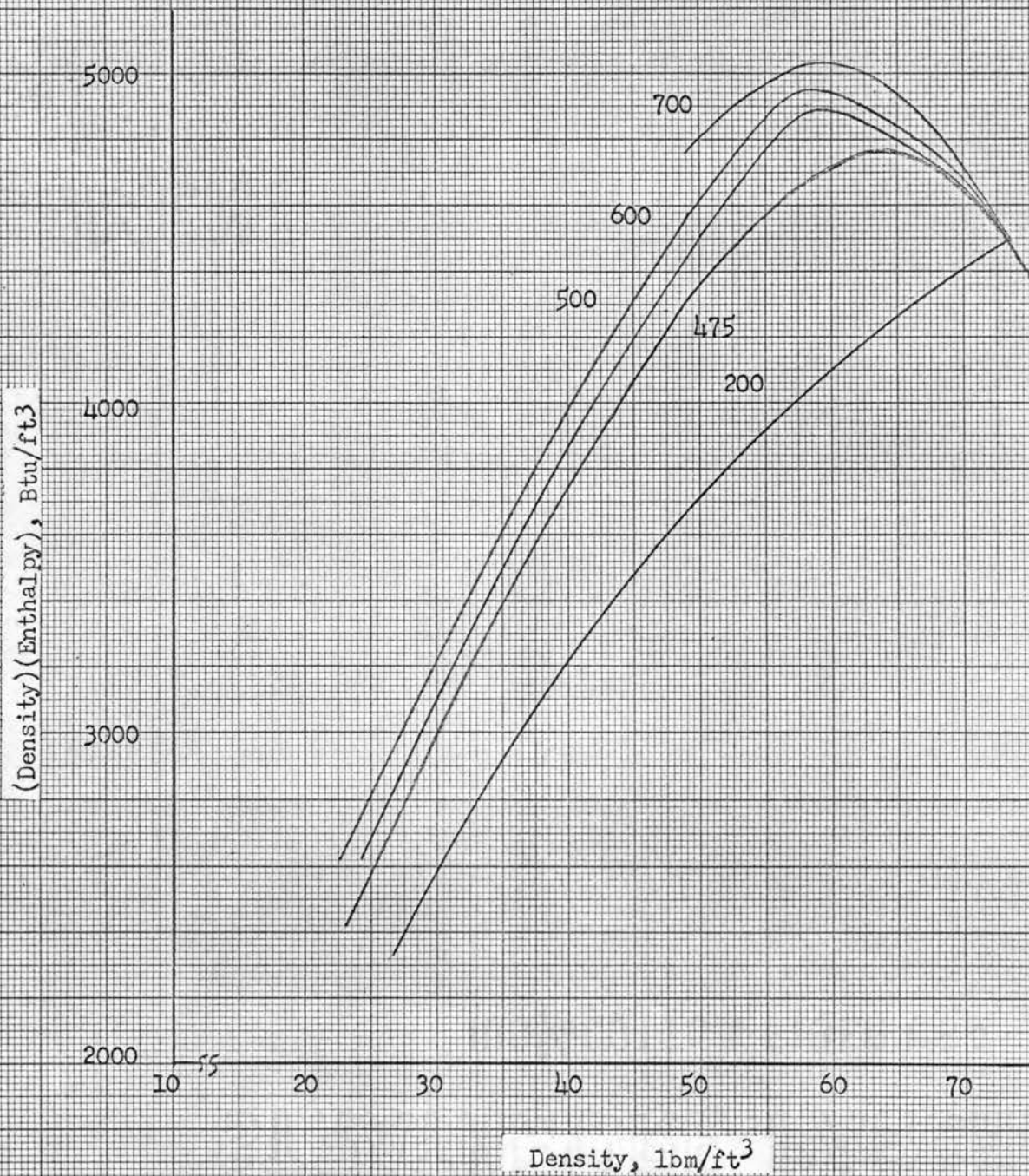
Fig. 39. Density-Enthalpy Product for F-114 along an Isobar as a Function of Density.
