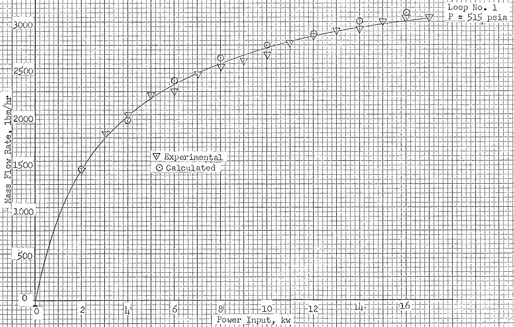
Fig.27 . Comparison of Experimental and Calculated Flow Rates
