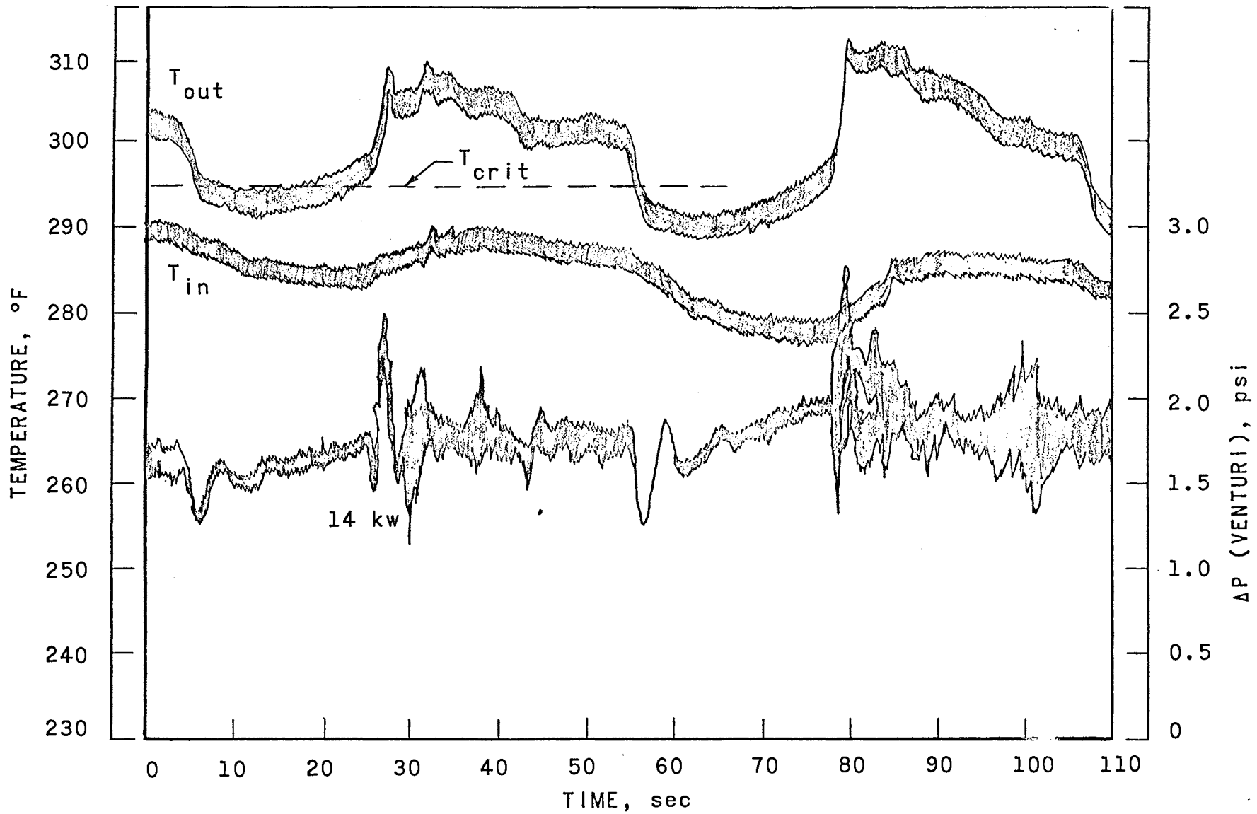
Fig. 17 Power Instability, Loop No. 1, 14 kw, 480 psia, Oct. 3, 1962
