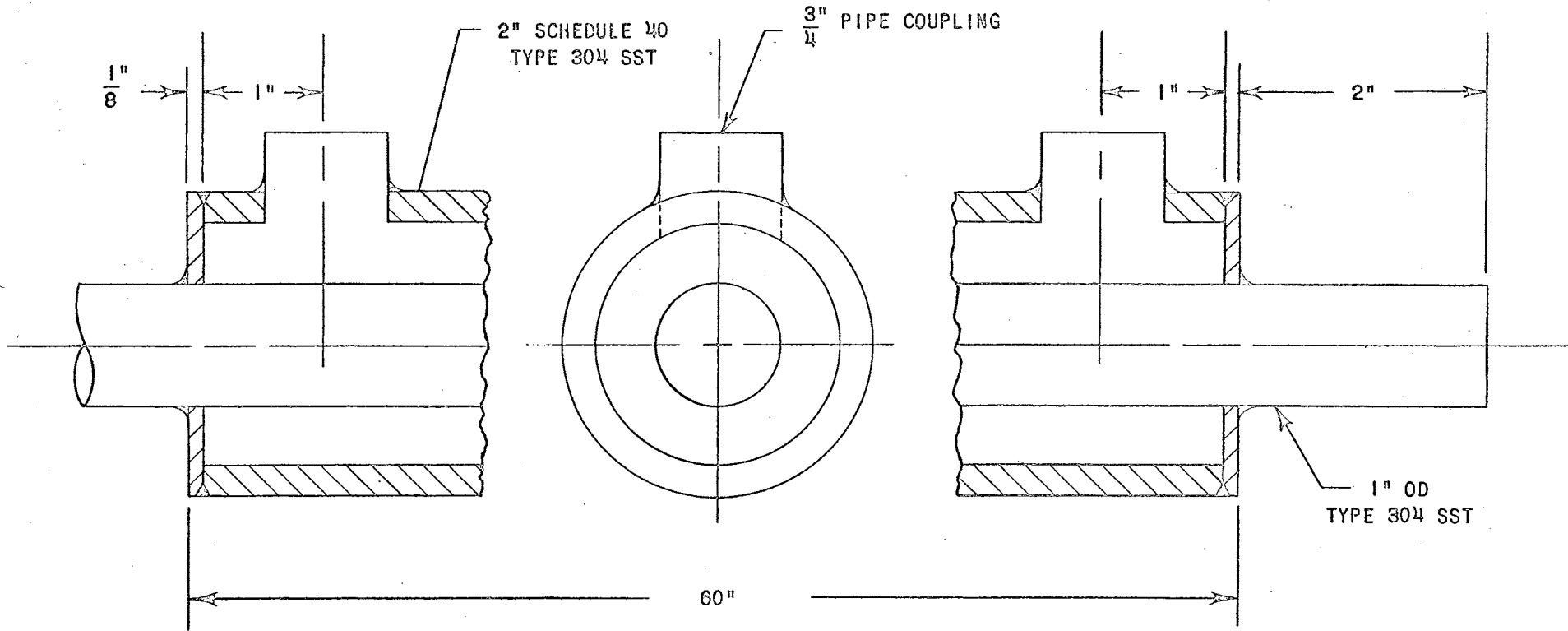
Fig. 10 Heat Exchanger Detail
