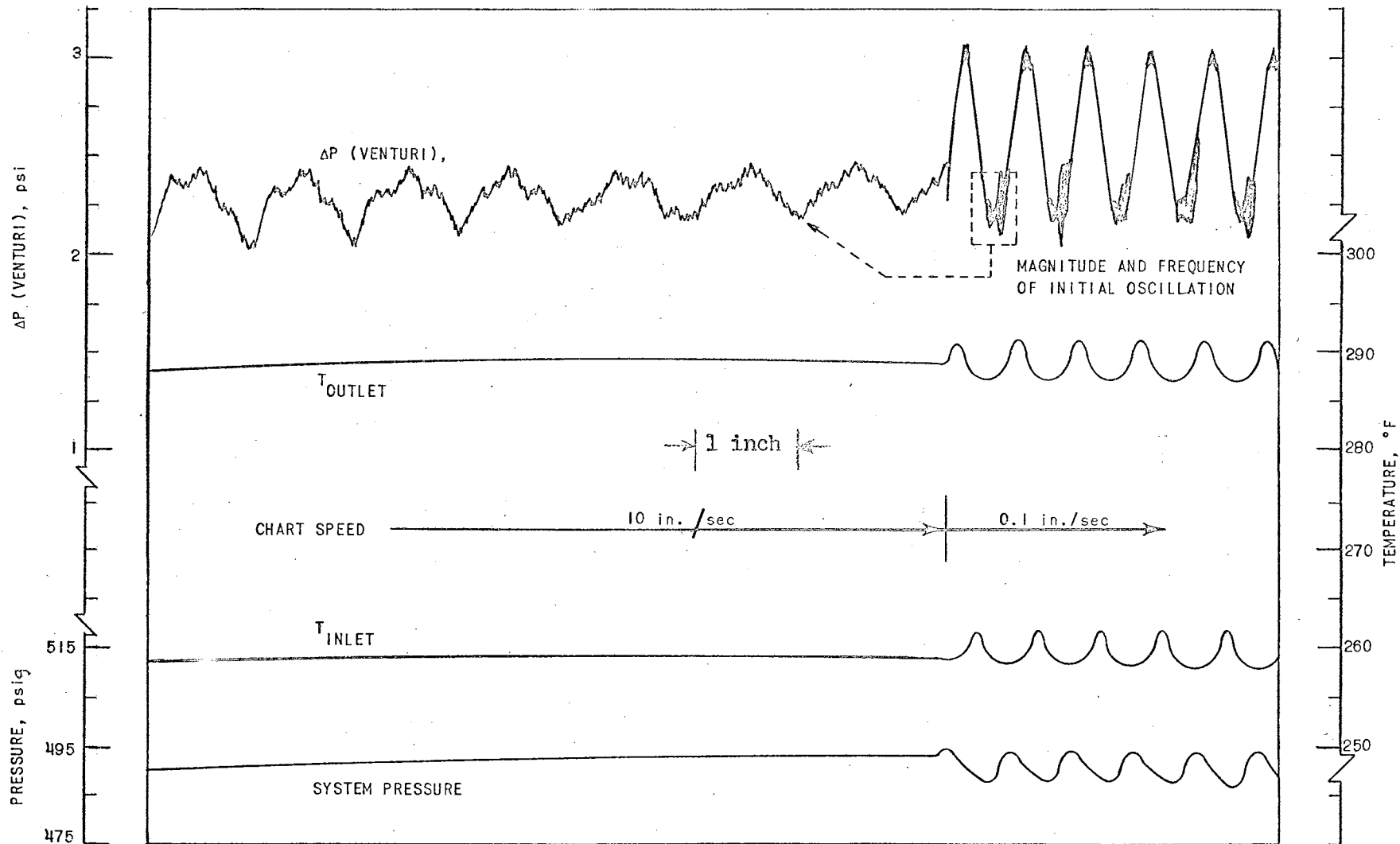
Fig. 19 Initial Oscillation Accompanying "Percolater Effect", Loop No. 2, 14 kw, Nov. 9, 1962
