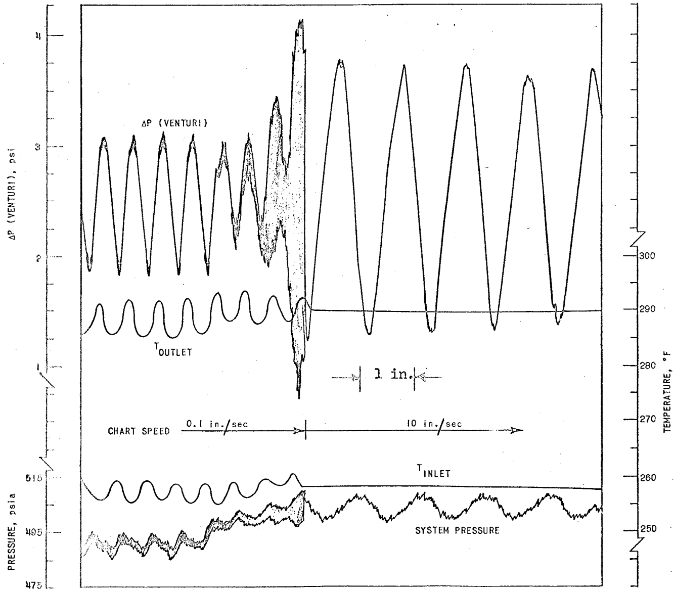
Fig. 25 Effect of Pressure Increase on Magnitude and Frequency, Loop No. 2, 14 kw, Nov. 9, 1962
