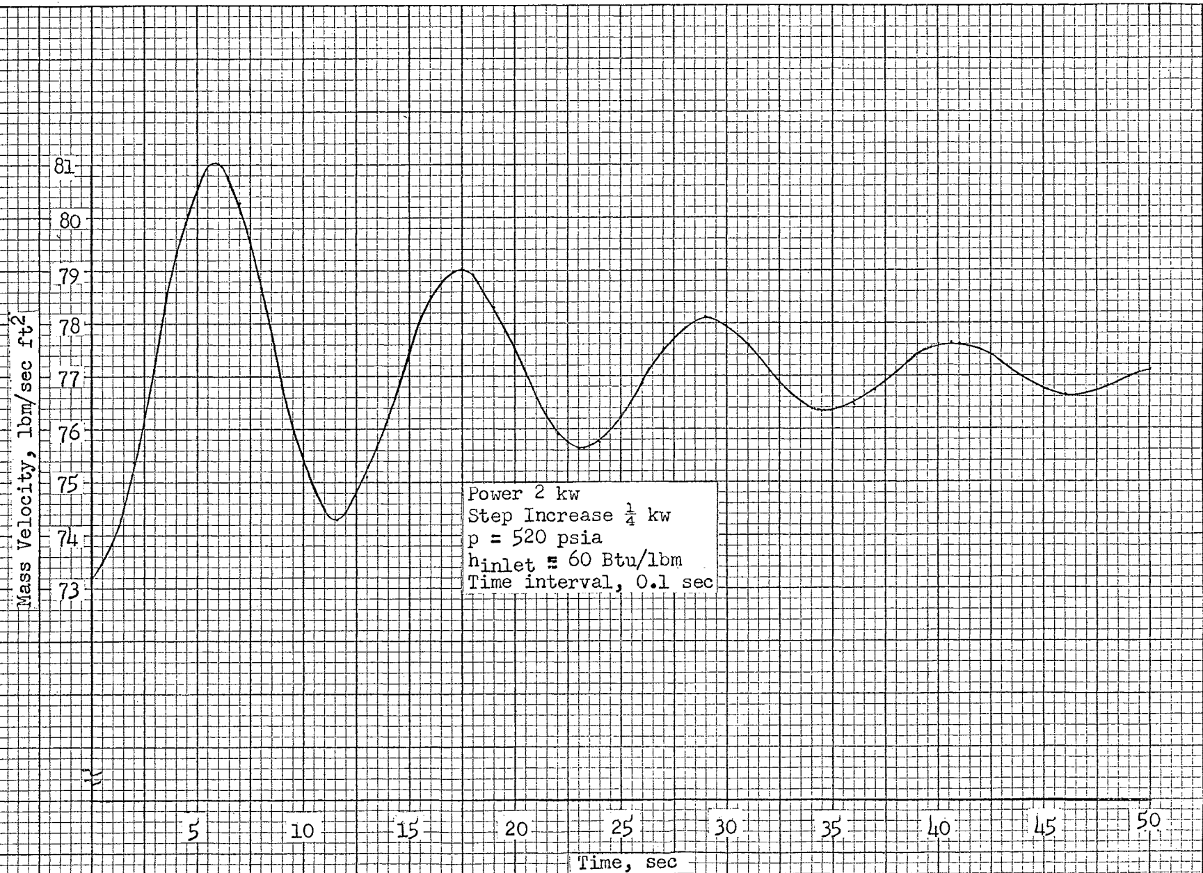
Fig. 30. Predicted Response of Loop No. 1 in a Stable Operating Region
