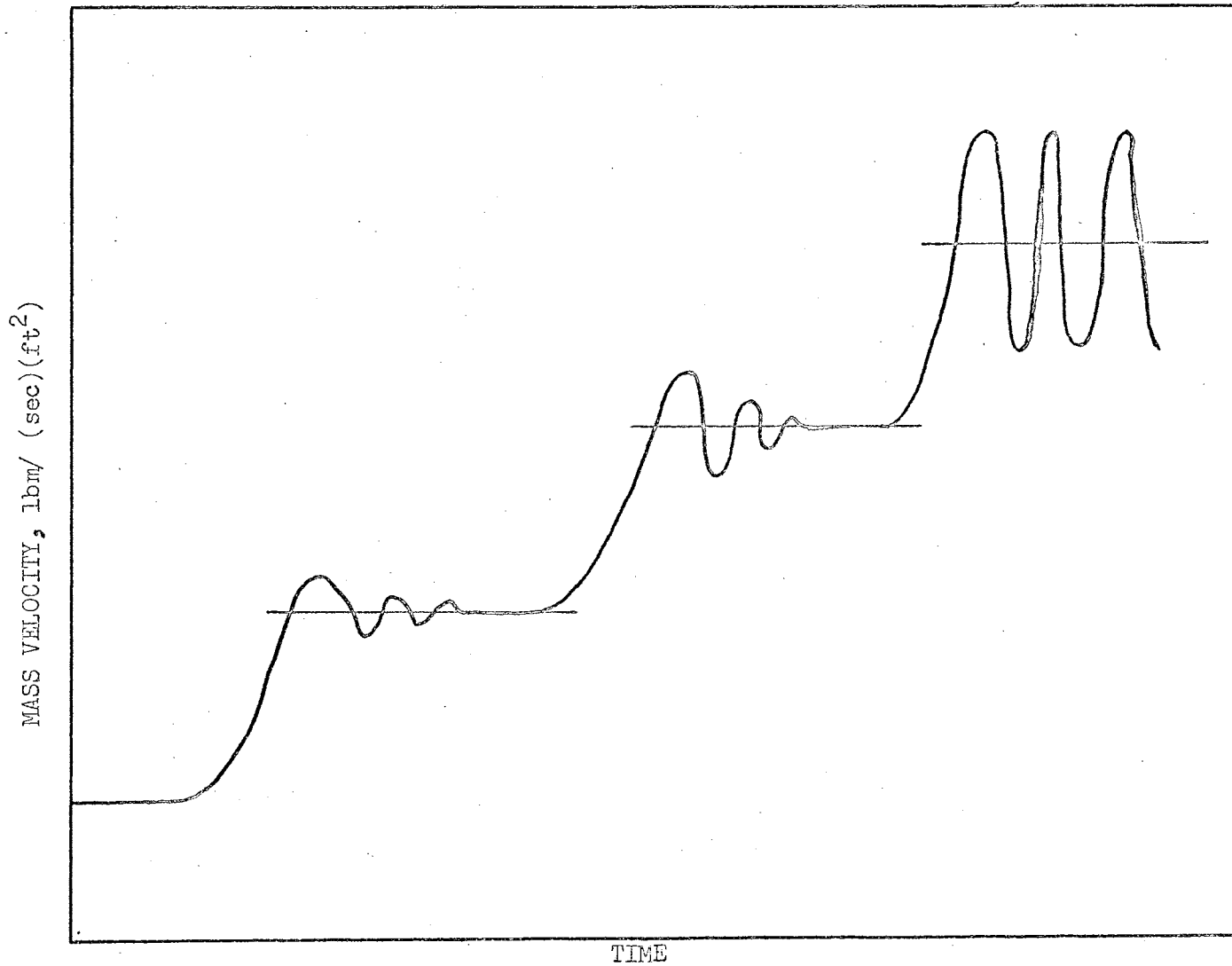
Fig. 2. Response of Natural-Circulation Loop to Step Increase in Heat Input
