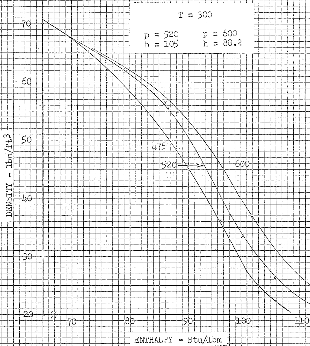
Fig. 14. Isobars of Density-Enthalpy for Freon-114
