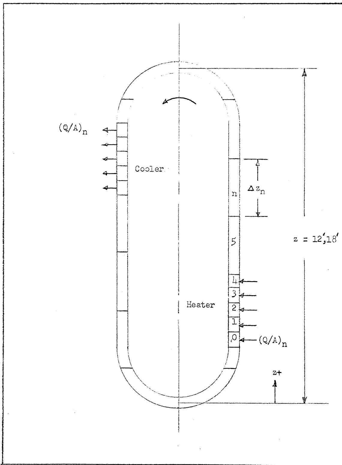
Fig. 1. Schematic of the Loop for Analytical Representation.
