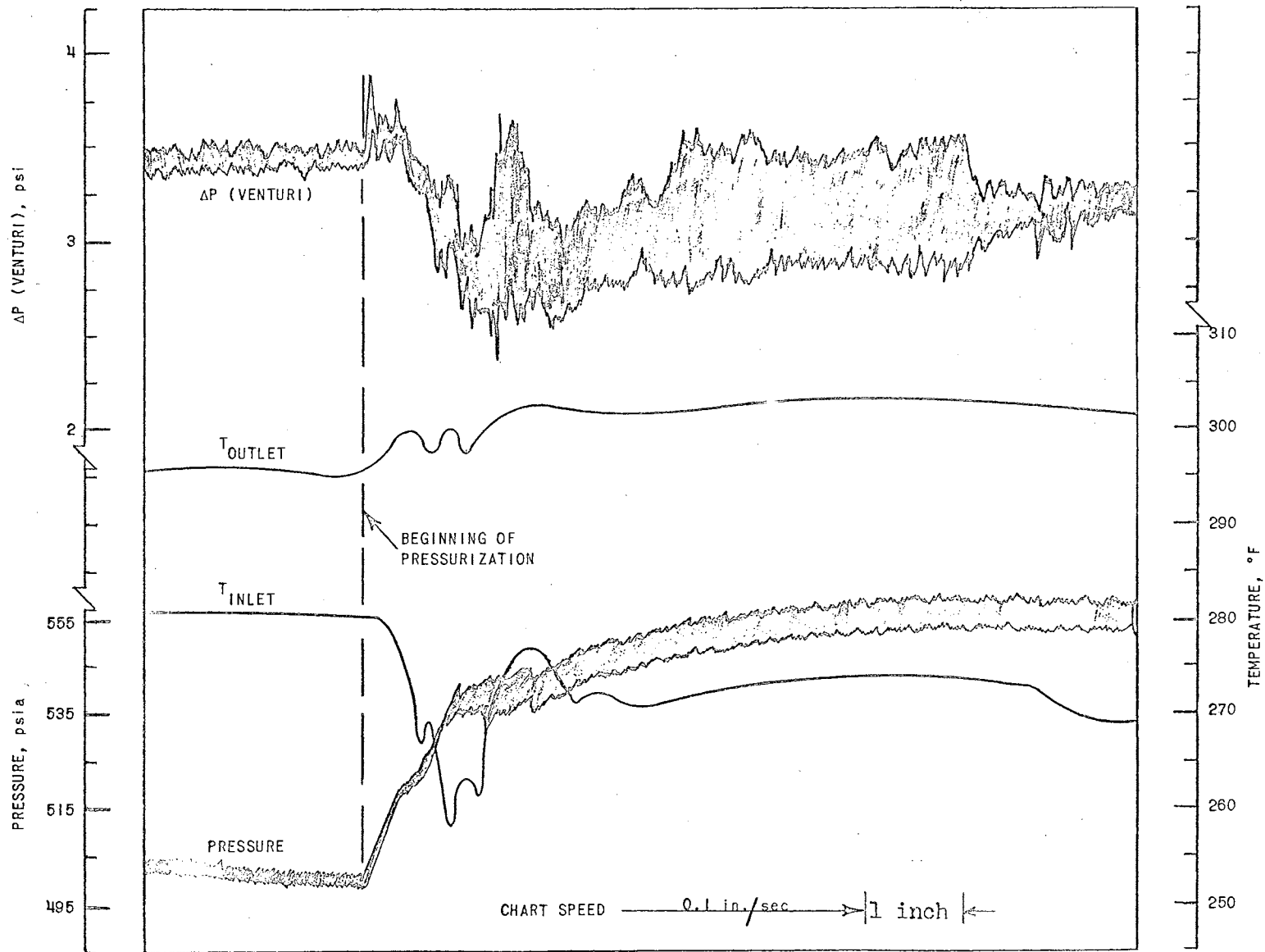
Fig. 18 Effect of Pressurization, Loop No. 2, 16 kw, Nov. 9, 1962
