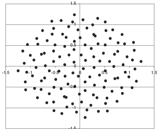
Fig. 6 Hammersley method
