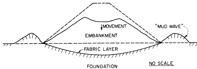
c. EXCESSIVE SETTLEMENT BEFORE STABLE BEARING CONDITIONS WERE ACHIEVED
