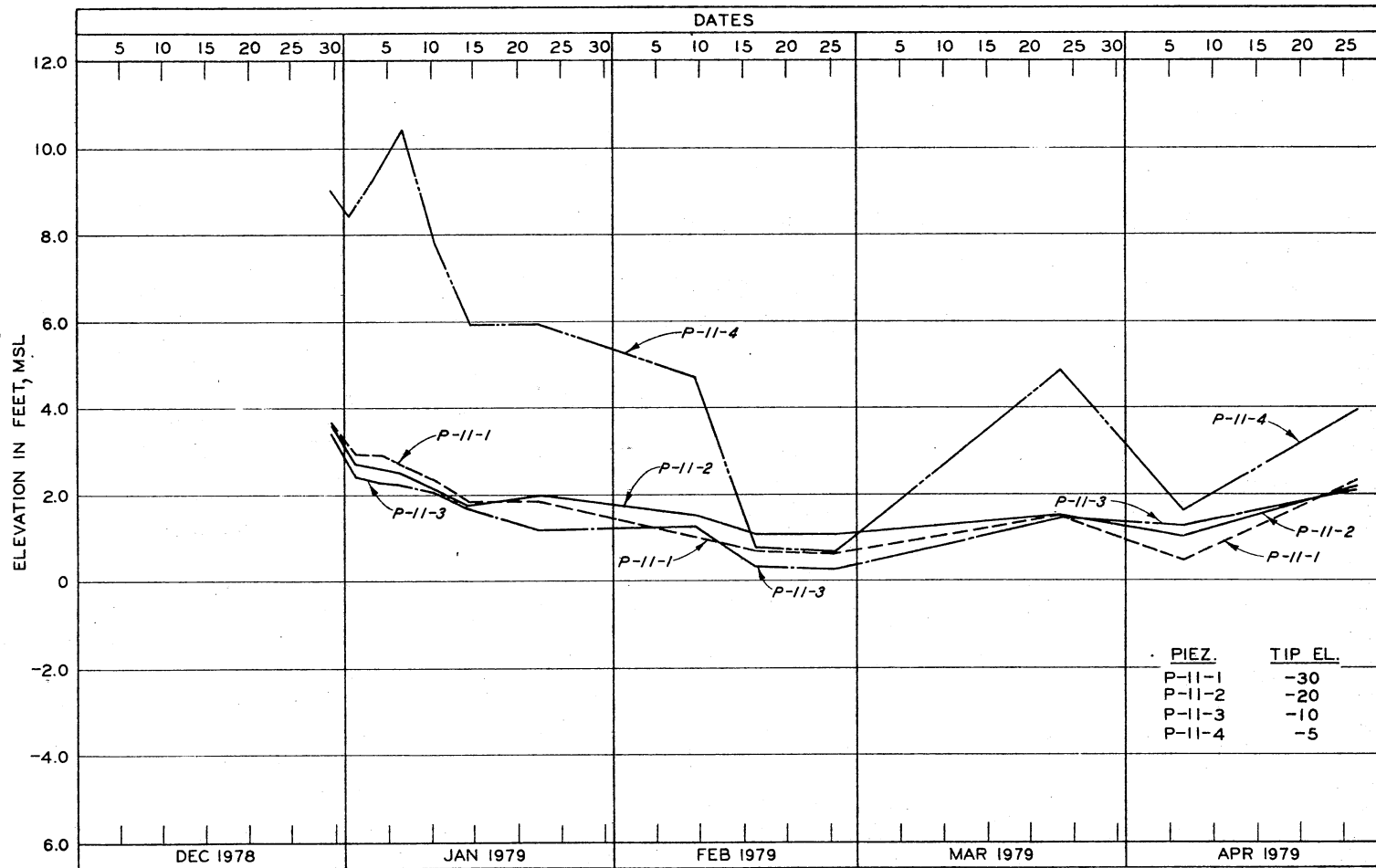
Figure 90. Pore Pressure versus Time for Piezometers P-11-1 through P-11-4
