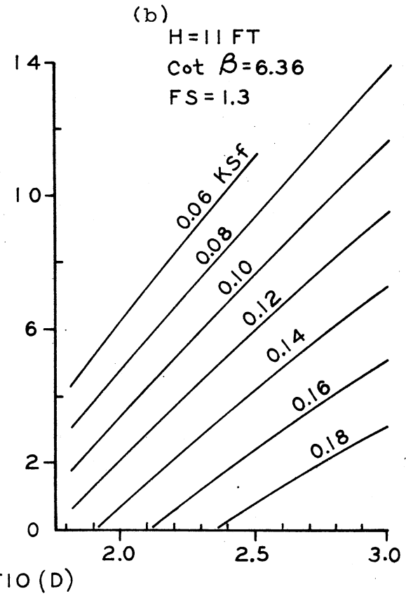
Figure 98. Design Curves for Dike Height = 11 ft
