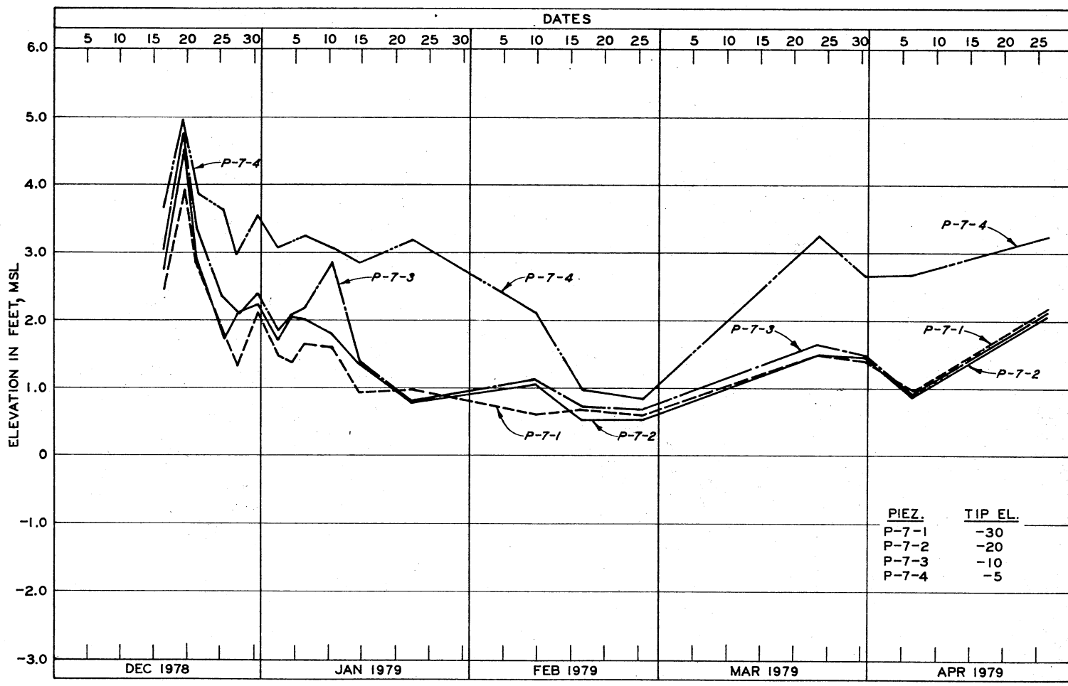
Figure 86. Pore Pressure versus Time for Piezometers P-7-1 through P-7-4
