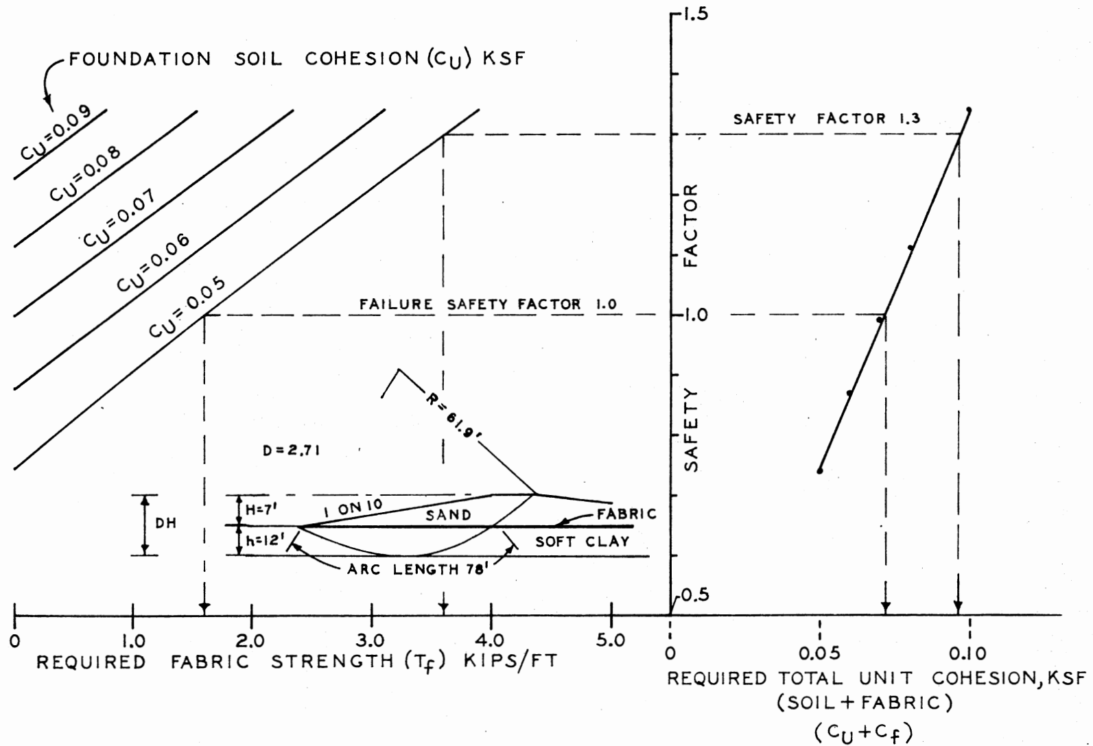
Figure 96. Typical Curves Used to Develop Design Curves
