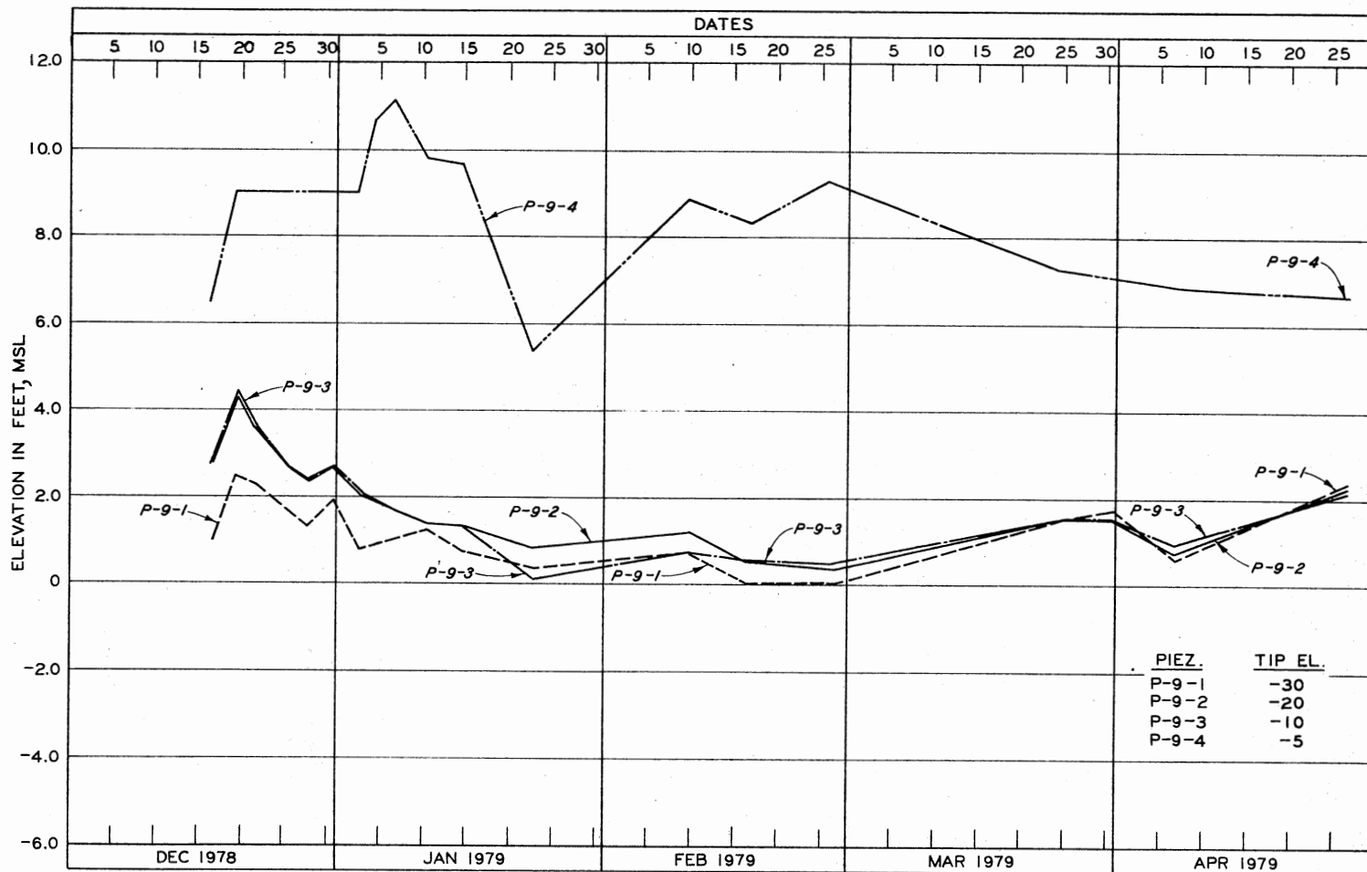
Figure 88. Pore Pressure versus Time for Piezometers P-9-1 through P-9-4
