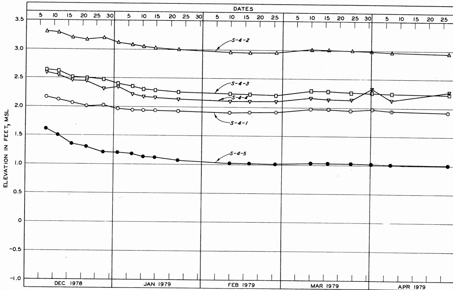
Figure 71. Settlement versus Time for Settlement Plates S-4-1 through S-4-5
