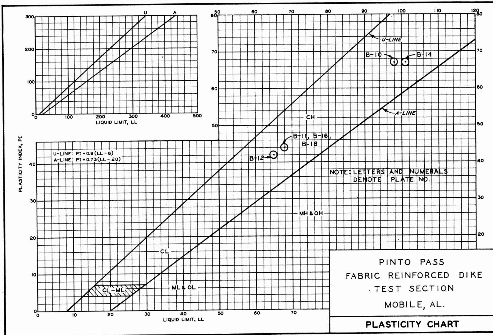
Figure 30. Plasticity Index versus Liquid Limit of Undisturbed Samples Used in Triaxial Tests
