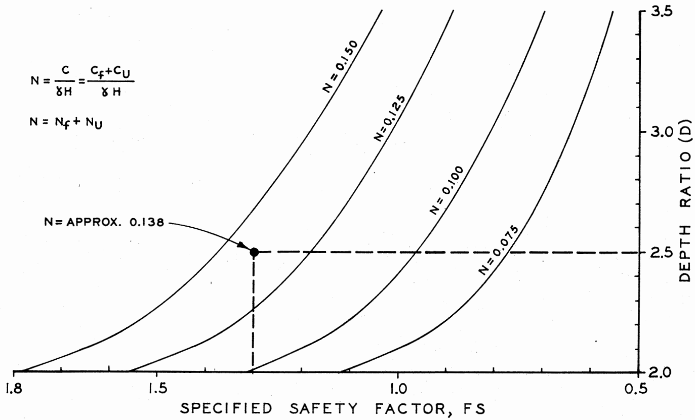
Figure 100. Design Chart 1 for Determining Stability Number N
