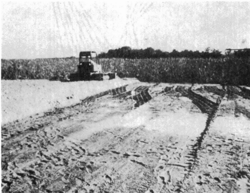
Figure 44. Dozer Spreading Dry Sand. Note Right Portion of Photo Shows Pore Water that Had Risen Overnight through Sand and Was Running off of the Working Table
