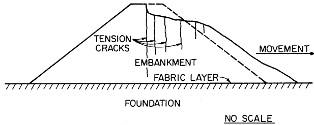
a. SLIDING WEDGE FAILURE OF EMBANKMENT
