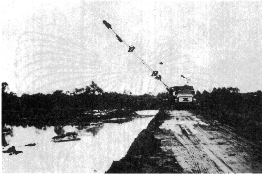
Figure 41. Dragline Loading Dump Truck at Dredged Material Disposal Area Borrow Pit
