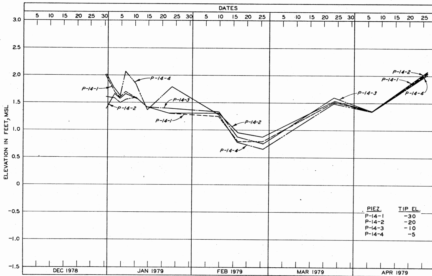
Figure 93. Pore Pressure versus Time for Piezometers P-14-1 through P-14-4
