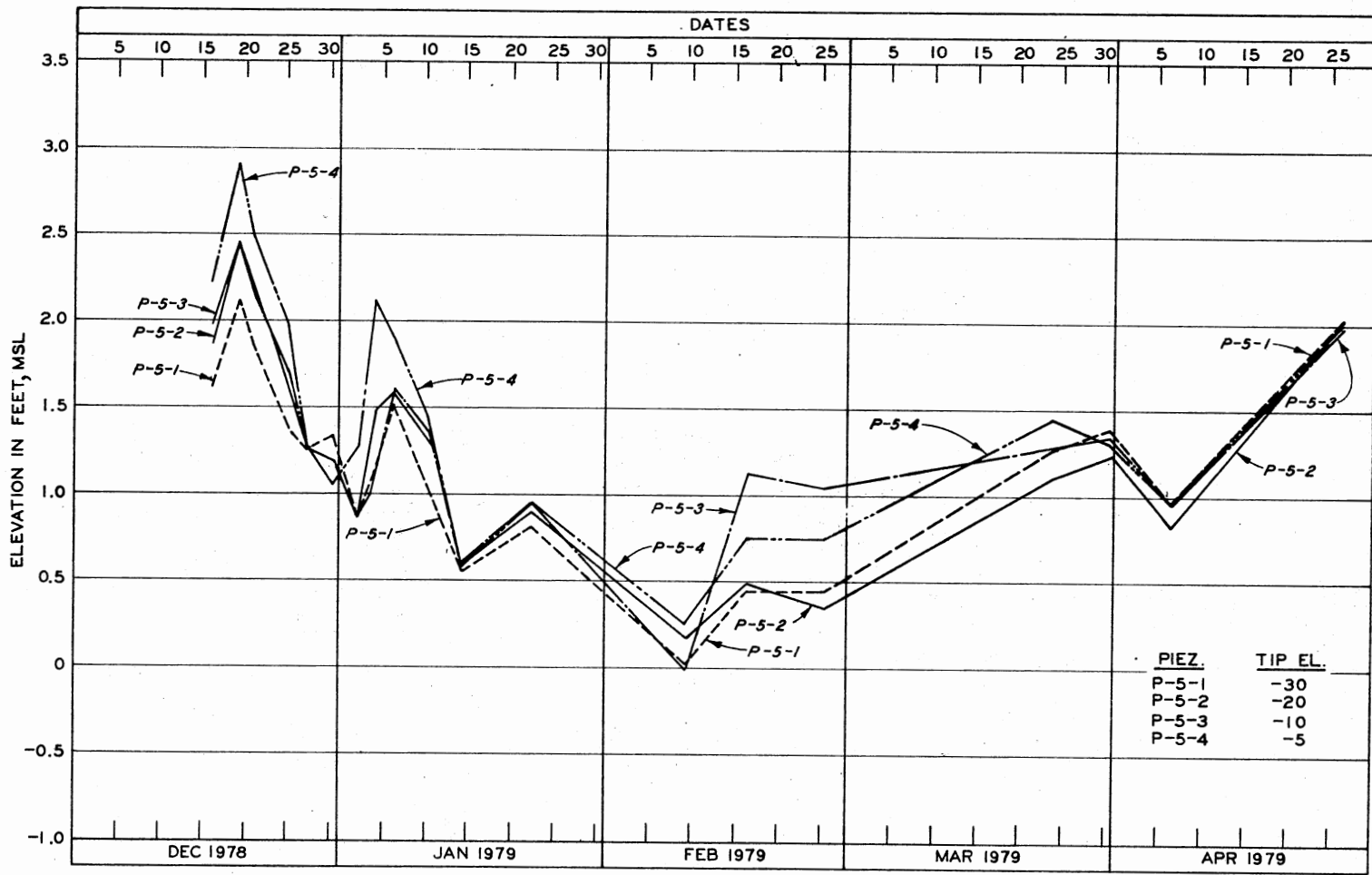
Figure 84. Pore Pressure versus Time for Piezometers P-5-1 through P-5-4
