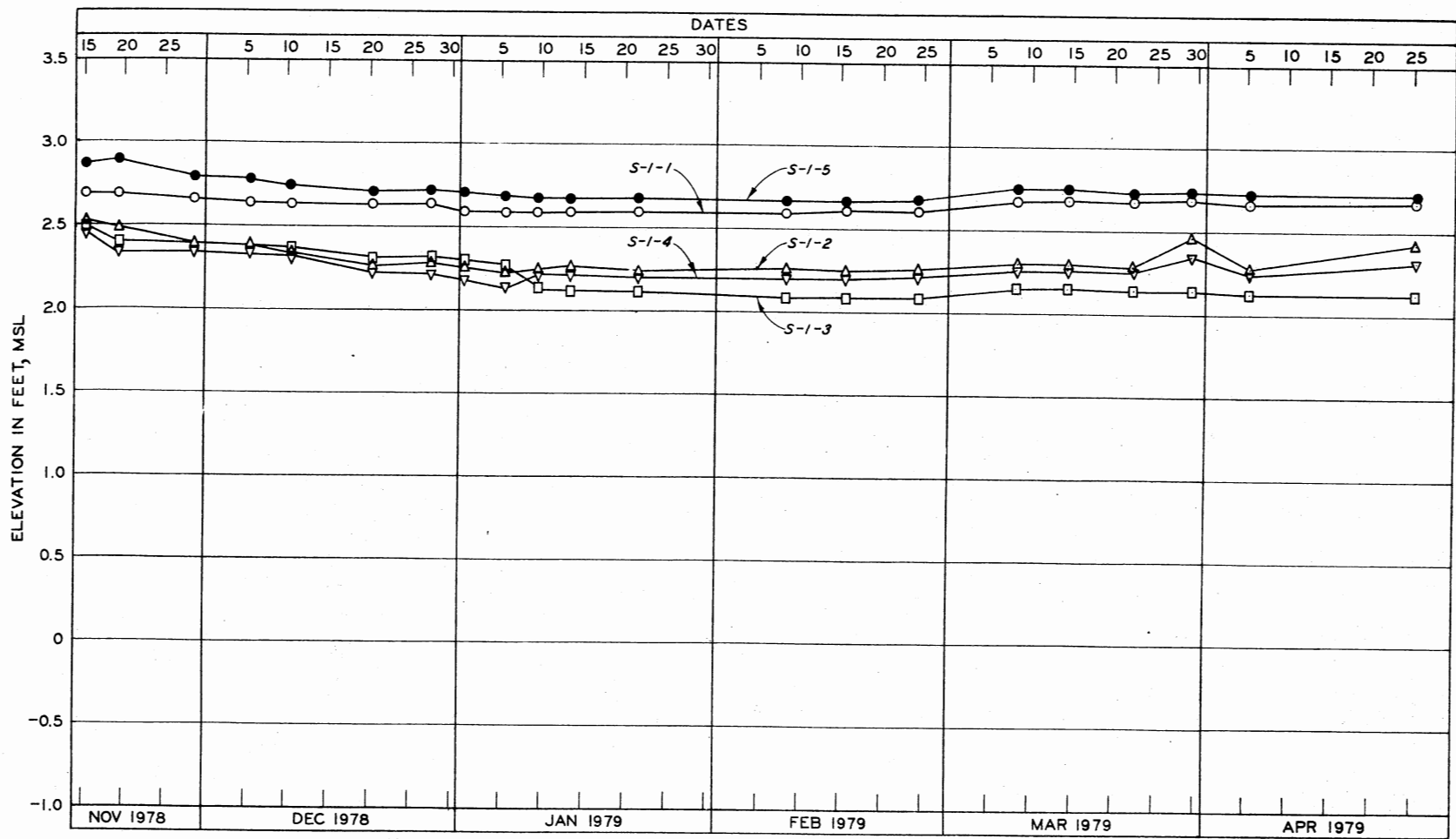
Figure 68. Settlement versus Time for Settlement Plates S-1-1 through S-1-5
