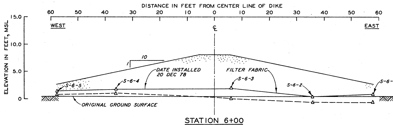
Figure 77. Settlement Profiles for Stations 5+00 and 6+00
