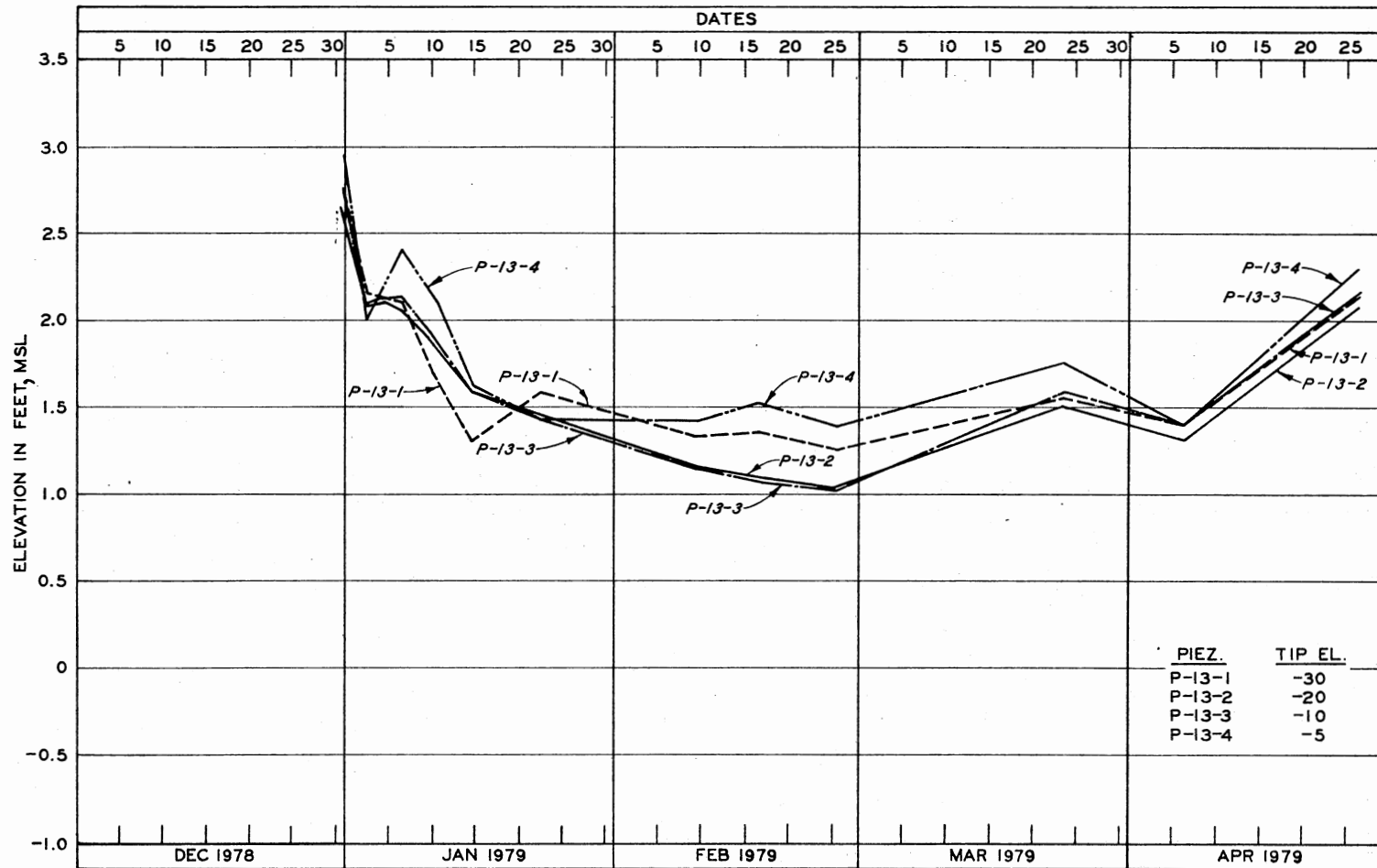
Figure 92. Pore Pressure versus Time for Piezometers P-13-1 through P-13-4
