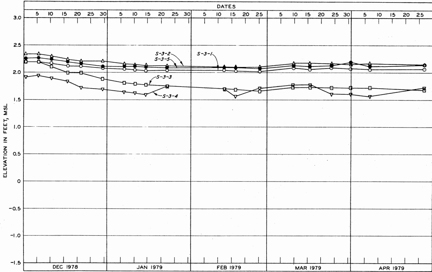
Figure 70. Settlement versus Time for Settlement Plates S-3-1 through S-3-5
