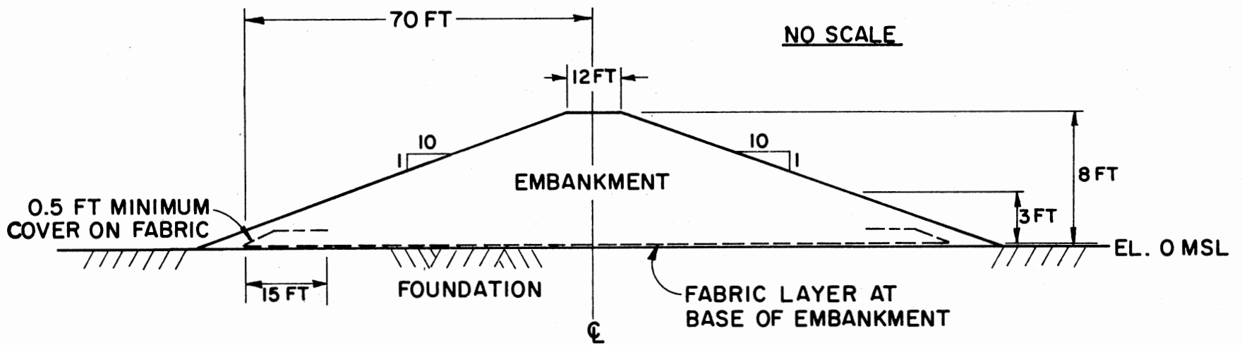
Figure 17. Simplified Fabric-reinforced Embankment Section Used for Analysis Purposes
