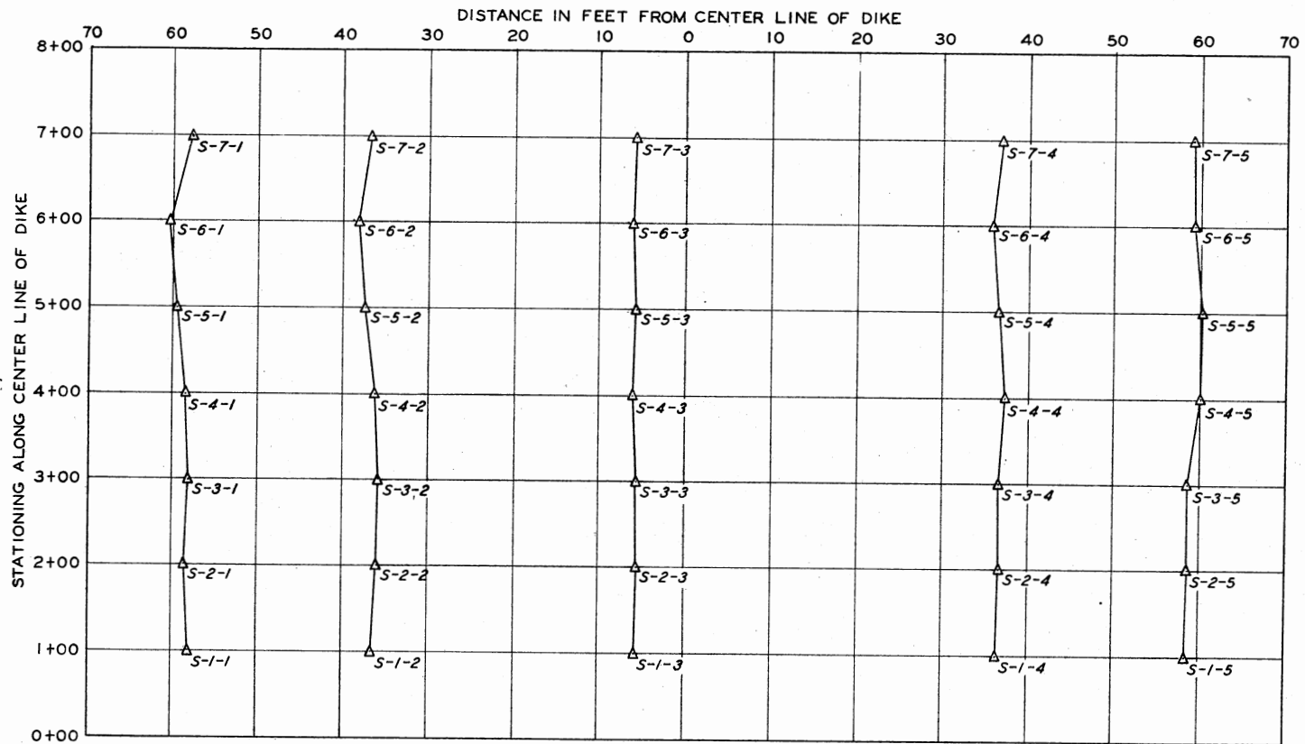
Figure 79. Plan View of Maximum Horizontal Displacement
