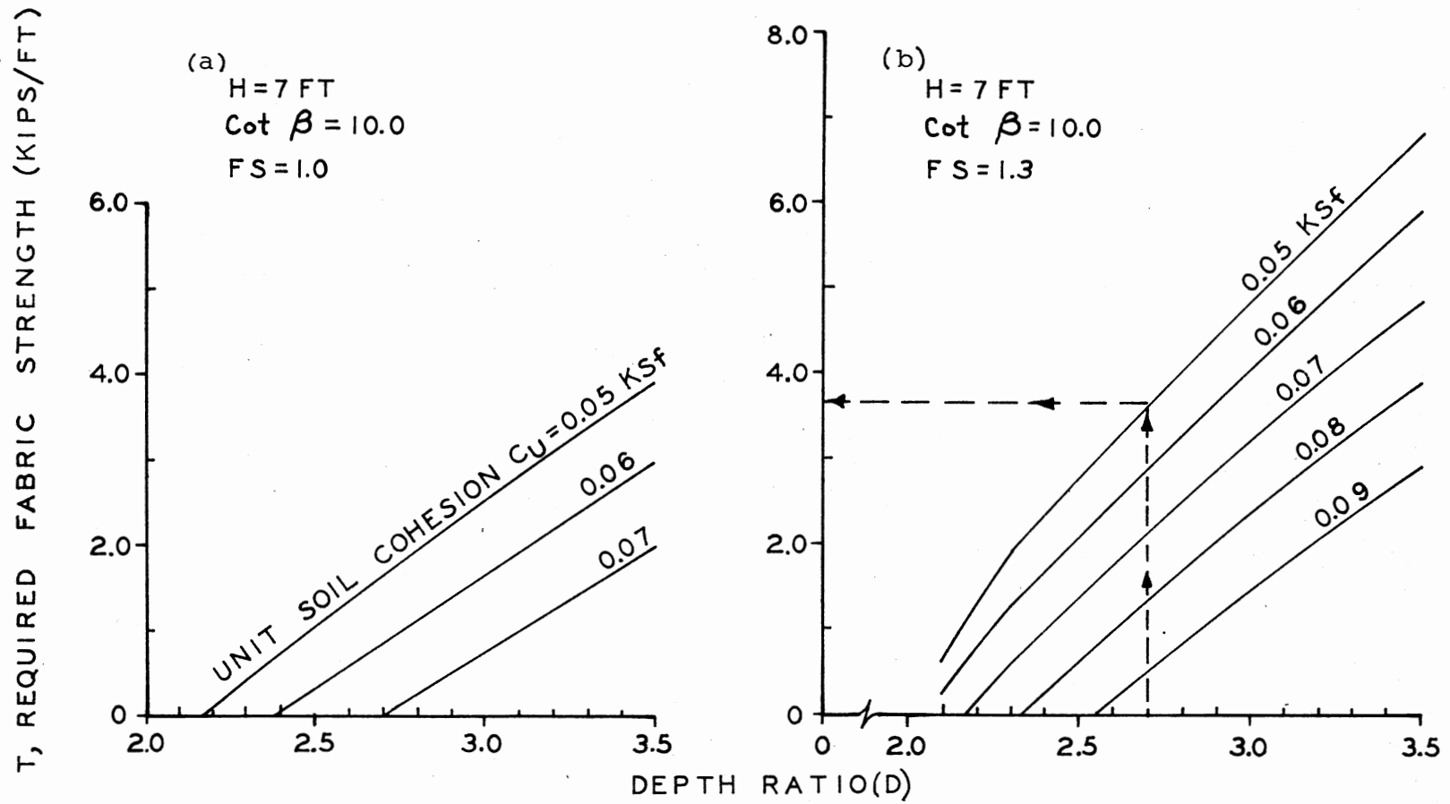
Figure 97. Design Curves for Dike Height = 7 ft
