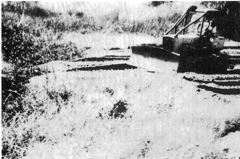
Figure 42. John Deere 350 Wide-track (28 in.) Dozer Spreading a 1-ft Layer of Borrow Material onto Grass Covering
