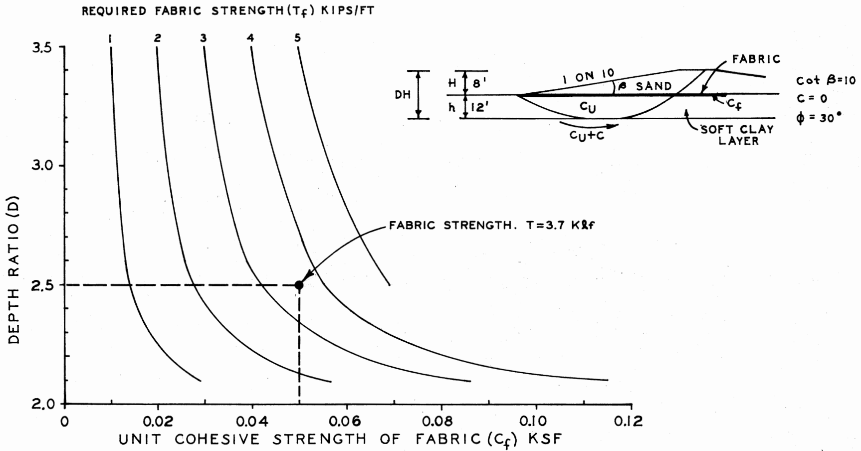
Figure 101. Design Chart 2 for Determining Fabric Strength T_f
