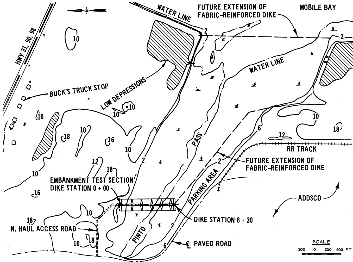
Figure 9. Location of Embankment Test Section, Pinto Pass, Mobile, Alabama
