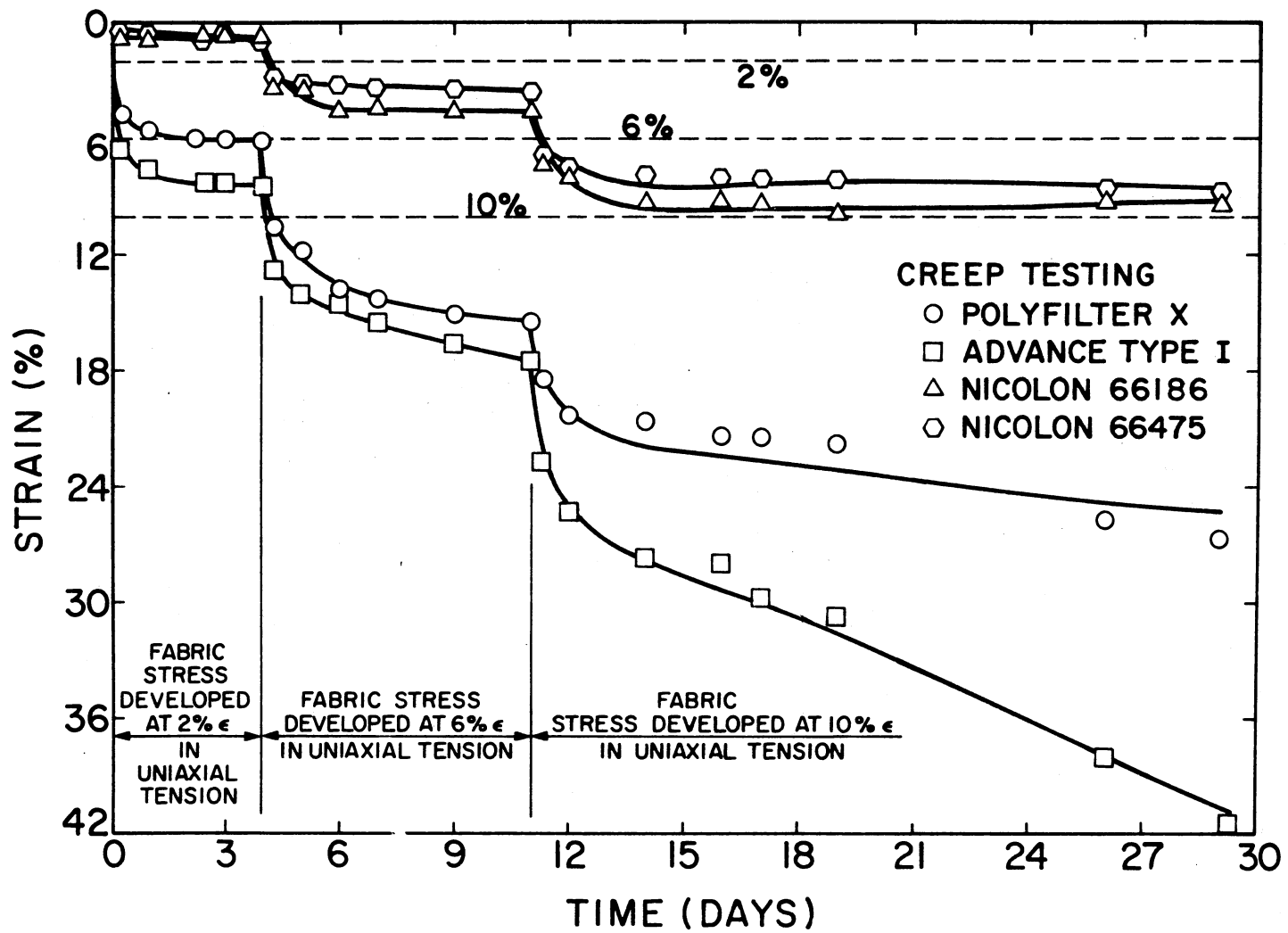
Figure 16. Results of Geotechnical Fabric Creep Testing
