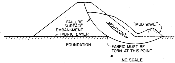
b. LOCAL BEARING FAILURE OF SOFT FOUNDATION
