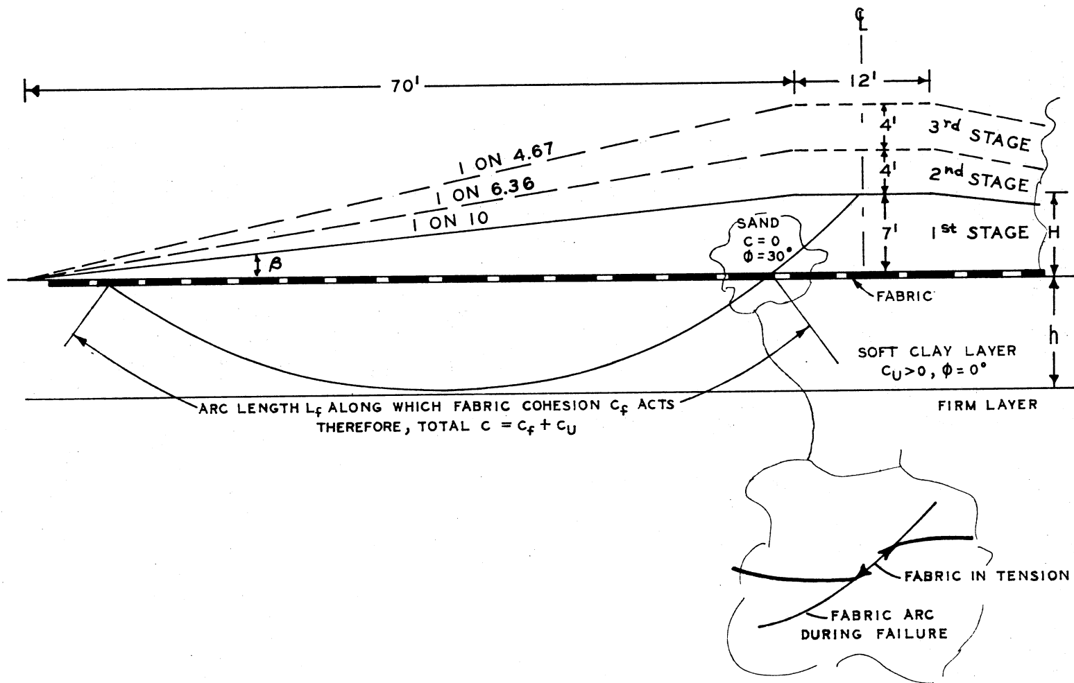
Figure 94. Fabric-reinforced Embankment Test Section
