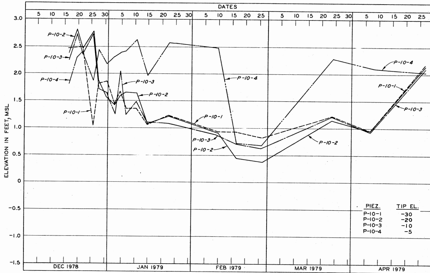
Figure 89. Pore Pressure versus Time for Piezometers P-10-1 through P-10-4
