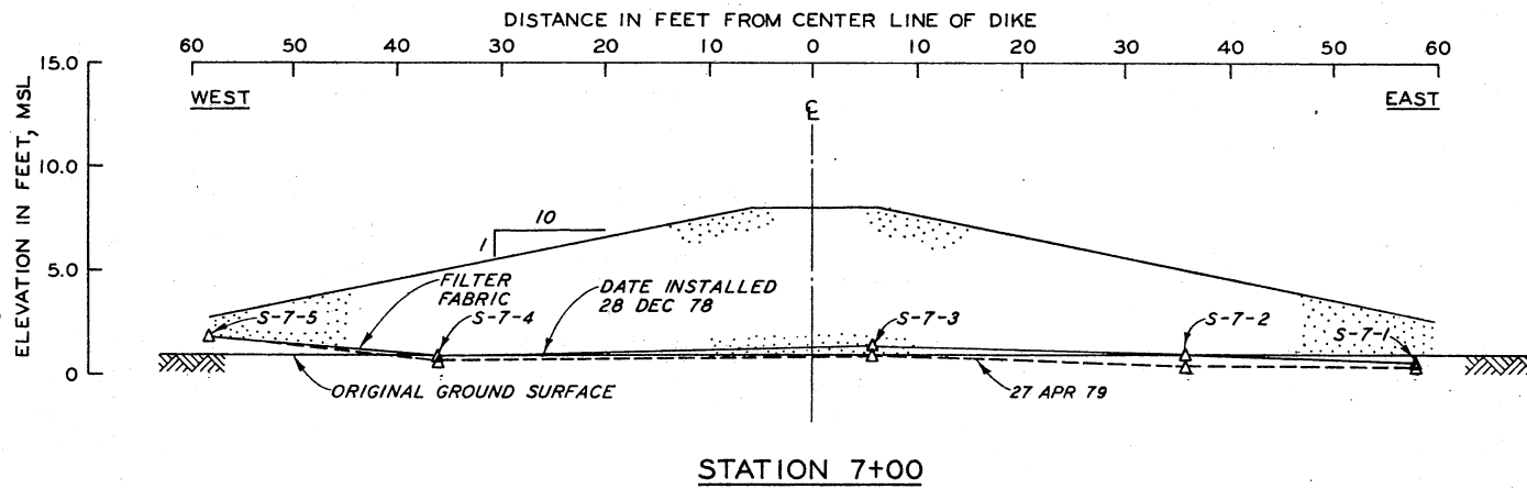
Figure 78. Settlement Profile for Station 7+00
