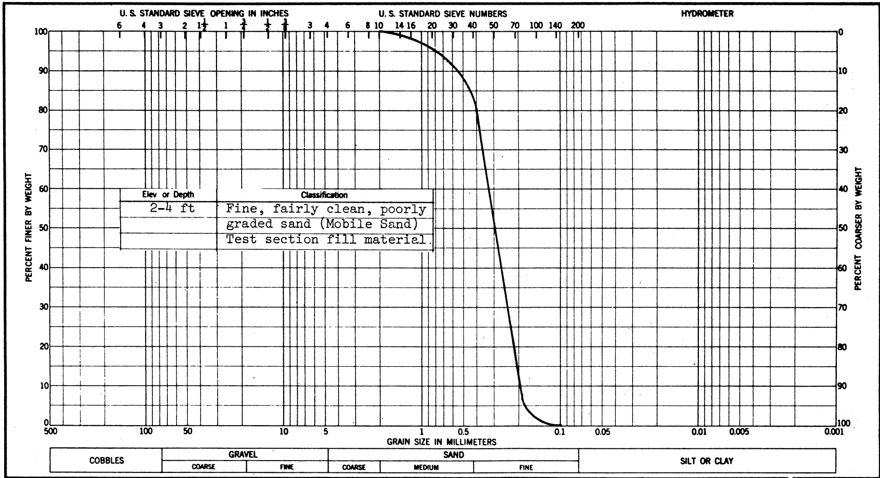
Figure 29. Gradation of Sand Used as Fill Material
