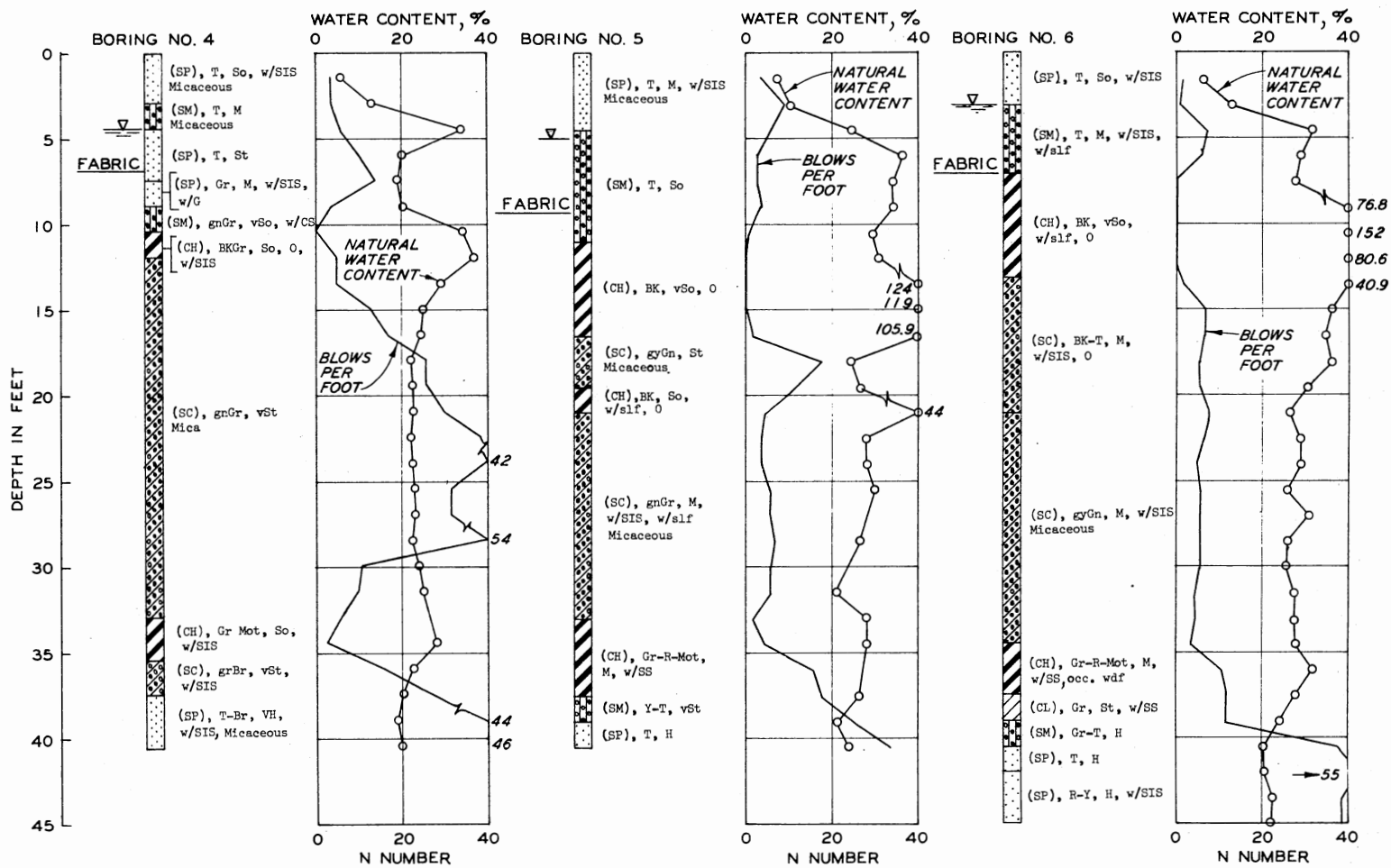
Figure 25. Boring Log and Water Content and N-Number versus Depth for Borings 4, 5, and 6
