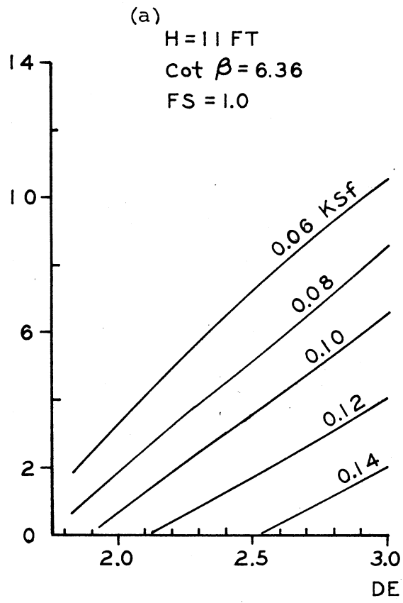
Figure 98. Design Curves for Dike Height = 11 ft
