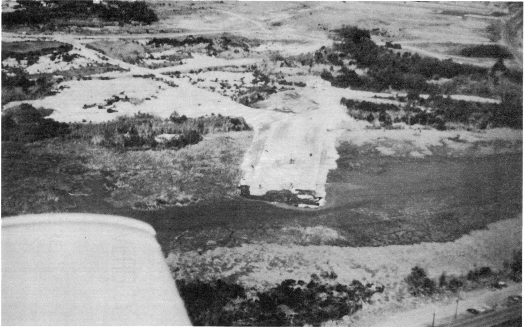
Figure 53. Aerial View of Fabric-reinforced Embankment Being Constructed Across Pinto Pass.
