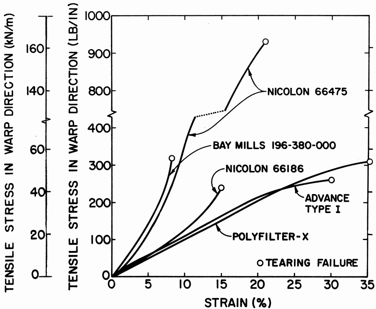
Figure 15. Stress-strain Data for the Five Geotechnical Fabrics Meeting Desired Tensile Strength Criteria
