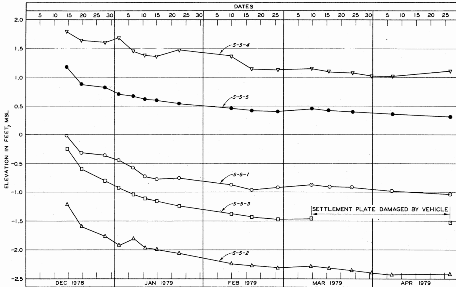
Figure 72. Settlement versus Time for Settlement Plates S-5-1 through S-5-5
