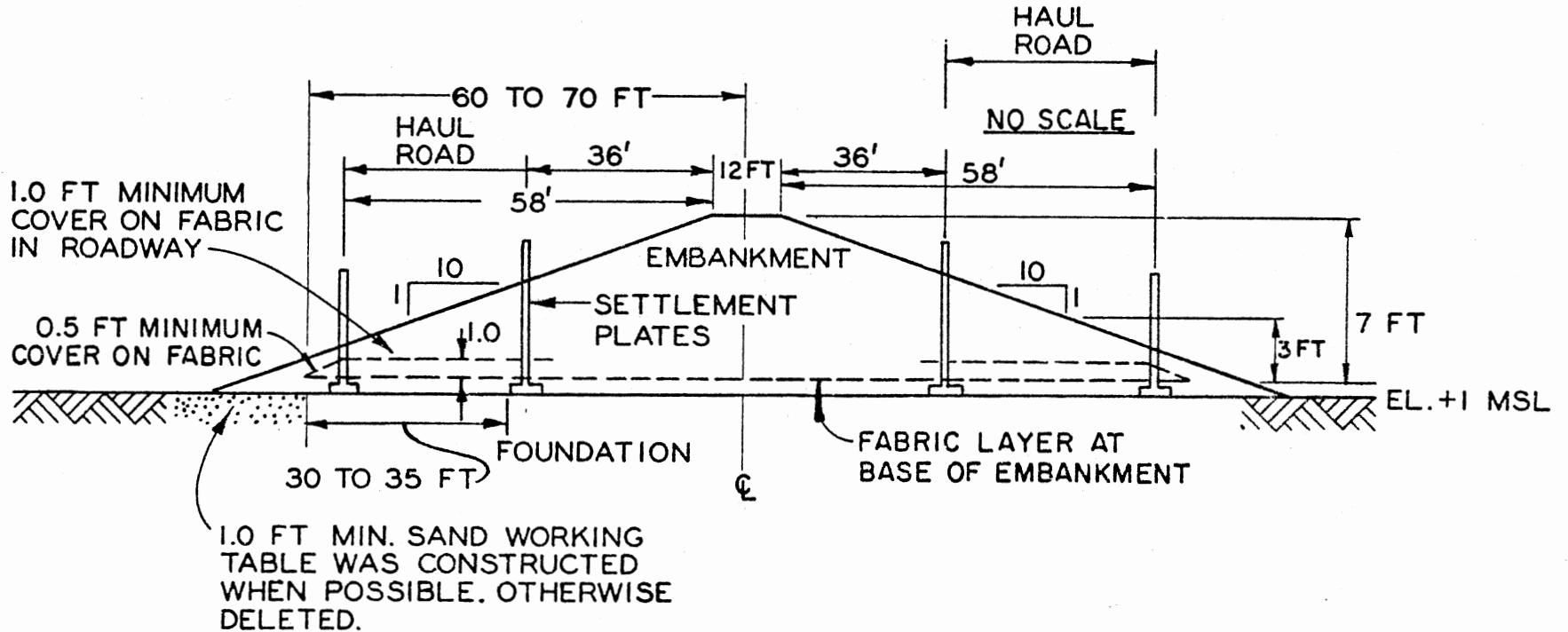
Figure 19. Construction Details of Actual Fabric-reinforced Embankment Section
