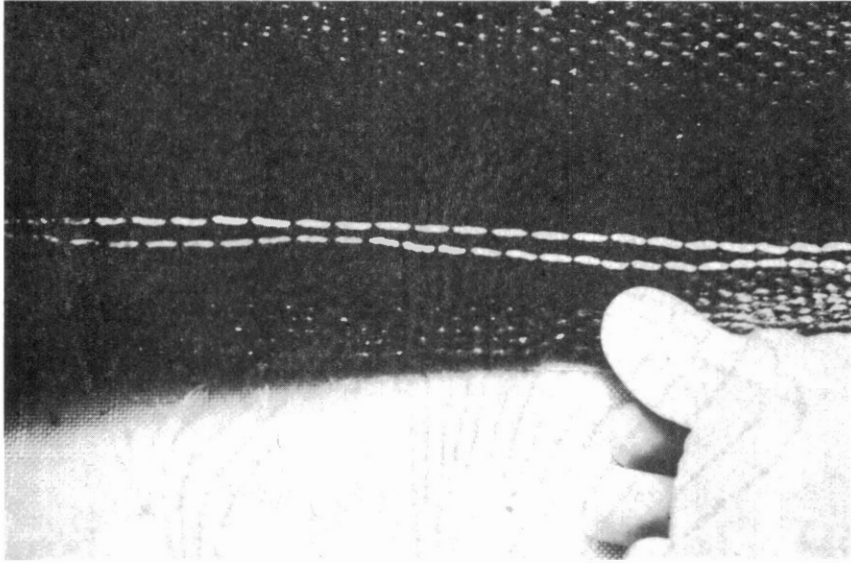
Figure 58. Top Side of Chain Stitch Joining Nicolon 66475 and Nicolon 66186 with 3 to 5 Stitches Per Inch
