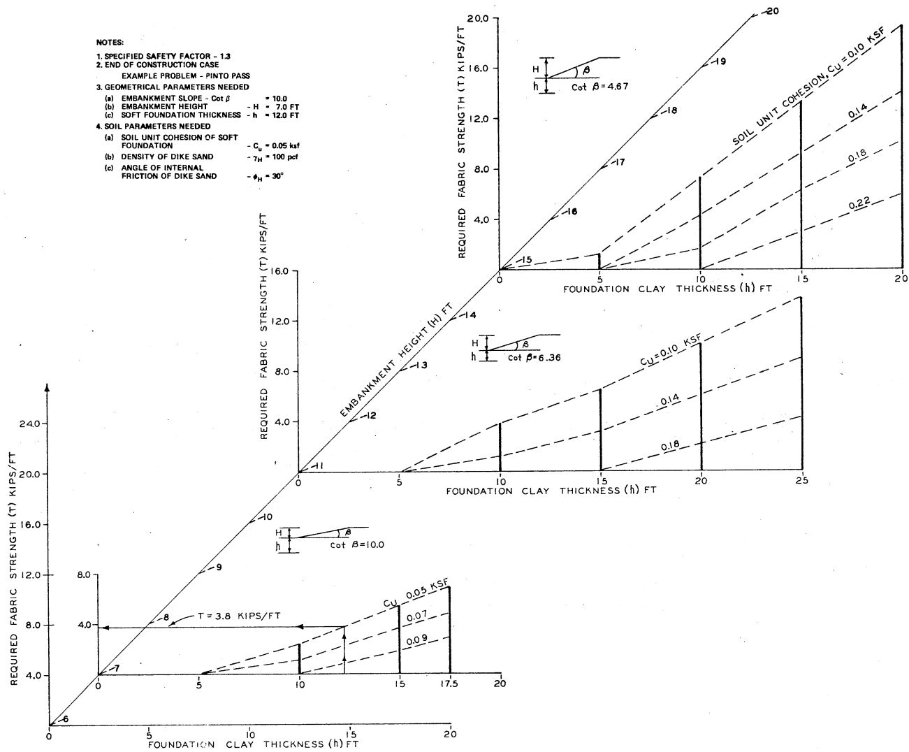
Figure 103. Design Curves to Determine Embankment Fabric Strength
