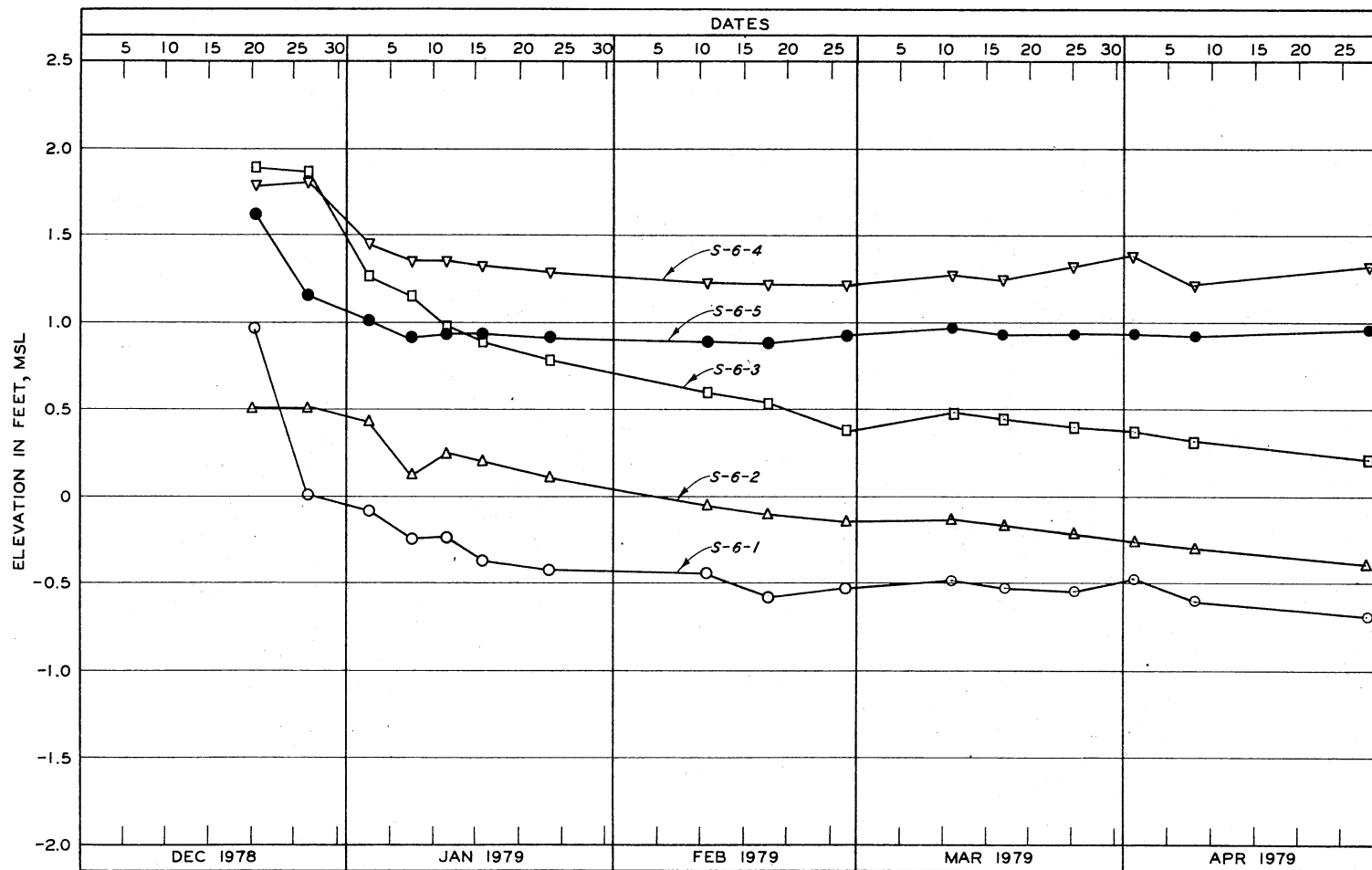
Figure 73. Settlement versus Time for Settlement Plates S-6-1 through S-6-5
