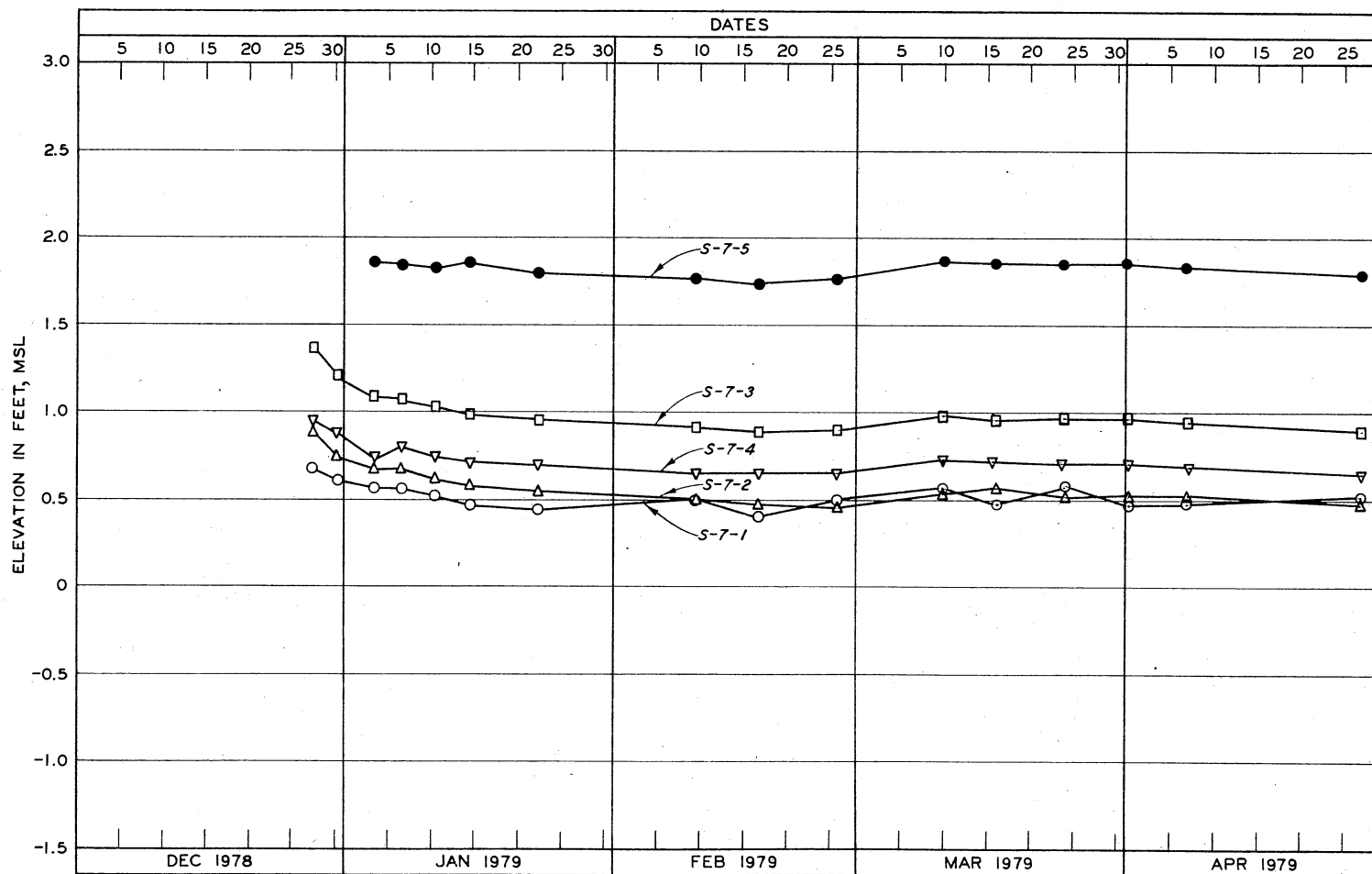
Figure 74. Settlement versus Time for Settlement Plates S-7-1 through S-7-5
