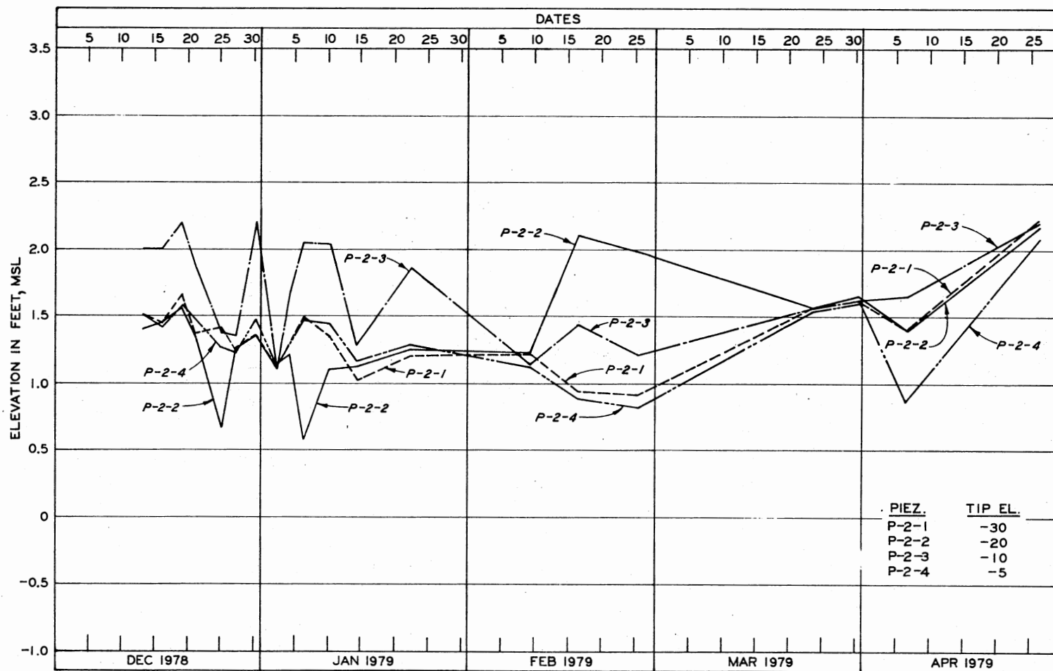
Figure 81. Pore Pressure versus Time for Piezometers P-2-1 through P-2-4
