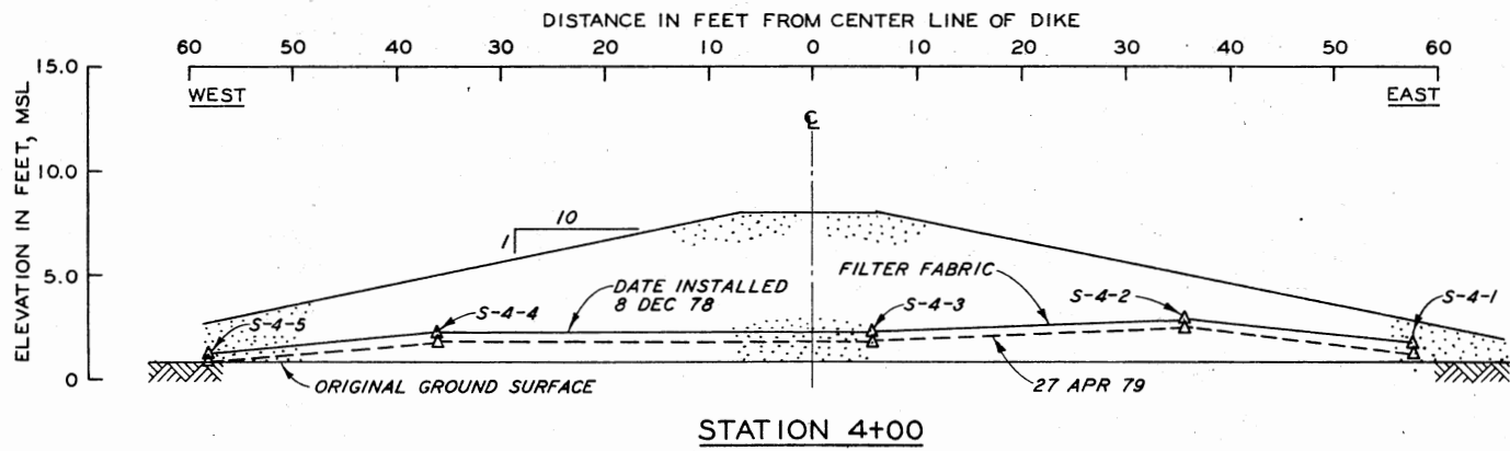
Figure 76. Settlement Profiles for Stations 3+00 and 4+00
