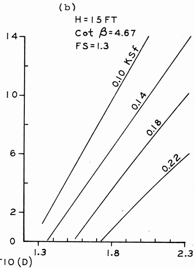
Figure 99. Design Curves for Dike Height = 15 ft
