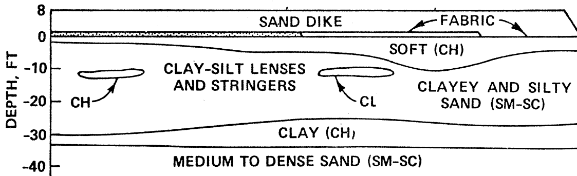
B. TYPICAL SOIL PROFILE PINTO PASS, ALABAMA
