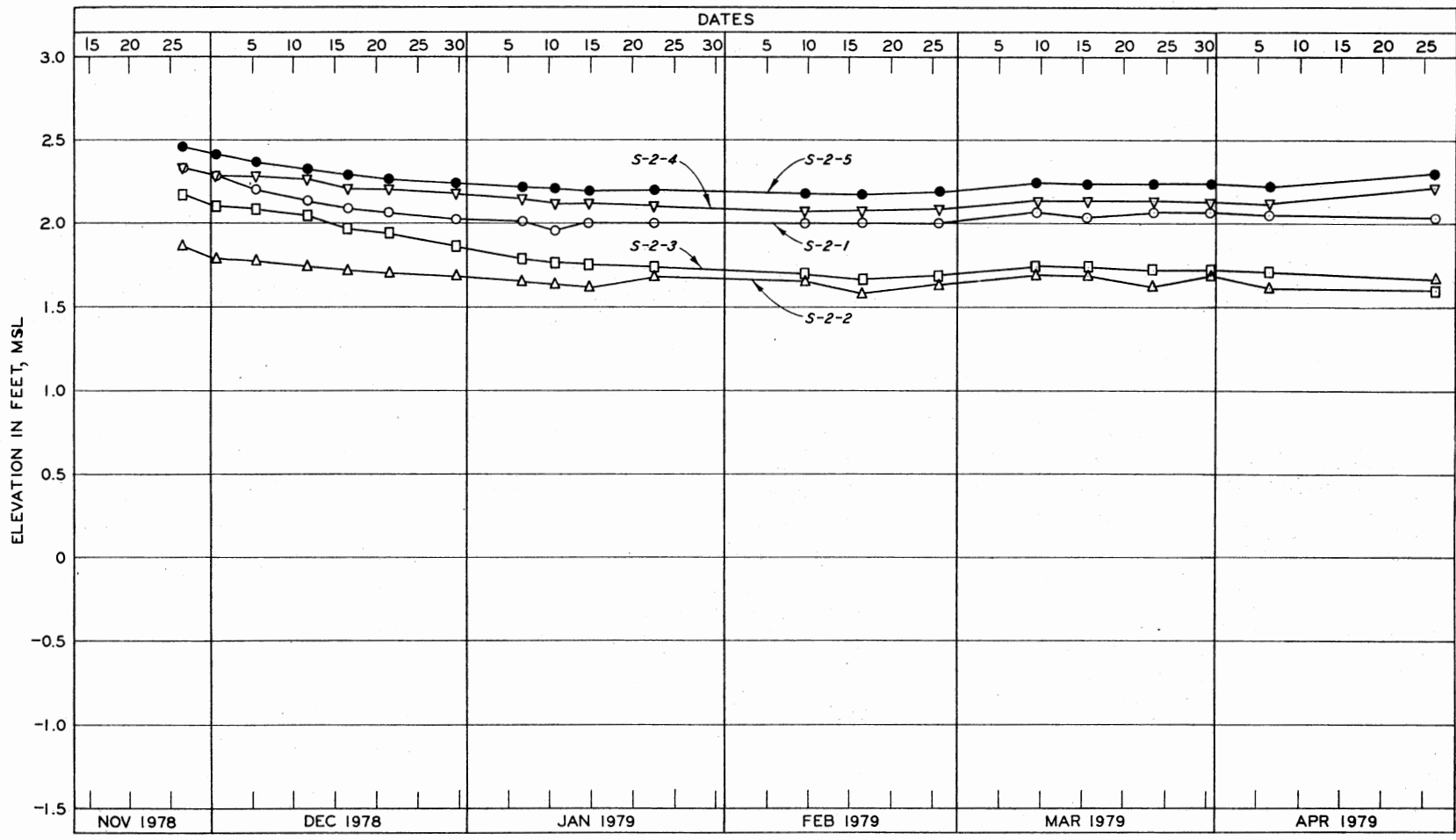
Figure 69. Settlement versus Time for Settlement Plates S-2-1 through S-2-5
