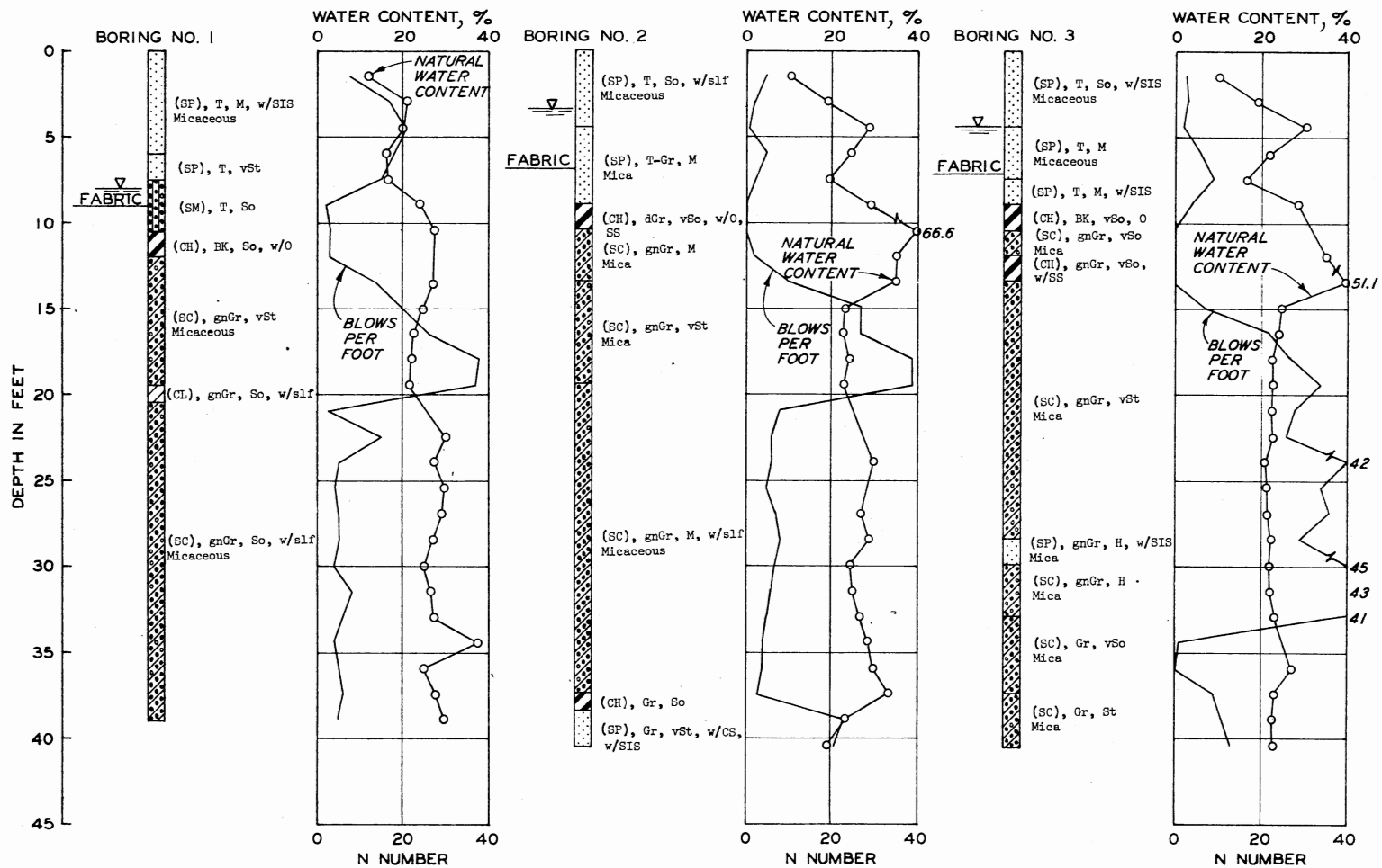
Figure 24. Boring Log and Water Content and N-Number versus Depth for Borings 1, 2, and 3
