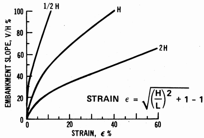
b. EMBANKMENT SLOPE VERSUS STRAIN
