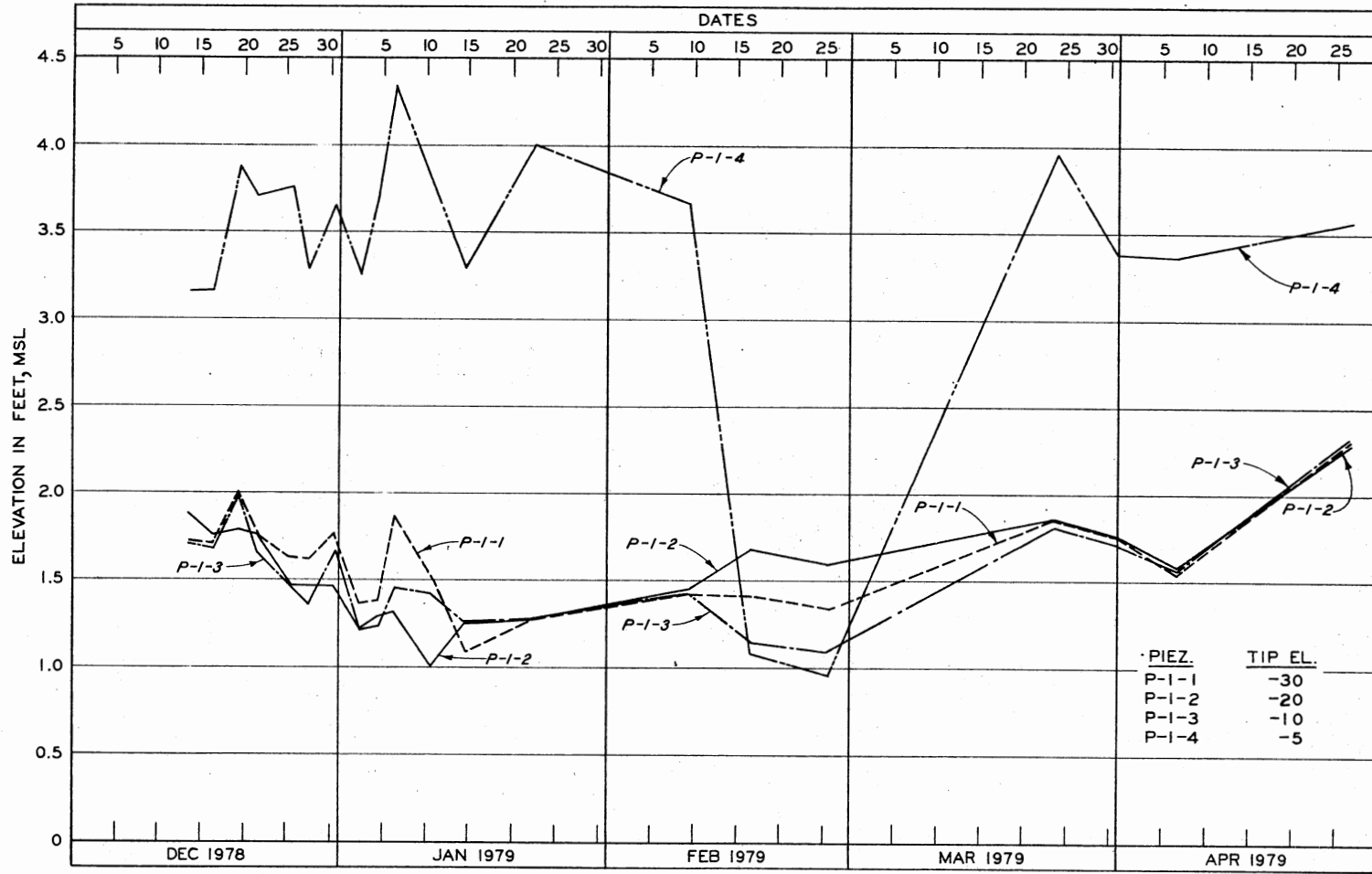
Figure 80. Pore Pressure versus Time for Piezometers P-1-1 through P-1-4
