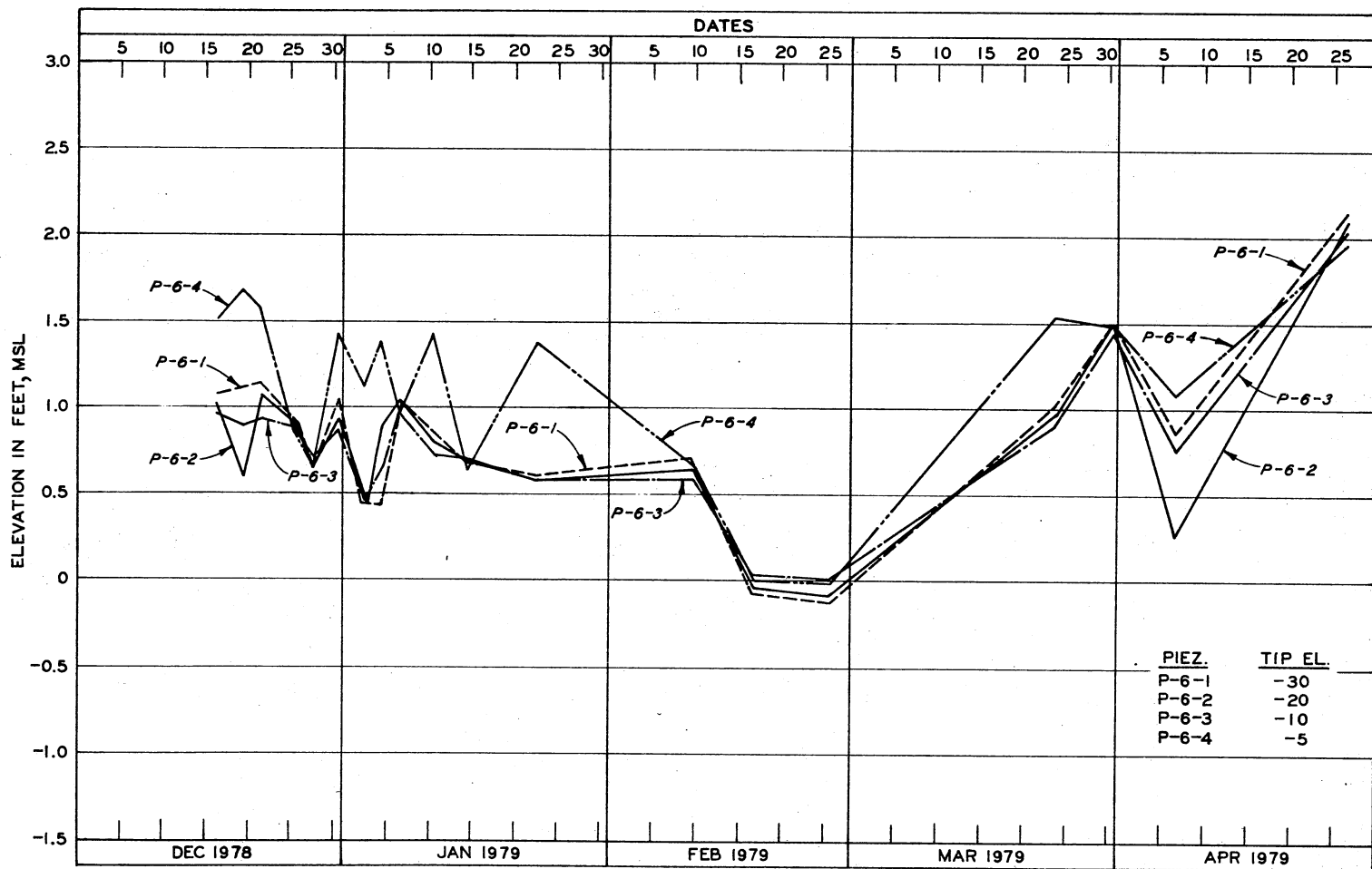
Figure 85. Pore Pressure versus Time for Piezometers P-6-1 through P-6-4
