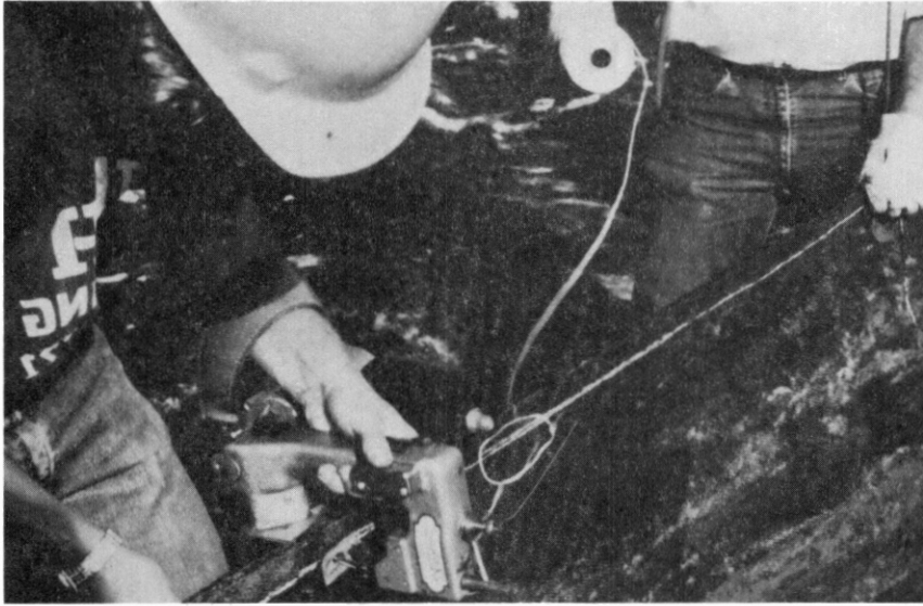
Figure 56. Closeup of Nicolon 66475 Fabric Being Sewn with a Sac-up Model BB Hand-held Field Sewing Machine
