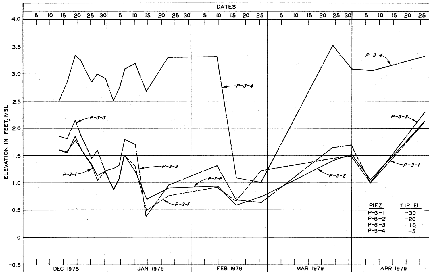
Figure 82. Pore Pressure versus Time for Piezometers P-3-1 through P-3-4
