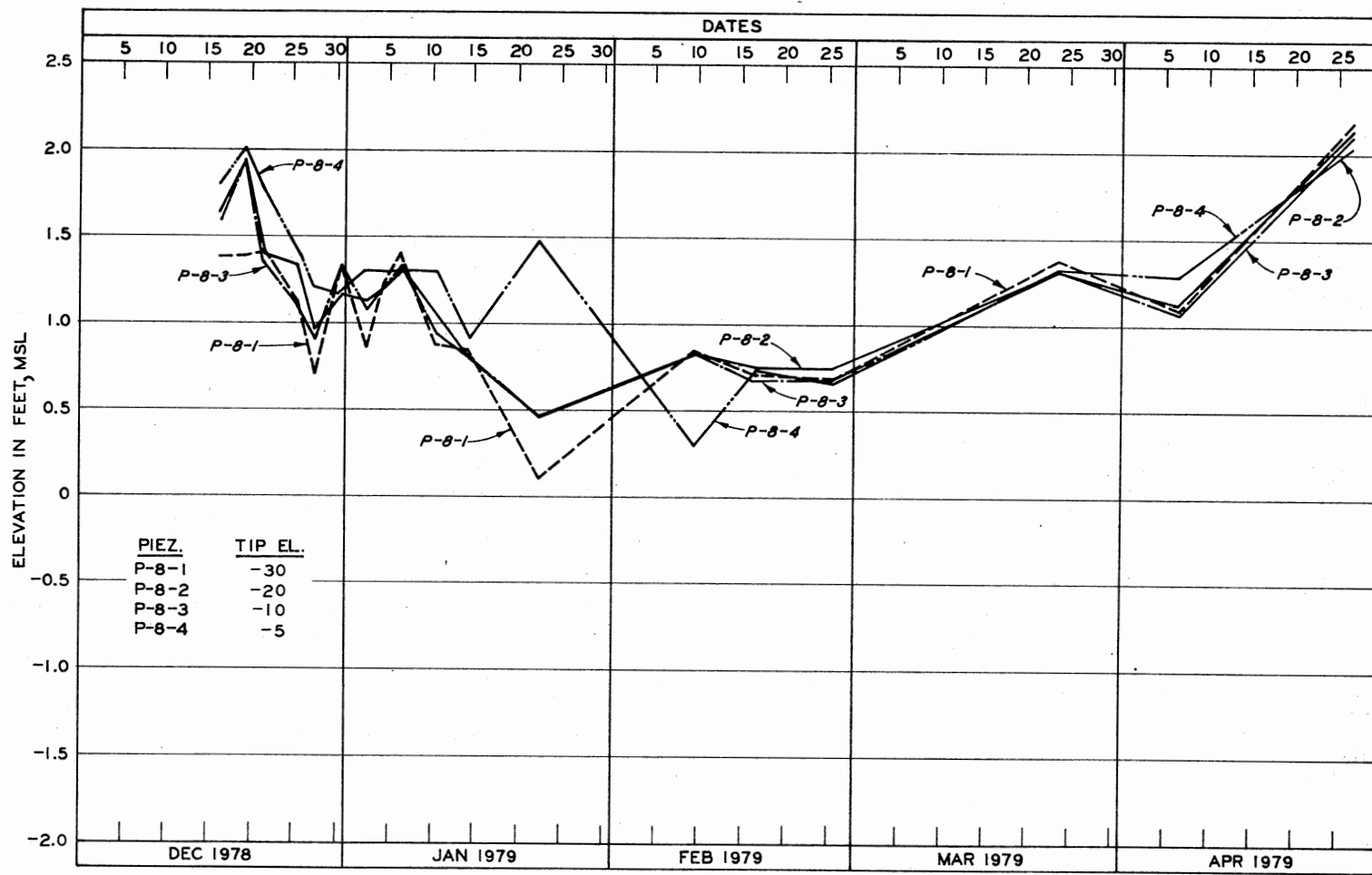
Figure 87. Pore Pressure versus Time for Piezometers P-8-1 through P-8-4
