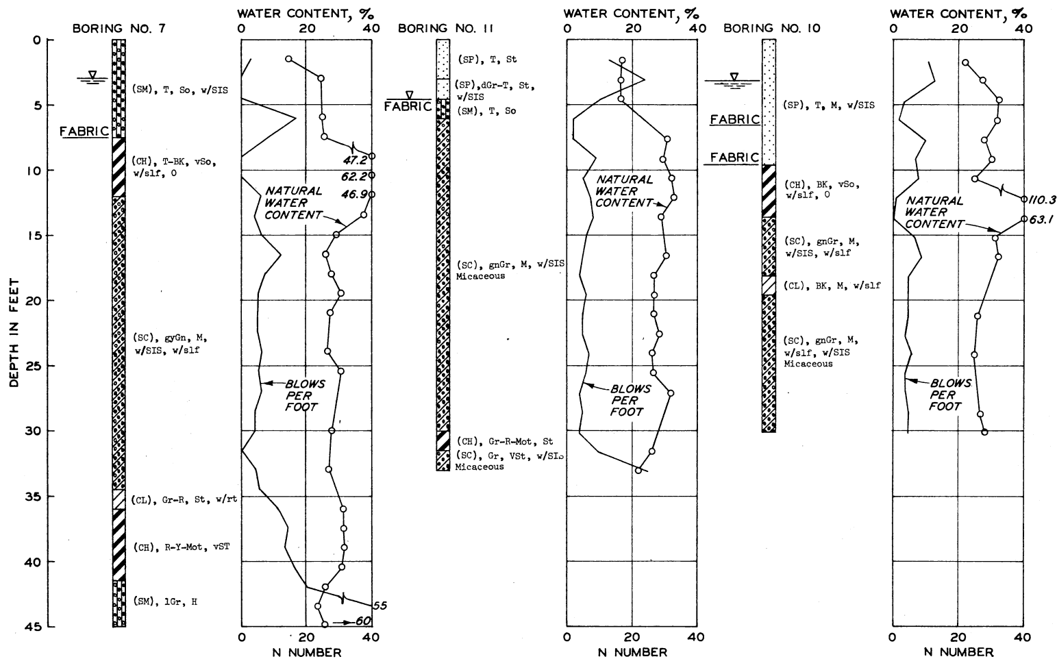
Figure 27. Boring Log and Water Content and N-Number versus Depth for Borings 7, 10, and 11
