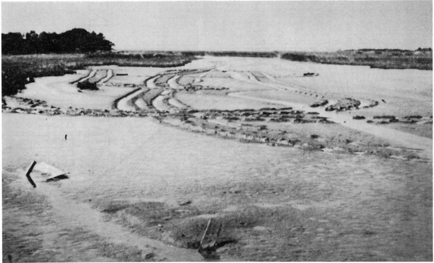
Figure 3. Ground Photograph of Pinto Pass Looking East to West with Mobile Harbor in the Background. Embankment Test Section to be Constructed West of the Narrow Channel Shown in the Photograph
