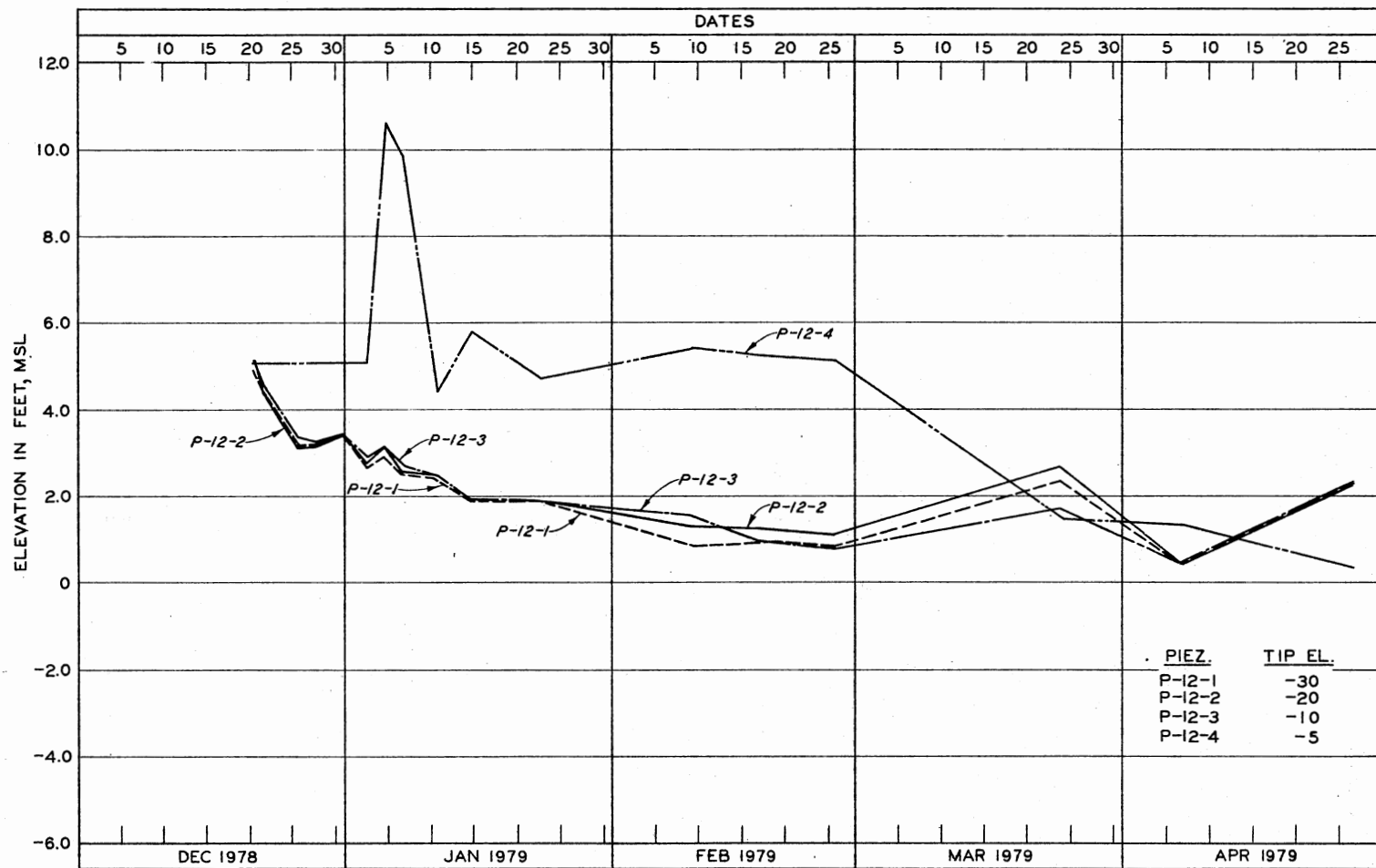
Figure 91. Pore Pressure versus Time for Piezometers P-12-1 through P-12-4
