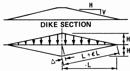
a. DIKE LOAD &amp; DISPLACEMENT
