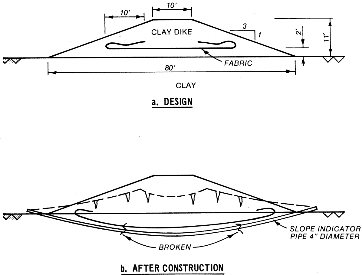
Figure 7. Embankment Section, Swan Lake, Mississippi
