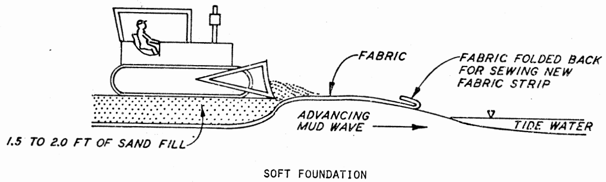
Figure 20. Laying Fabric on Mud Wave
