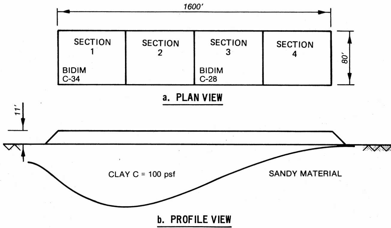
Figure 6. Plan and Profile View of Embankment Constructed at Swan Lake, Mississippi
