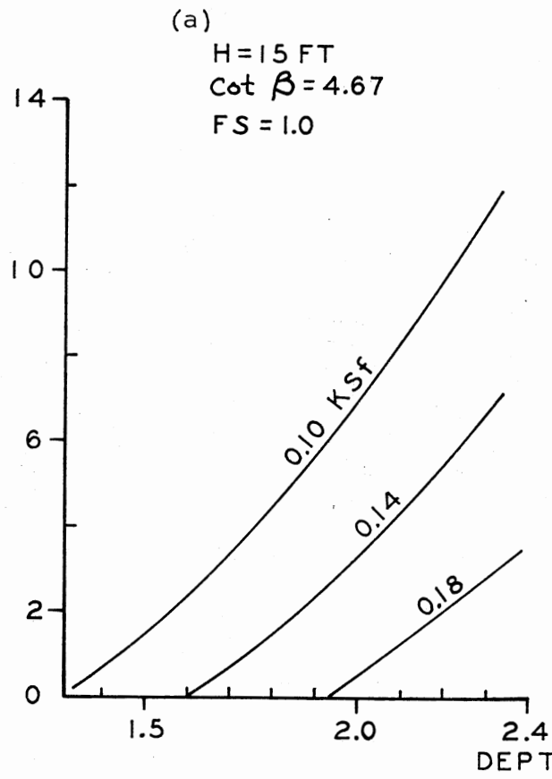
Figure 99. Design Curves for Dike Height = 15 ft
