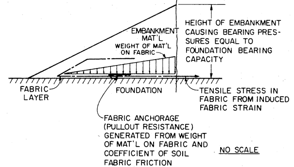
d. INSUFFICIENT FABRIC ANCHORAGE DURING EMBANKMENT DEFORMATION
