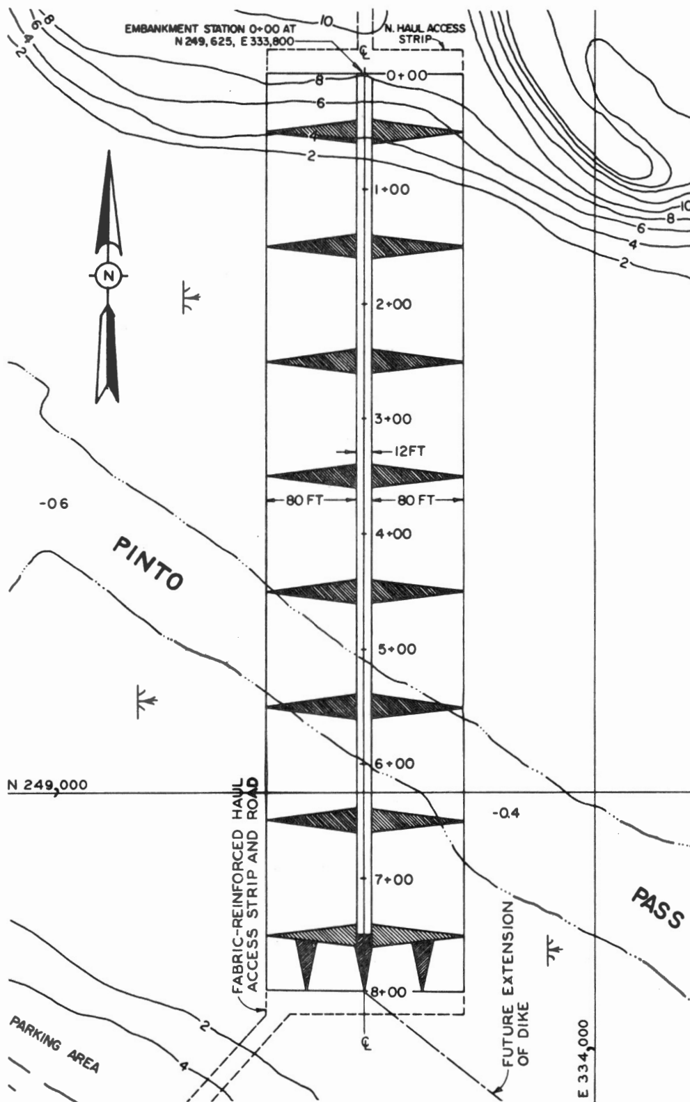
Figure 10, Detailed Plan View of Embankment Test Section
