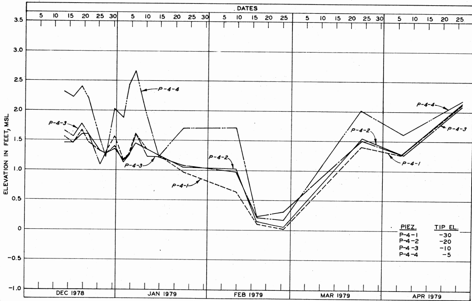
Figure 83. Pore Pressure versus Time for Piezometers P-4-1 through P-4-4
