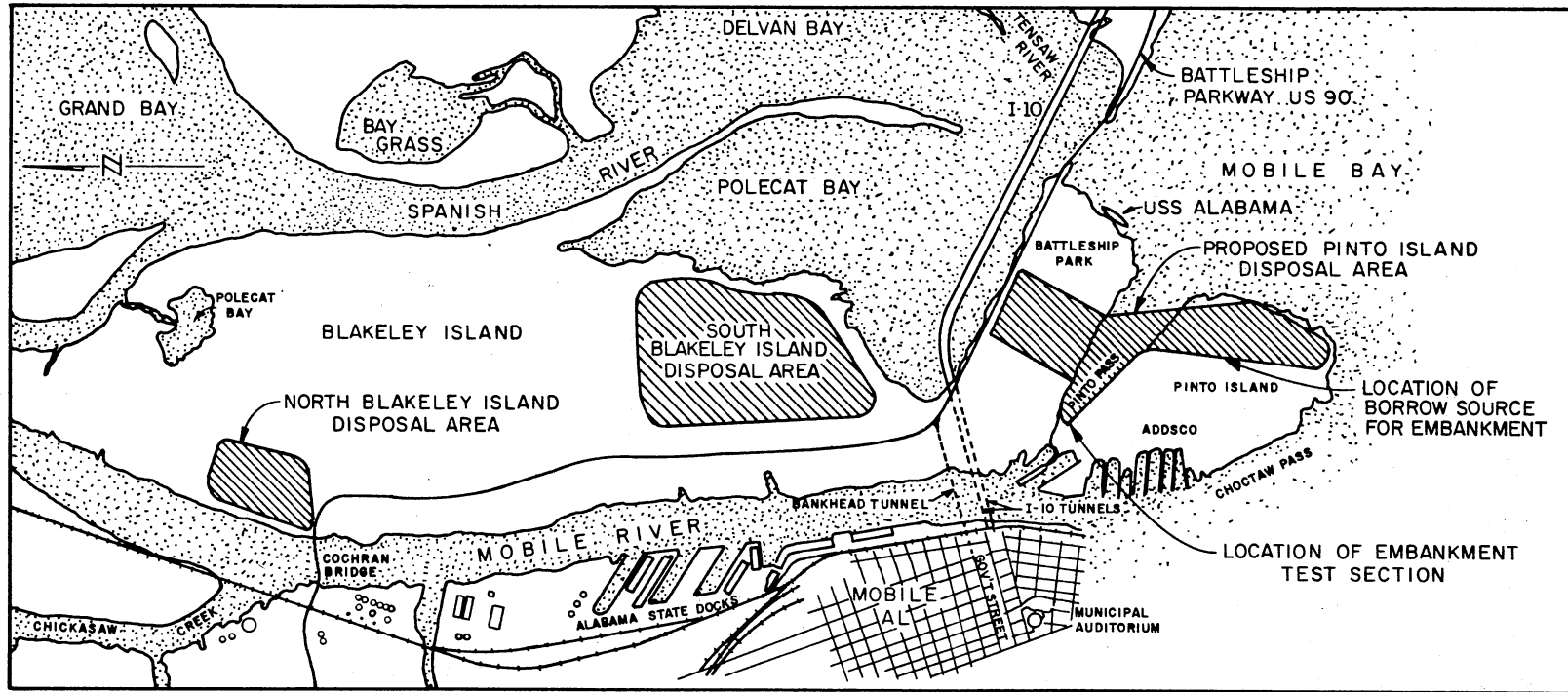
Figure 1. General Location of Embankment Test Section in Mobile Harbor, Alabama
