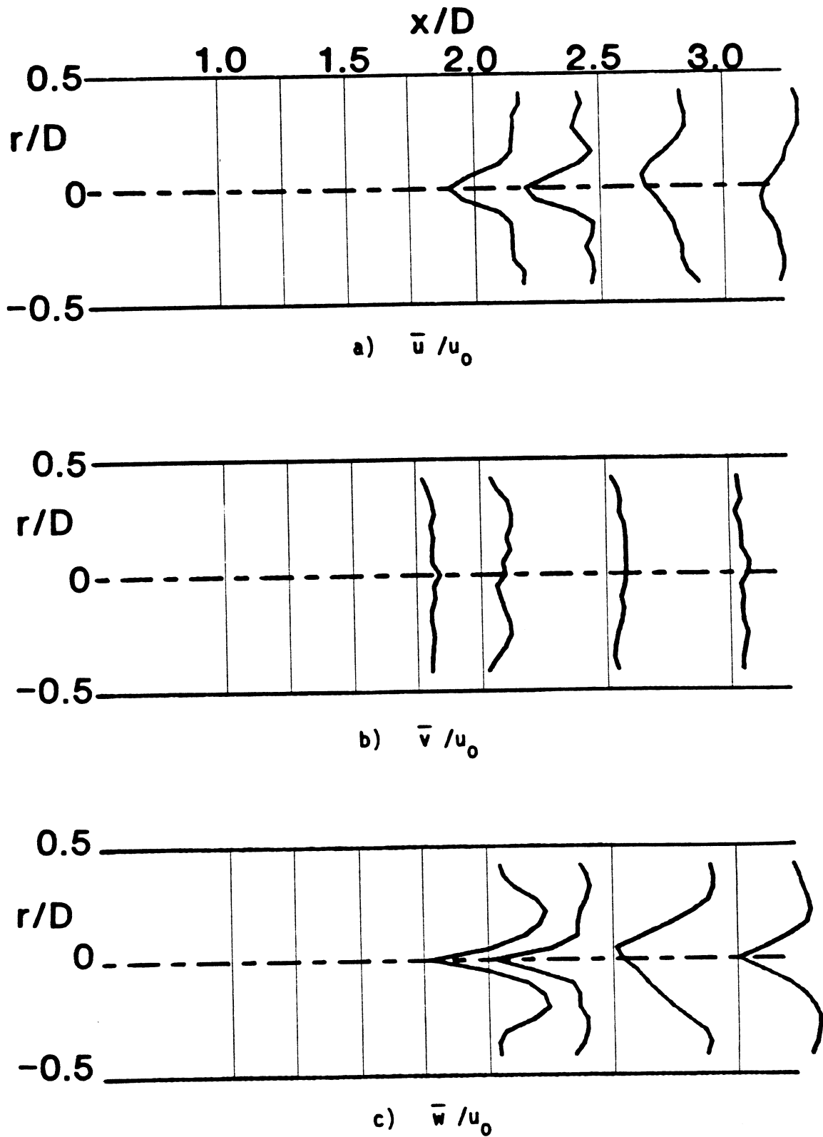
Figure 18. Time-Mean and Turbulent Flowfield, R = 4 , \phi = 45 Degrees, Traverse Angle \theta = 30 Degrees.
