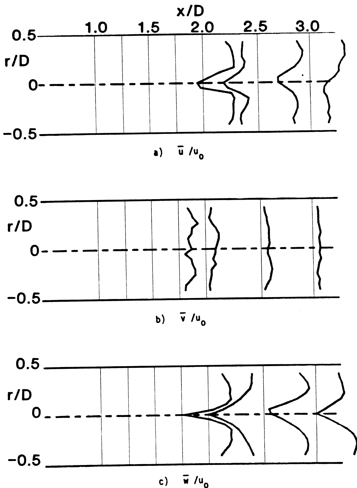
Figure 19. Time-Mean and Turbulent Flowfield, R = 4 , \phi = 45 Degrees, Traverse Angle \theta = 60 Degrees.
