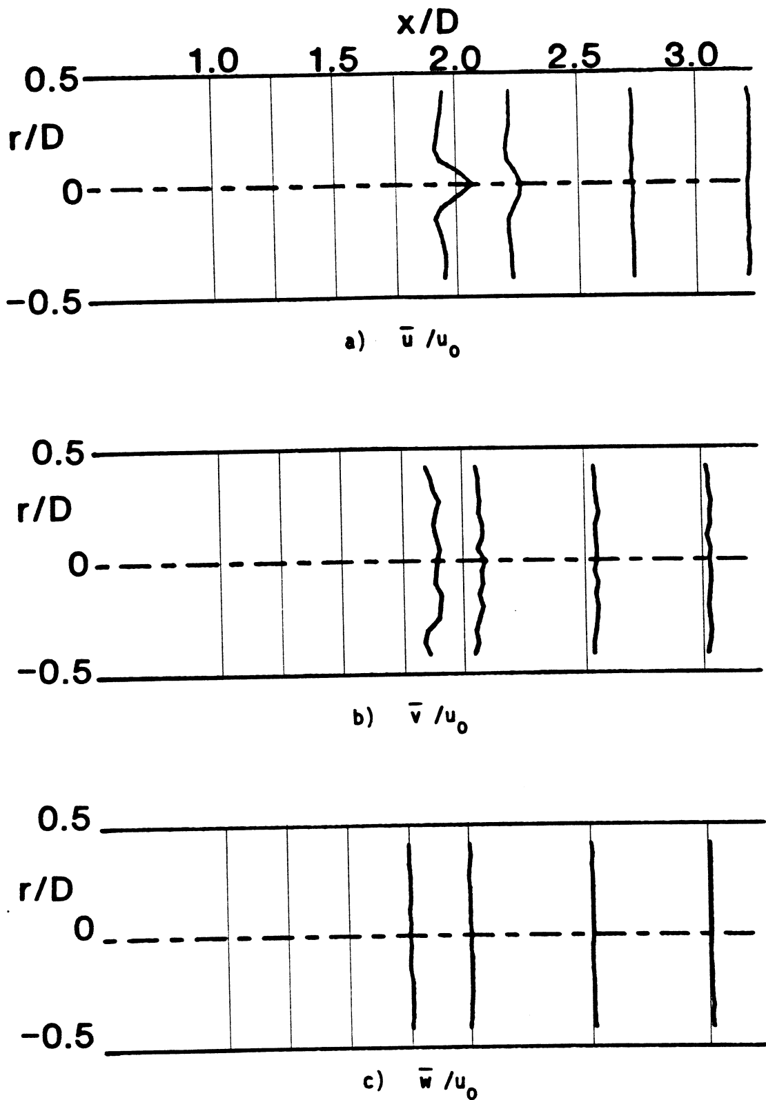
Figure 11. Time-Mean and Turbulent Flowfield, R = 4 , \phi = 0 Degrees (Swirler Removed), Traverse Angle \theta = 0 Degrees.
