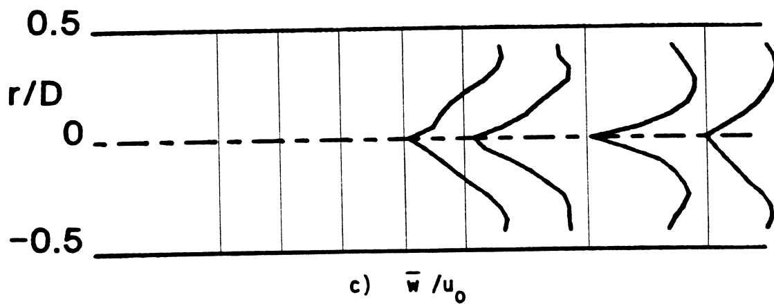
Figure 15. Time-Mean and Turbulent Flowfield, R = 4 , \phi = 45 Degrees, Traverse Angle \theta = 300 Degrees.
