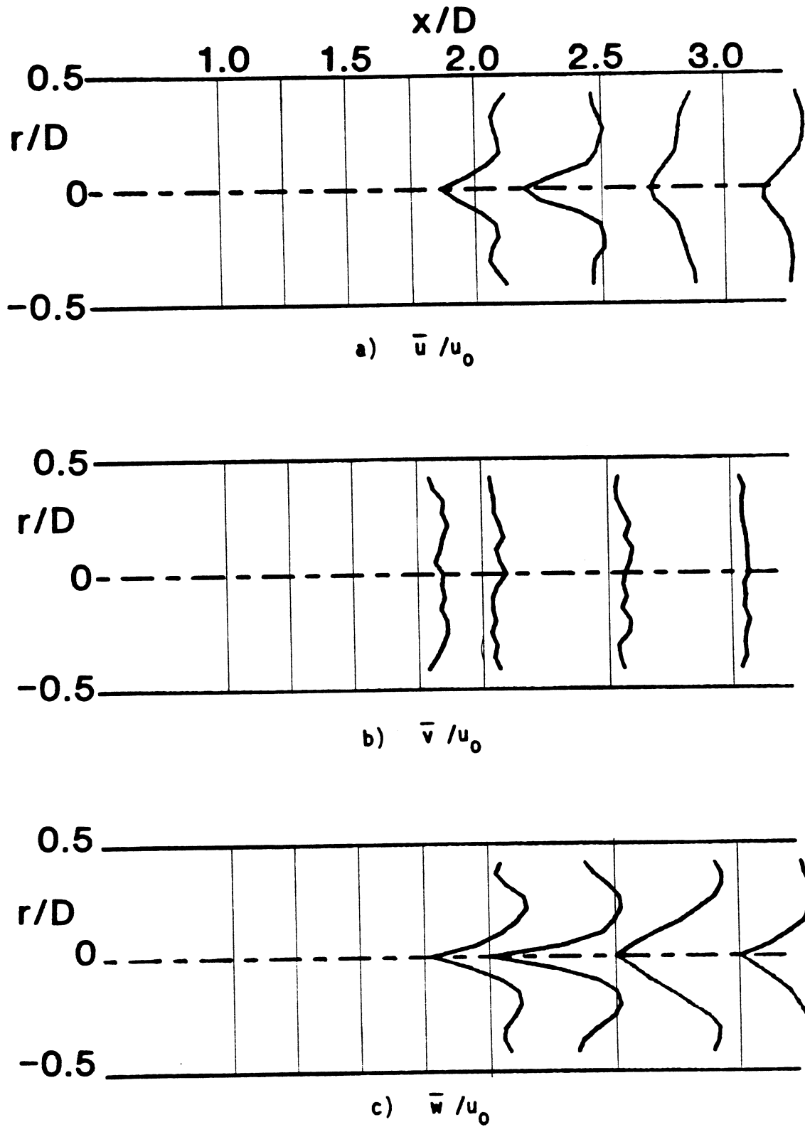
Figure 17. Time-Mean and Turbulent Flowfield, R = 4 , \phi = 45 Degrees, Traverse Angle \theta = 0 Degrees.
