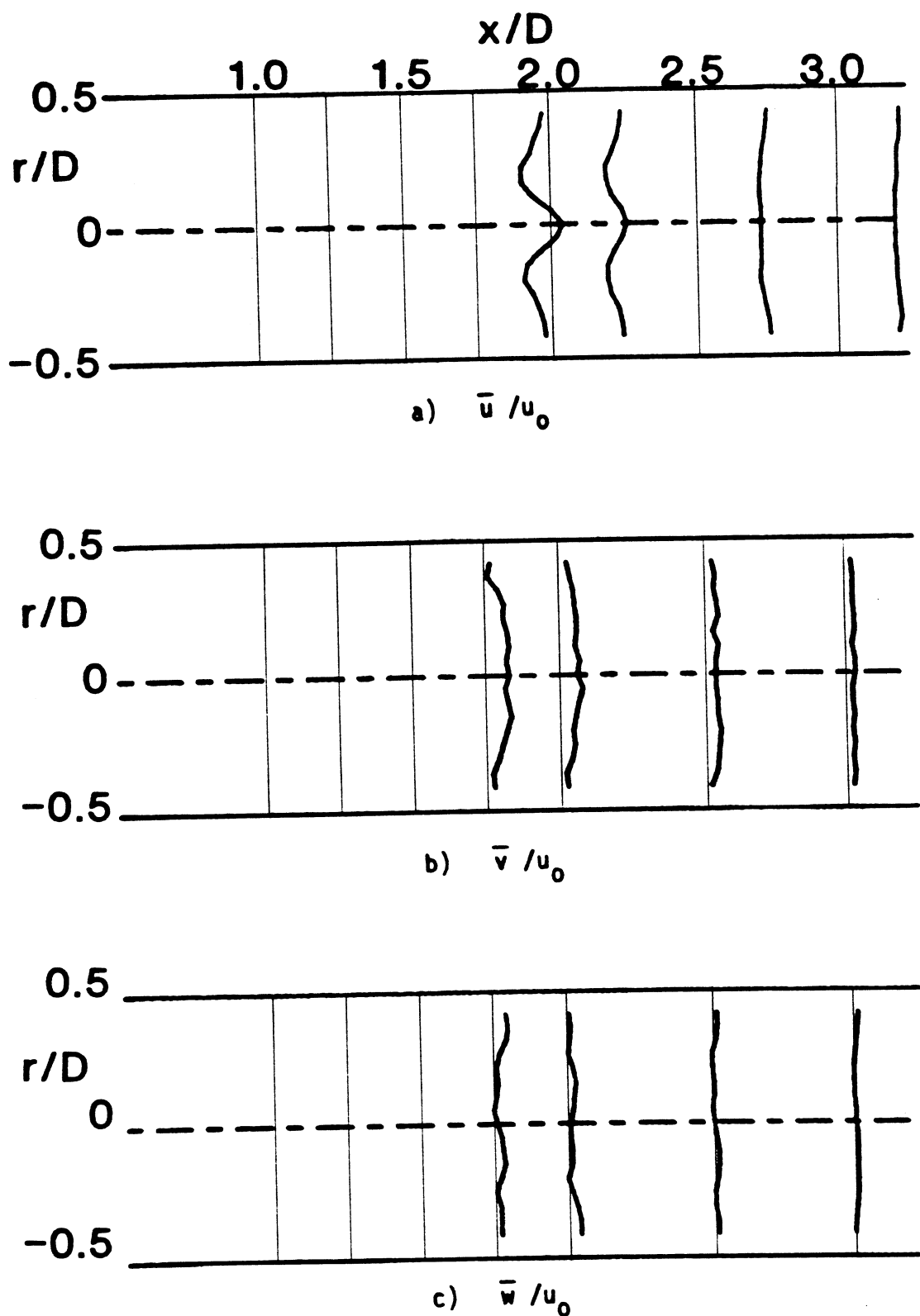
Figure 12. Time-Mean and Turbulent Flowfield, R = 4 , \phi = 0 Degrees (Swirler Removed), Traverse Angle \theta = 30 Degrees.
