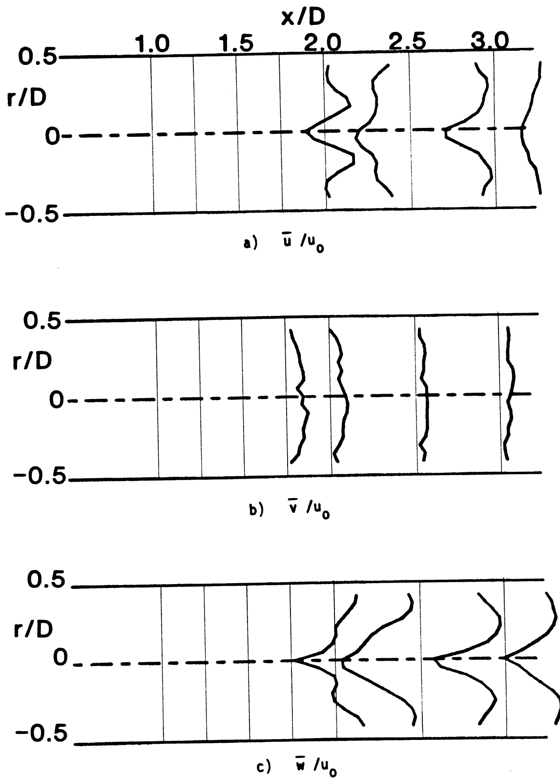
Figure 14. Time-Mean and Turbulent Flowfield, R = 4 , \phi = 45 Degrees, Traverse Angle \theta = 270 Degrees.
