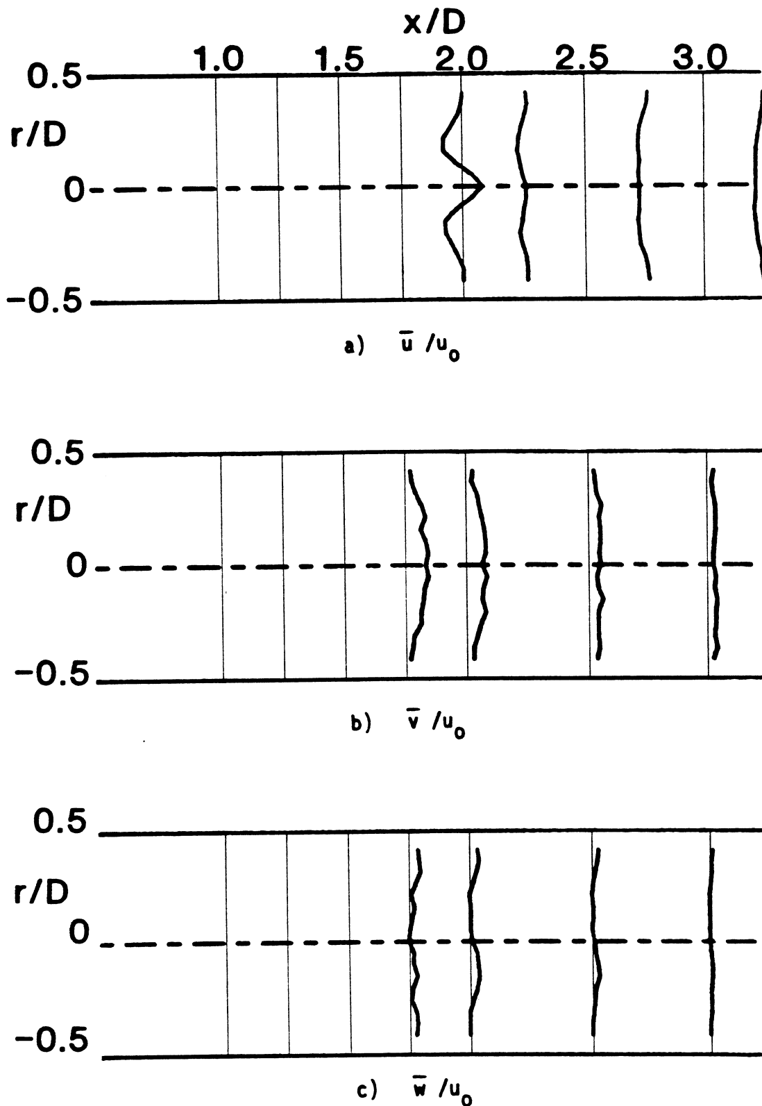
Figure 13. Time-Mean and Turbulent Flowfield, R = 4 , \phi = 0 Degrees (Swirler Removed), Traverse Angle \theta = 60 Degrees.
