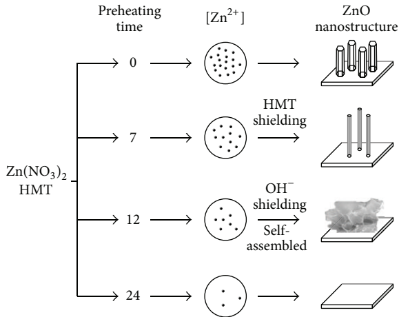
FIGURE 7: Schematic growth diagram of the ZnO nanostructures fabricated by preheating hydrothermal method.
