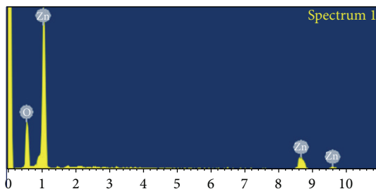
FIGURE 4: The EDS spectrum corresponds to the flower-like ZnO nanostructures.
