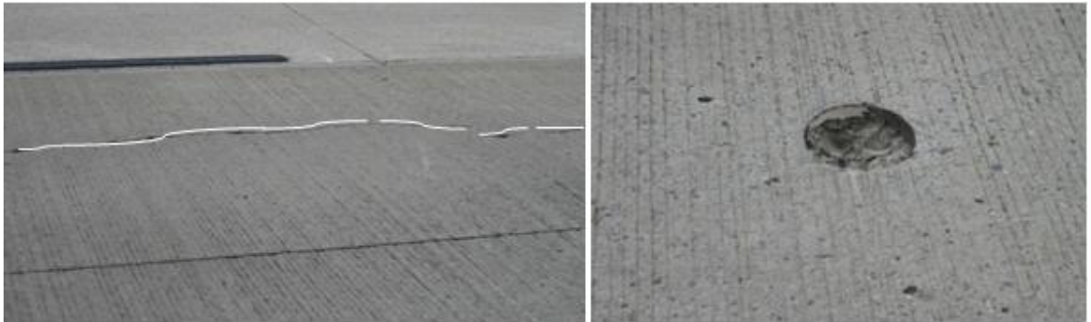
Figure 2.7 - Longitudinal Cracking spanning over panels Figure 2.8 -Testing core not refilled well.
