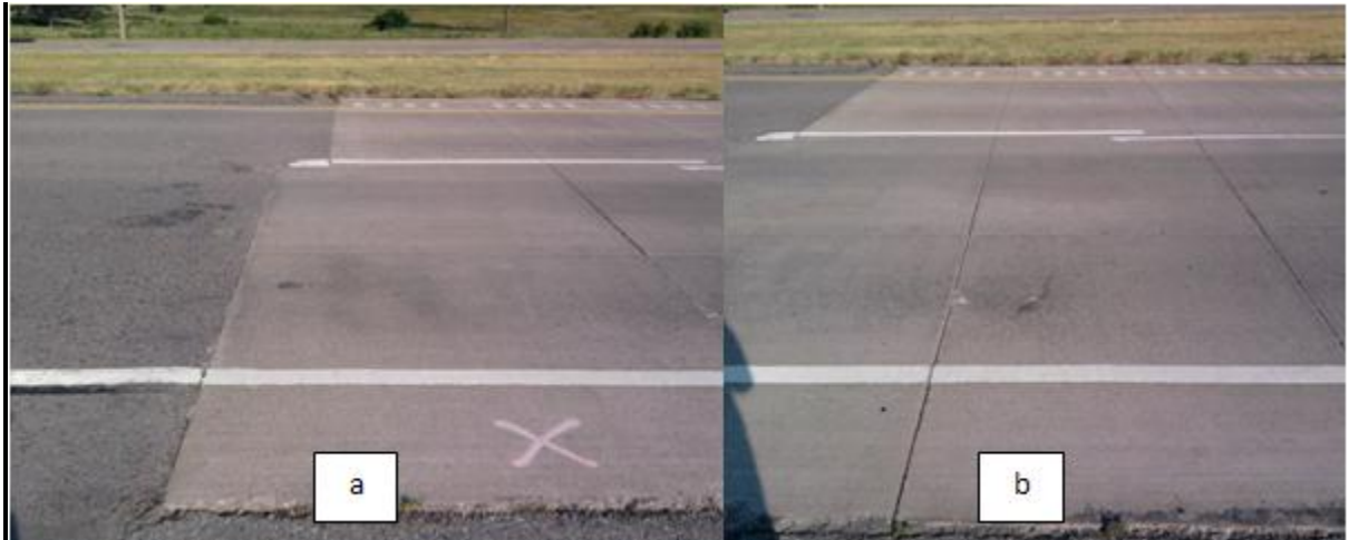
Figure 2.22 - Photo a showing start of the overlay where the asphalt pavement ends. A corner crack was seen on the second panel right after the start of the overlay as shown in photo b.
