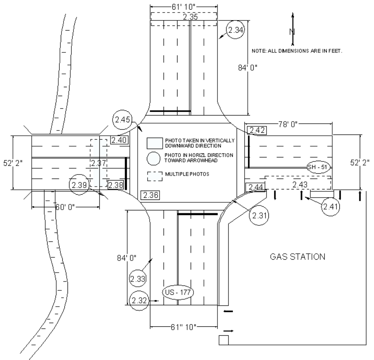
Figure 2.30 - Layout of the intersection of US – 177 and SH – 51 depicting the location where the photographs were taken.
