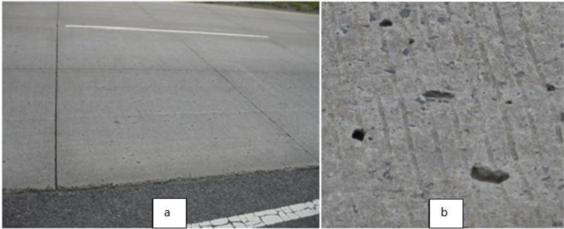
Figure 2.14 - Photo a showing pop outs (about 20 pop outs/panel) of larger aggregates (on about 24 panels) at about 0.5 miles from the south end of the overlay. Photo b is just the closer view of photo a.
