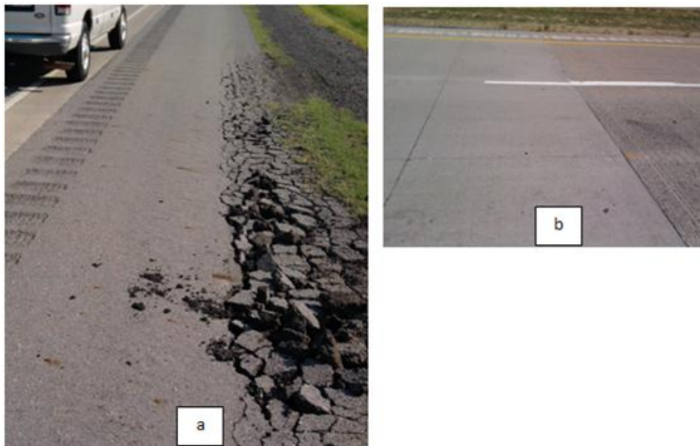
Figure 2.23 – Photo a shows the deterioration of the asphalt shoulders. Photo b shows the interface of the overlay with a CRCP. The end of the overlay was in excellent condition.
