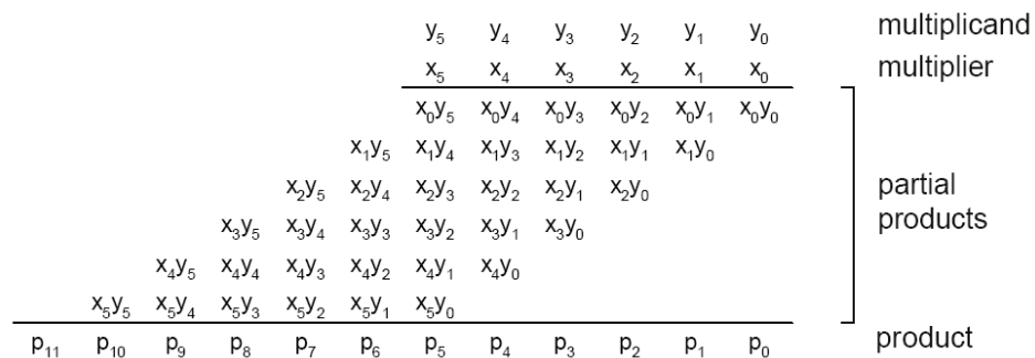
Figure 10. Partial products during multiplication, taken from [32].
