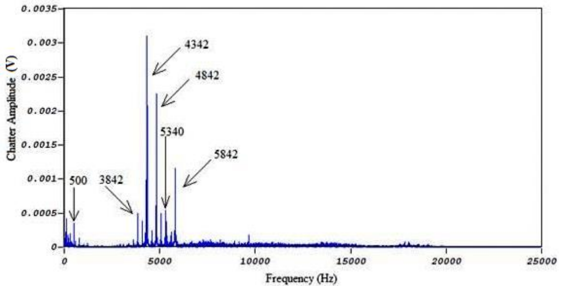
Figure 3.8 Frequency domain signal for milling without vibration assistance
