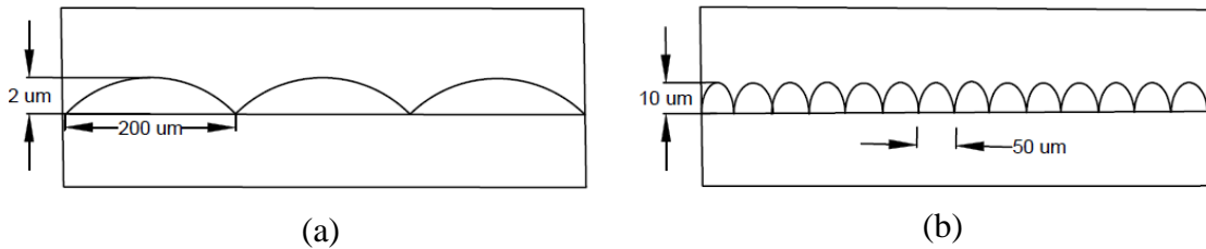
Figure 4.1 Tool tip trajectory using time domain simulation for (a) conventional (b) vibration assisted milling
