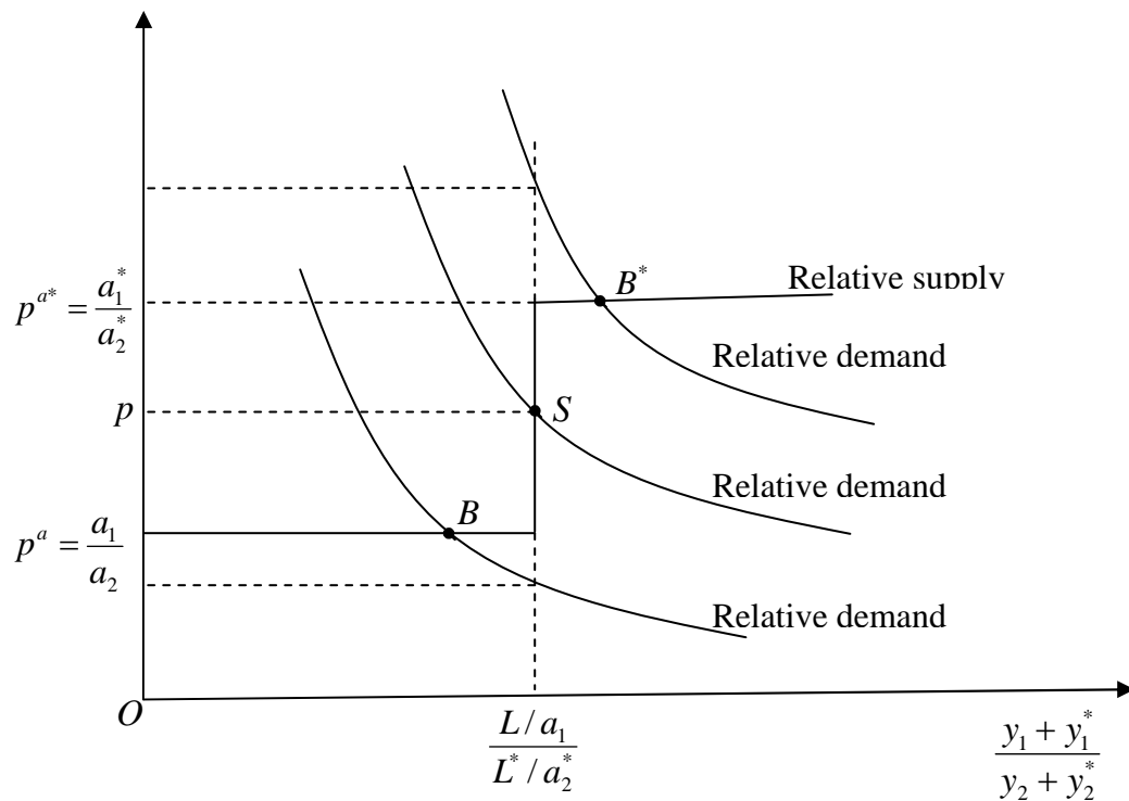
Figure 2-1: Regime Switch
