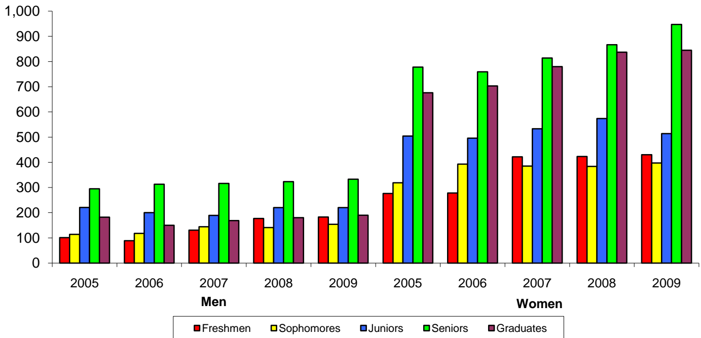
Men/Women Comparison
